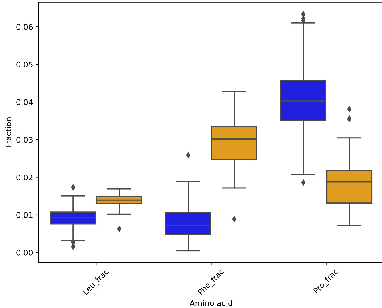
Light-strand genes
