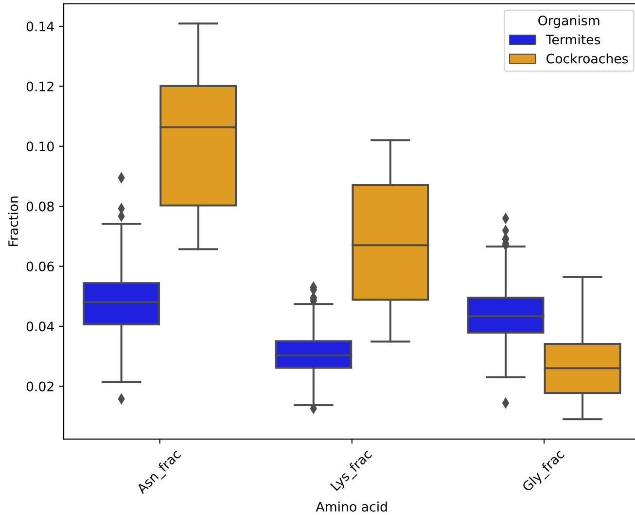
Heavy-strand genes
