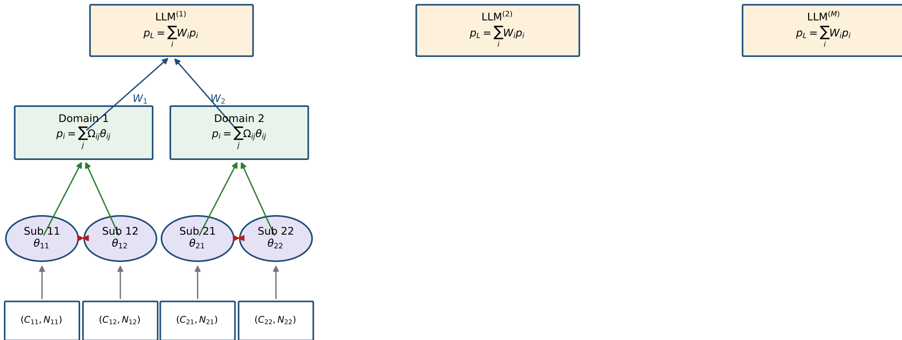
Fig. 1 (redrawn): hierarchy across LLM instances, domains, subdomains and tasks rectangle = independent component, oval = dependent component
