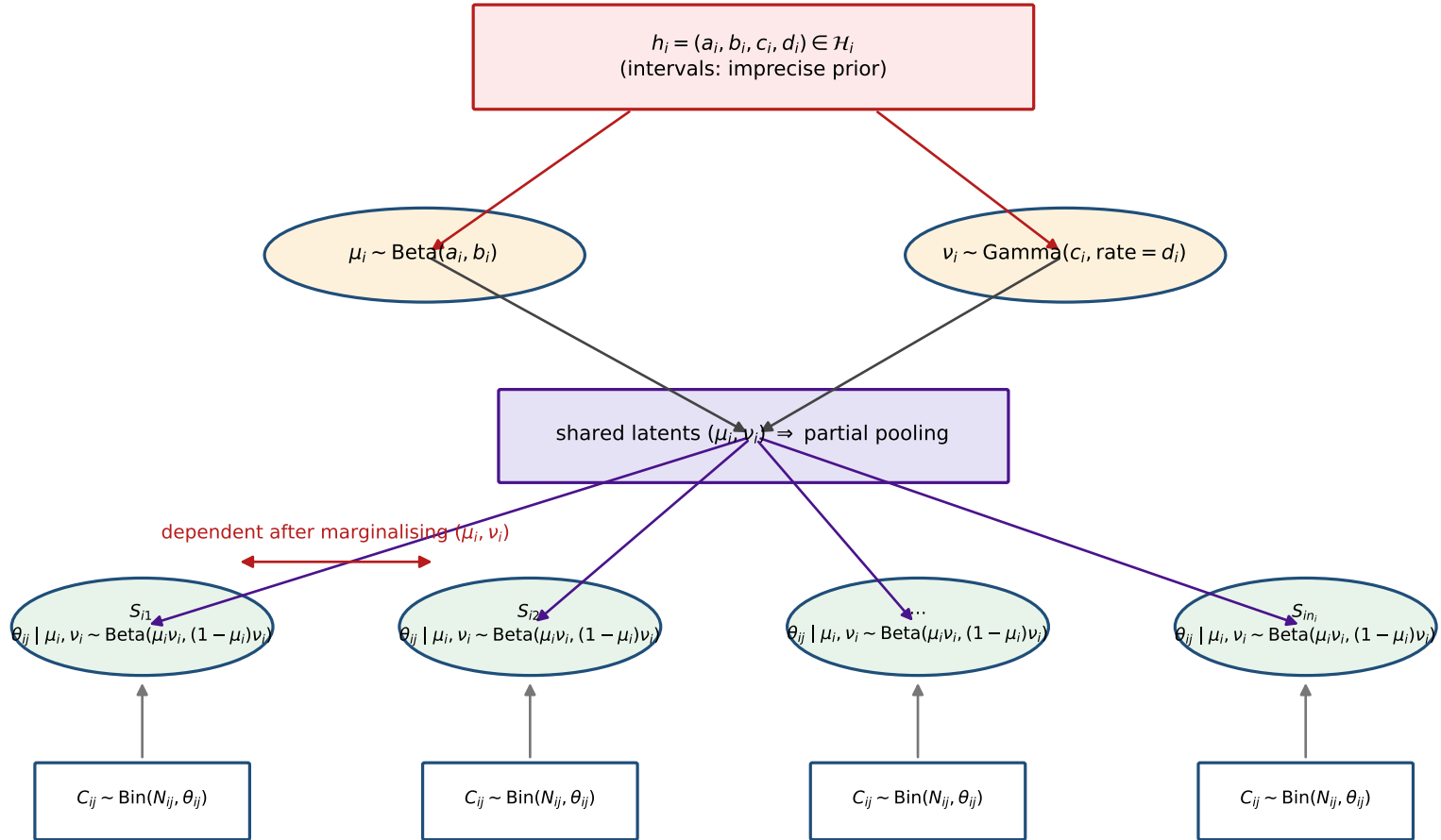
Fig. 2 (redrawn): detailed hierarchical probabilistic structure imprecise hyper-hyper-parameters -> hyperpriors -> shared latents -> subdomain reliabilities -> data
