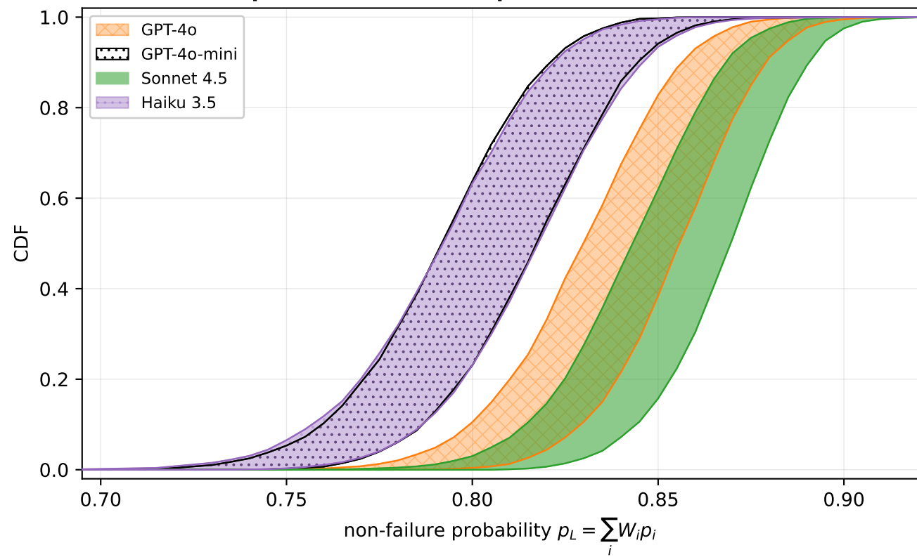
LLM posterior CDF envelopes (Overall Performance)
