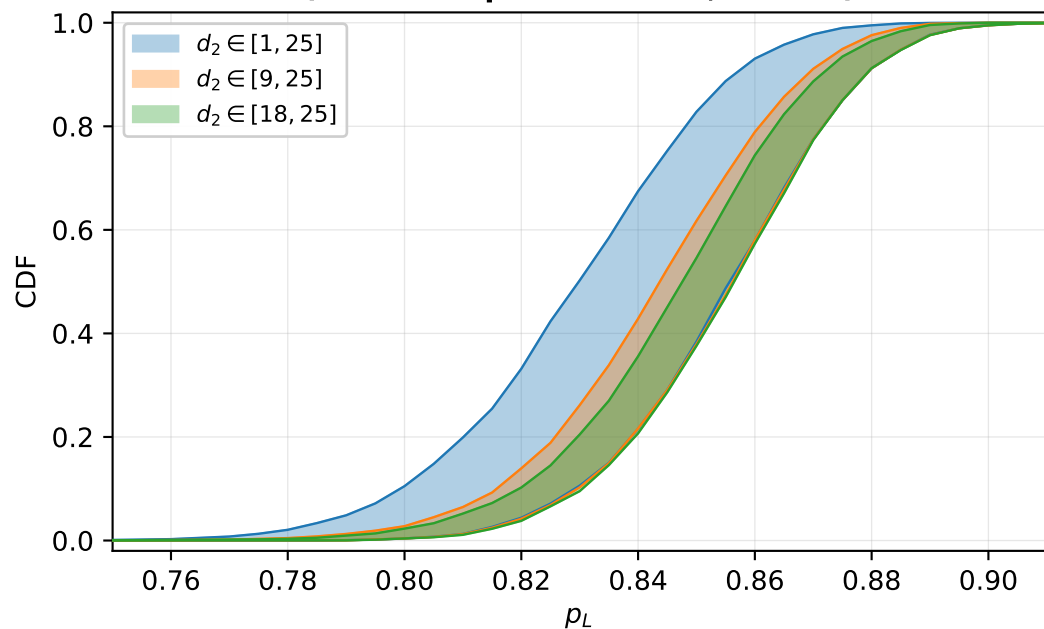
Narrowing the d_2 prior range (LLM-level posterior CDF, GPT-4o)
