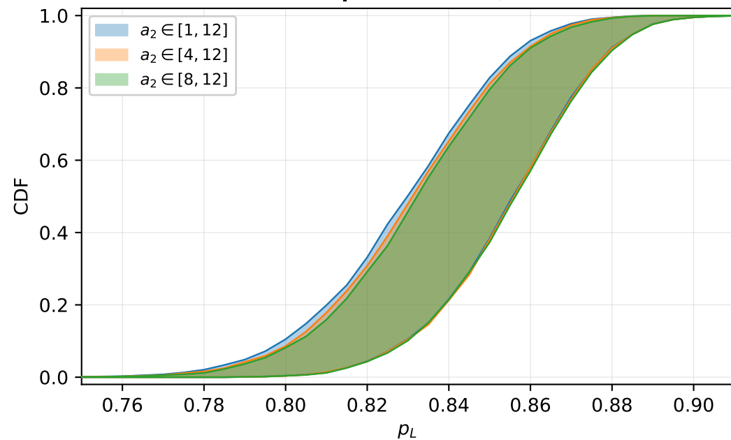
Narrowing the a_2 prior range (LLM-level posterior CDF, GPT-4o)
