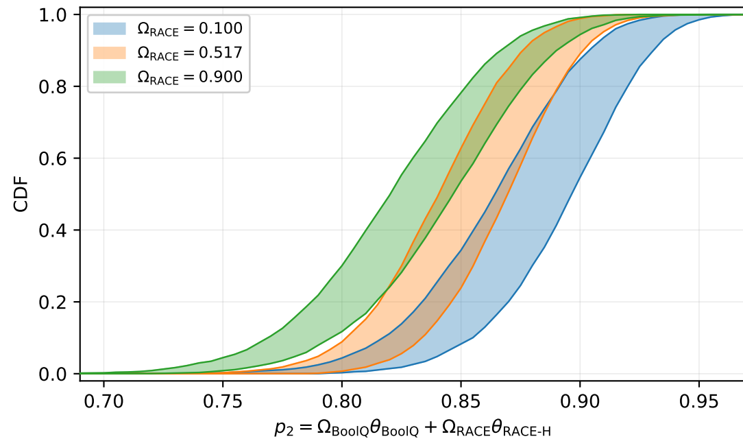
Reasoning domain D2 vs RACE-H weight (Sonnet 4.5)
