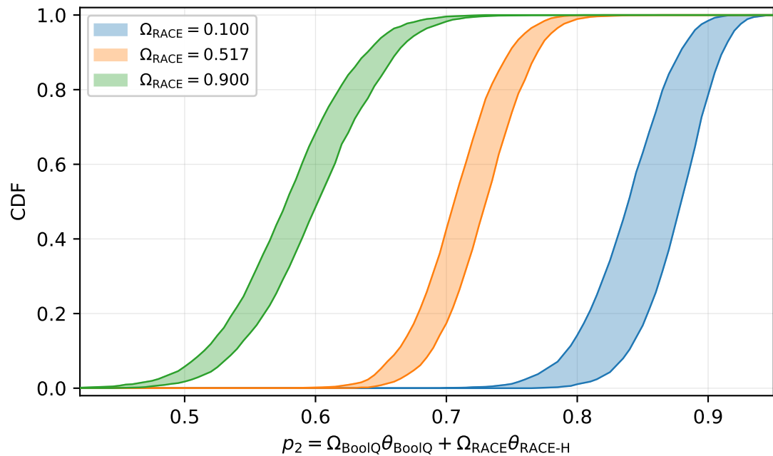
Reasoning domain D2 vs RACE-H weight (GPT-4o)
