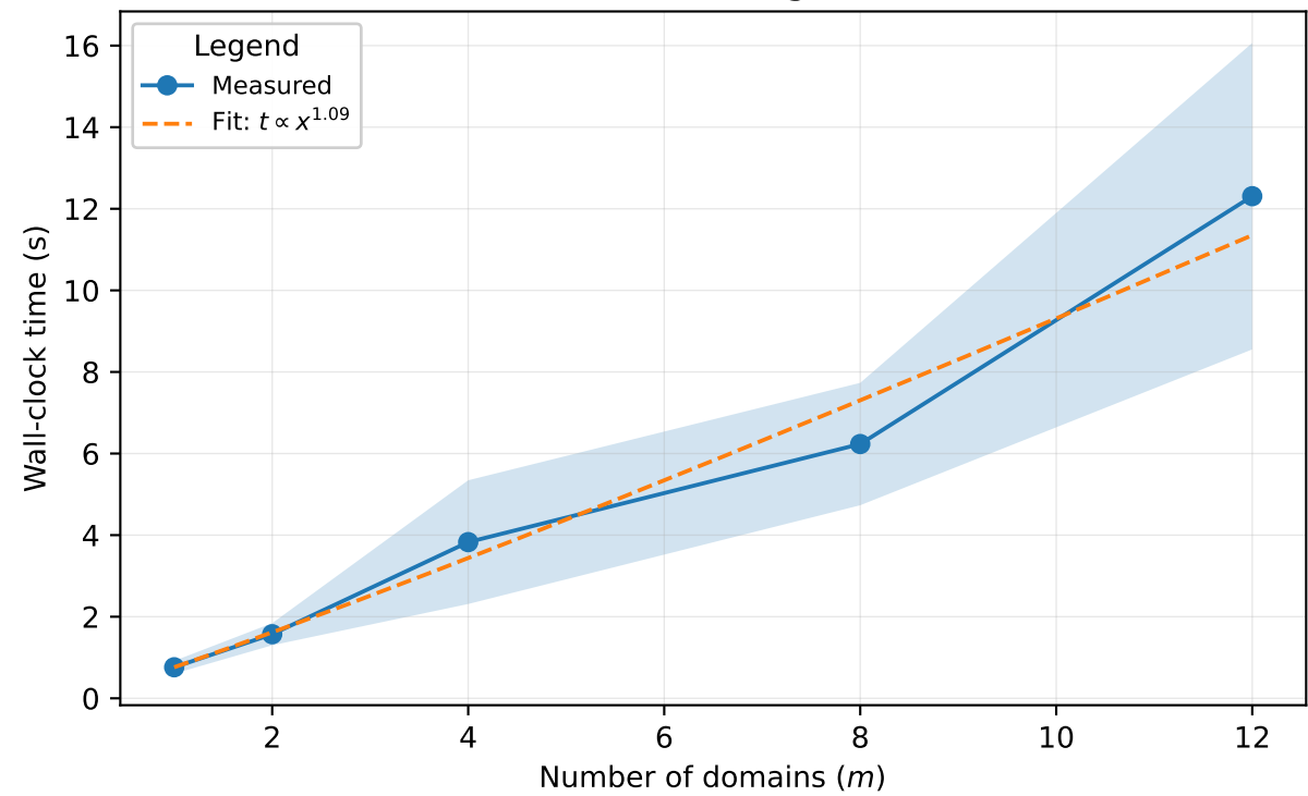
HIP-LLM scaling vs m
