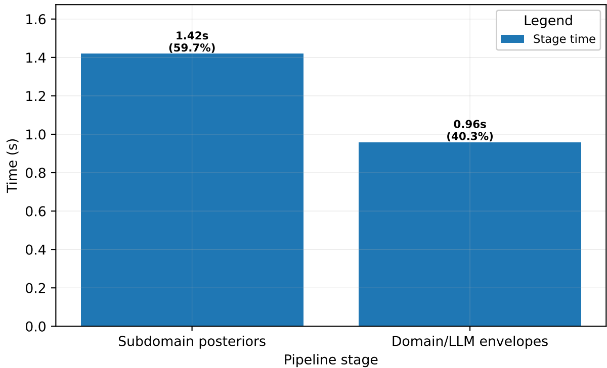
Baseline timing breakdown ( m=2, n=2, K=160, S=3000, T=201 )
