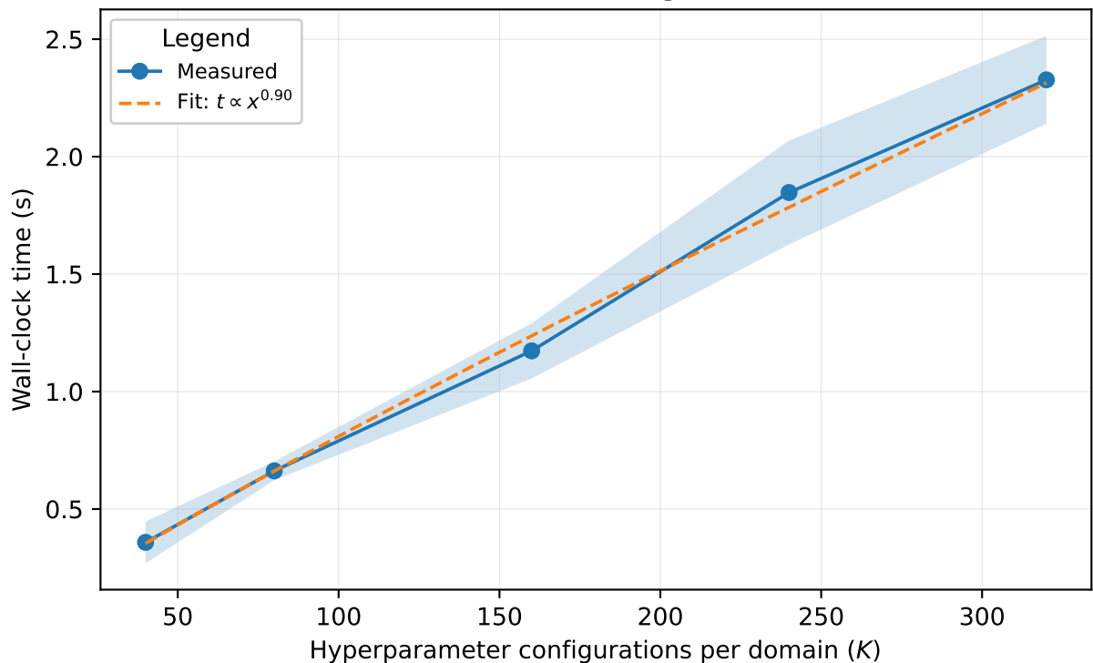
HIP-LLM scaling vs K
