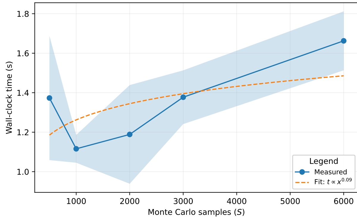
HIP-LLM scaling vs S
