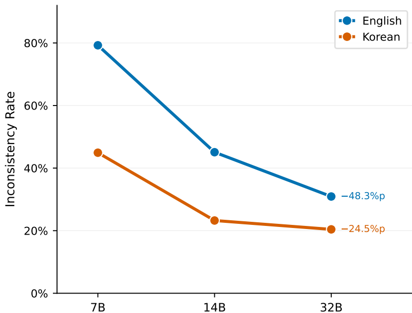
(a) Same-family: Qwen scaling
