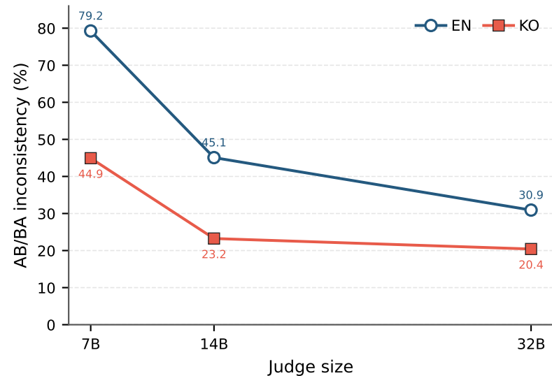
(a) Same-family judge scaling
