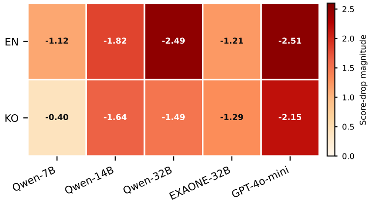
(a) Reference-guided score drop
