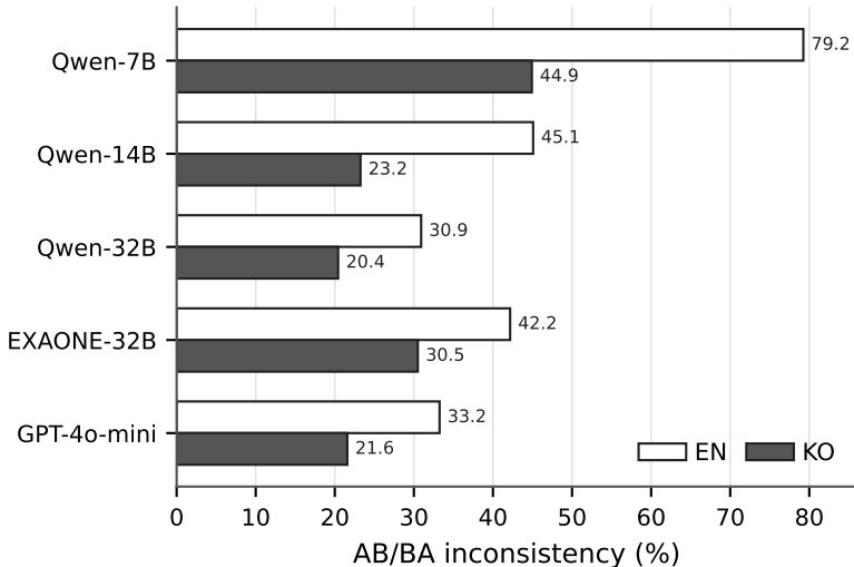
(a) Order-swap inconsistency
