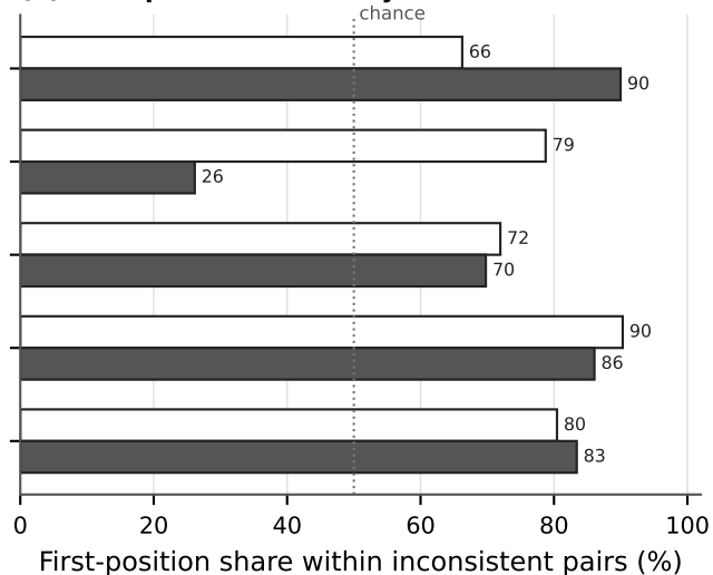
(b) First-position tendency
