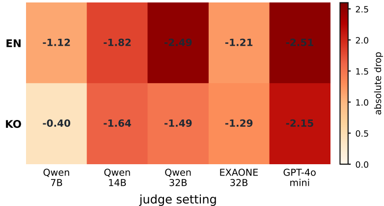
(a) Reference-guided score drop
