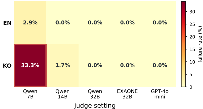
(b) Reference parse failure
