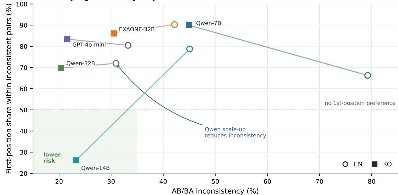
Pairwise judge reliability map
