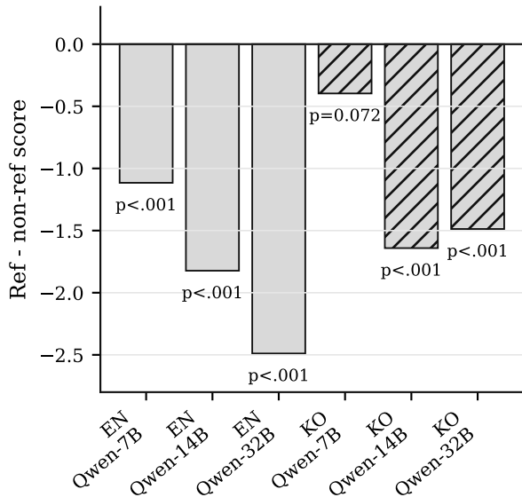
(a) Reference-guided scoring
