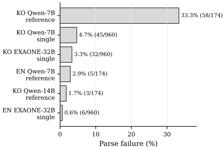
(b) Highest parse-failure settings
