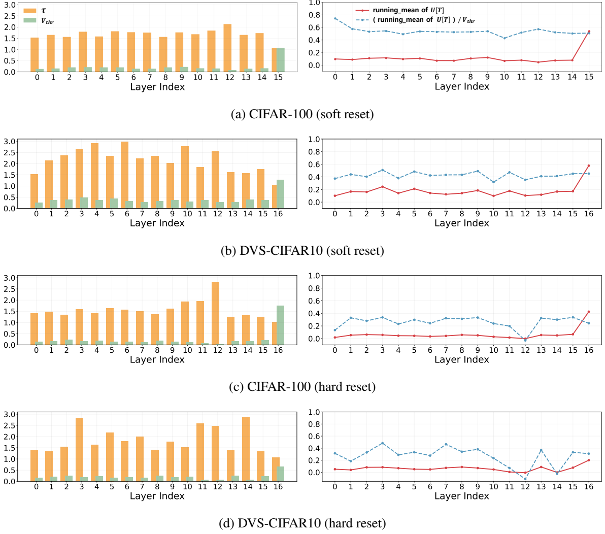
Figure 6.12: Final values of V_{thr} , \tau , and the running mean of U[T] after training. ResNet-19 on CIFAR-100 ( T = 4 ) and DVS-CIFAR10 ( T = 10 ).
