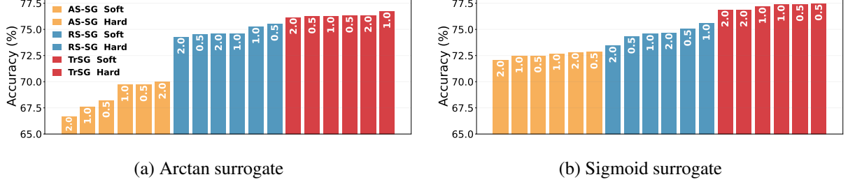
Figure 6.9: Accuracy under different initial V_{thr} \in \{0.5, 1.0, 2.0\} for Arctan and Sigmoid surrogates ( \tau = 2.0 ). We compare AS-SG, RS-SG, and TrSG on ResNet-19 (CIFAR-100, T = 4 ), evaluating both soft- and hard-reset LIF neurons.
