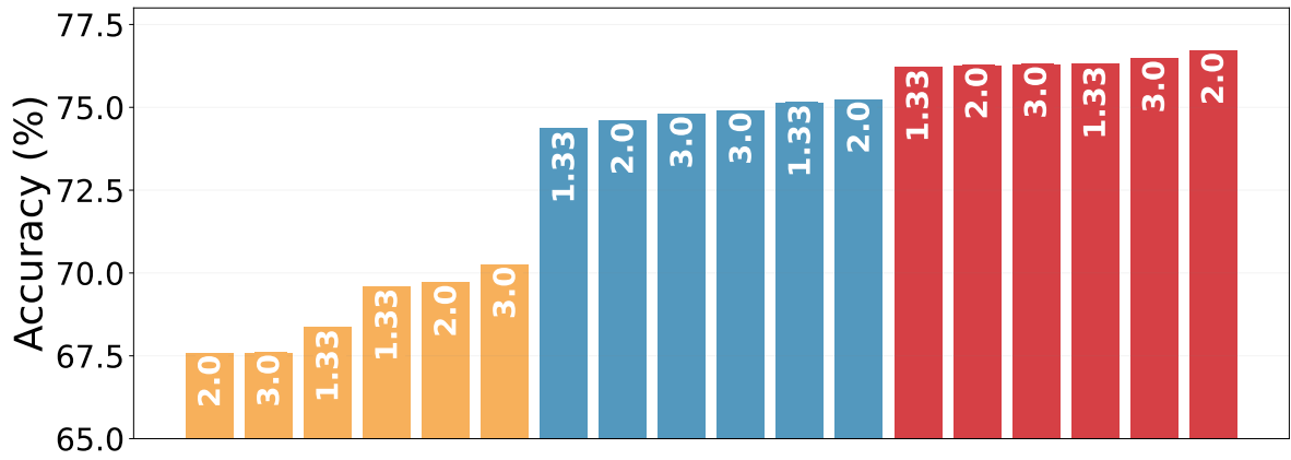
(b) Arctan: V_{thr} = 1.0 , \tau \in \{1.33, 2.0, 3.0\}
