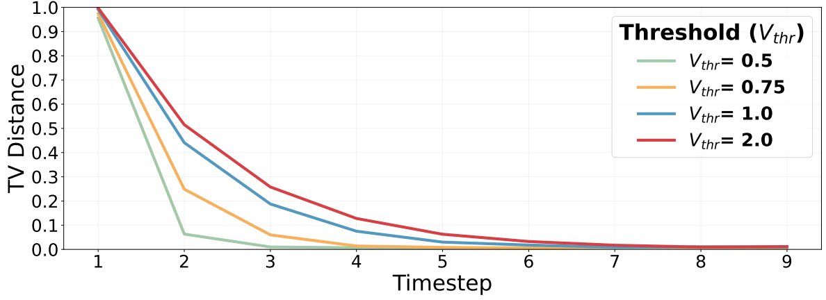
(a) Impact of varying V_{thr} on convergence speed.
