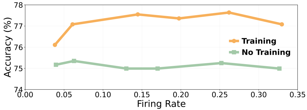
Figure 6.10: Accuracy vs. firing rate under TrSG. We sweep a sparsity loss [49] to match global firing rates and compare Training (learn V_{\text{thr}} and \tau with TrSG) against No Training (both frozen).
