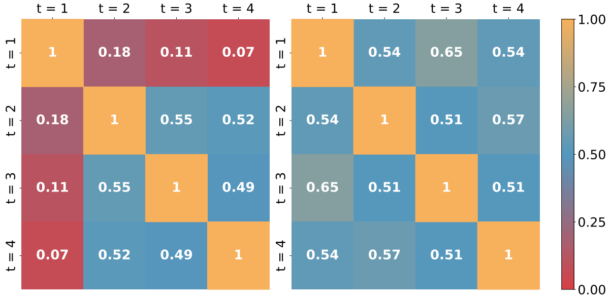
Figure 4.7: Gradient conflicts across timesteps with and without MP-Init. Cosine similarity of gradients across timesteps in ResNet-19 on CIFAR-100. Left: Without MP-Init, the gradient from t = 1 strongly conflicts with later timesteps, reflecting the temporal inconsistency highlighted by MPS [32]. Right: With MP-Init, conflicts are largely resolved and similarities improve, indicating that MP-Init aligns temporal ensemble members and stabilizes training.
