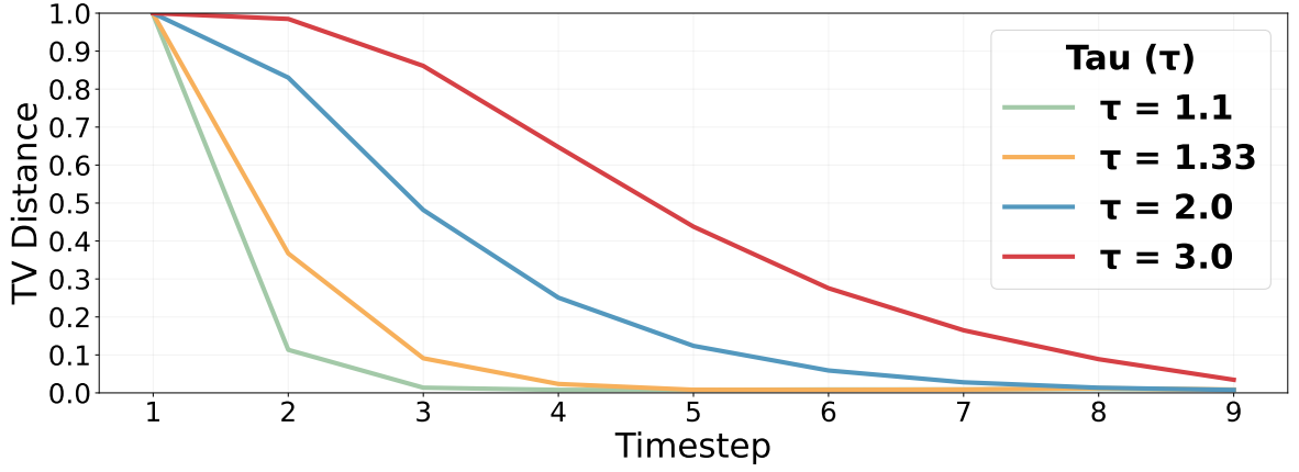
(b) Impact of varying \tau on convergence speed.
