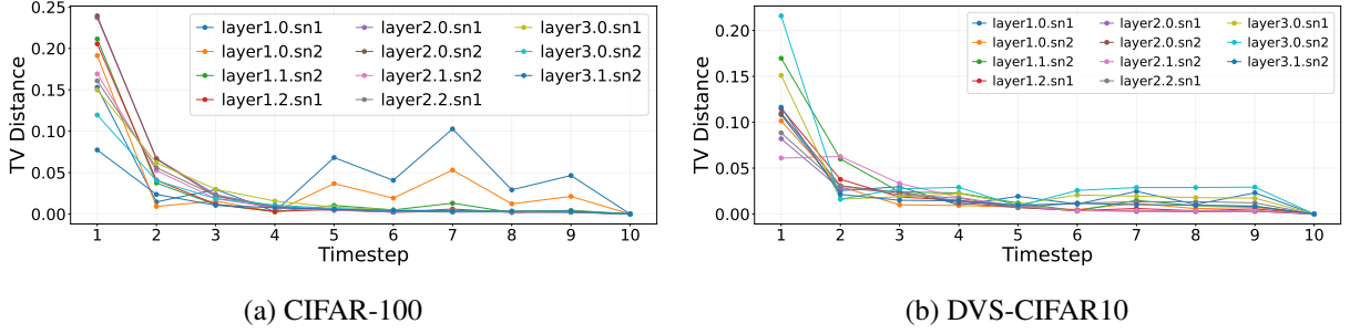
Figure 4.6: TV distance from the input distribution as t increases.
