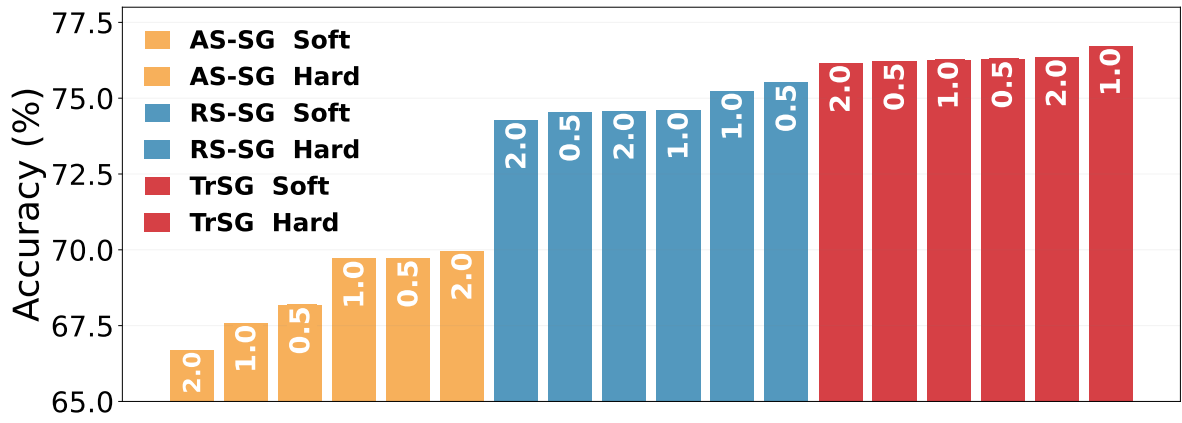
(a) Arctan: \tau = 2.0 , V_{thr} \in \{0.5, 1.0, 2.0\}
