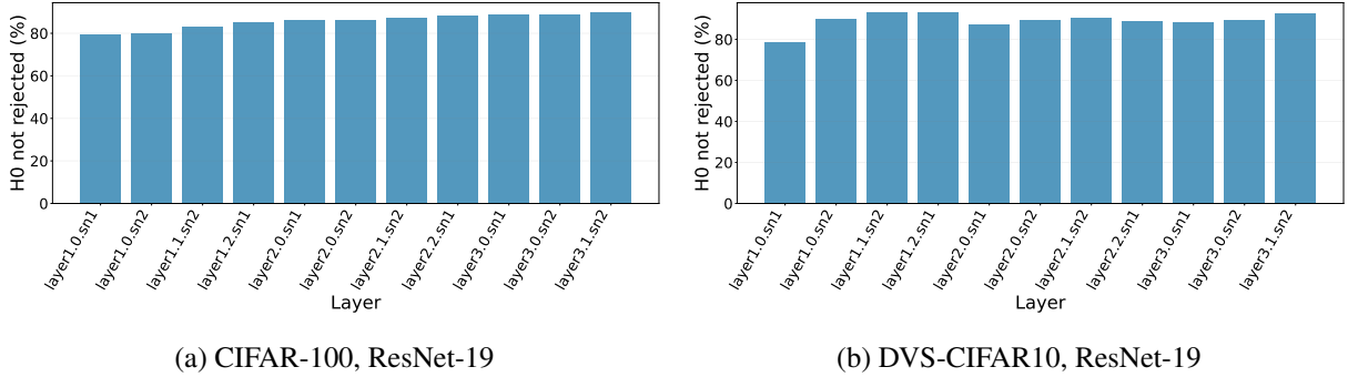
Figure 4.3: Ljung–Box test (lag 1) for the presynaptic input across layers and timesteps.
