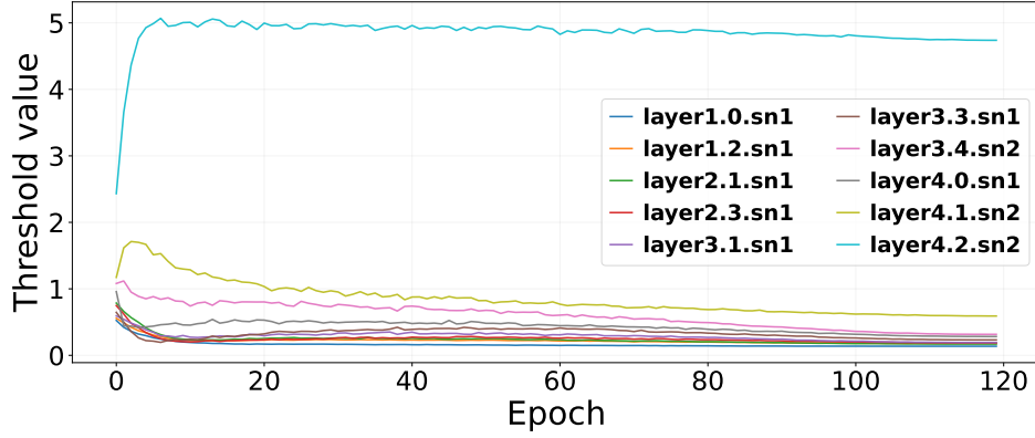
(c) ResNet-34 on ImageNet
