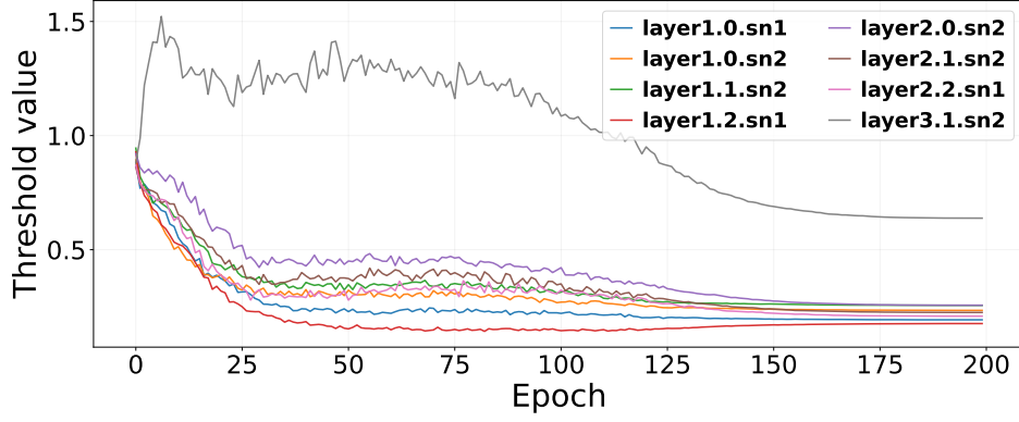
(b) ResNet-19 on DVS-CIFAR10
