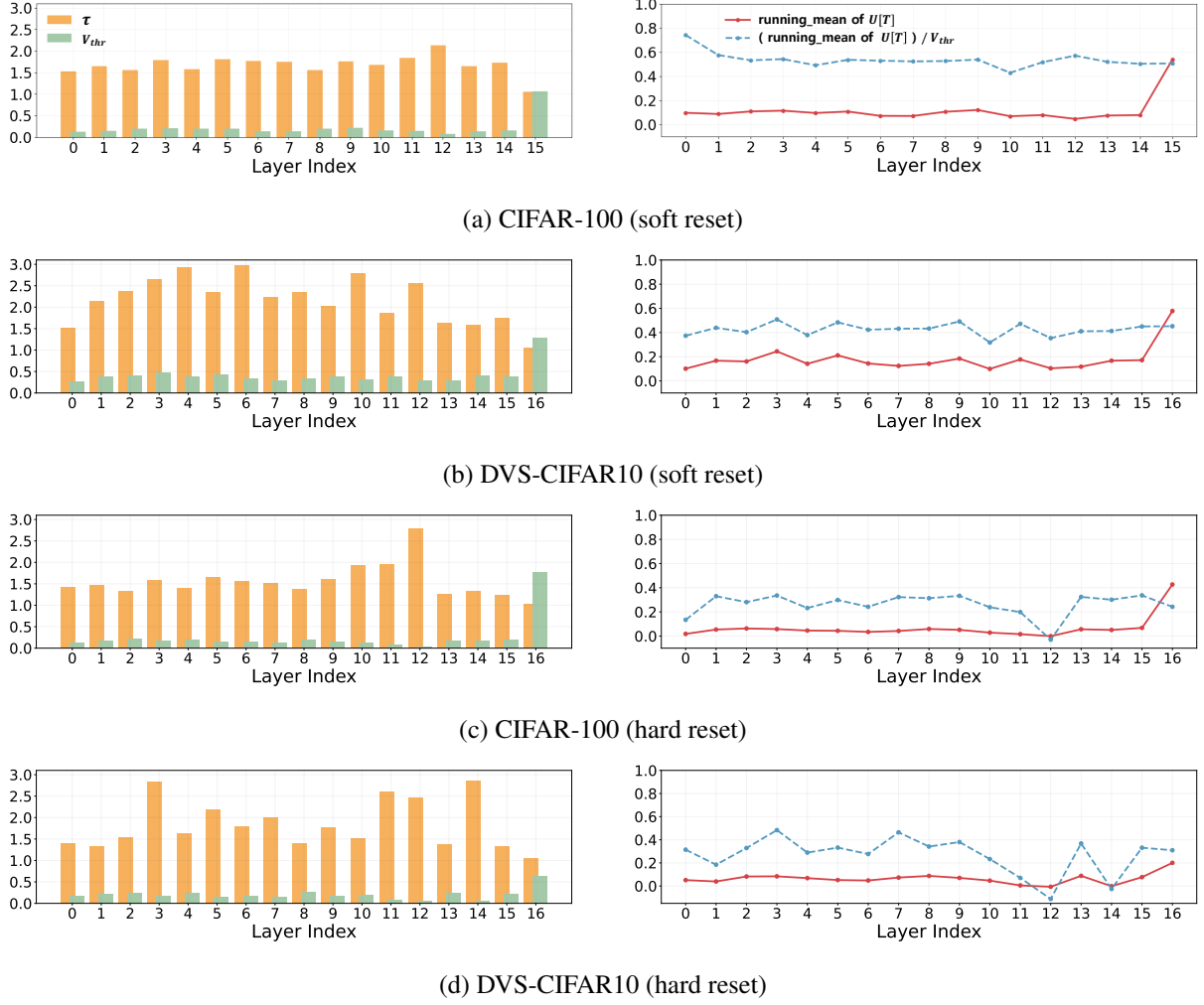
Figure 6.12: Final values of V_{thr} , \tau , and the running mean of U[T] after training. ResNet-19 on CIFAR-100 ( T = 4 ) and DVS-CIFAR10 ( T = 10 ).
