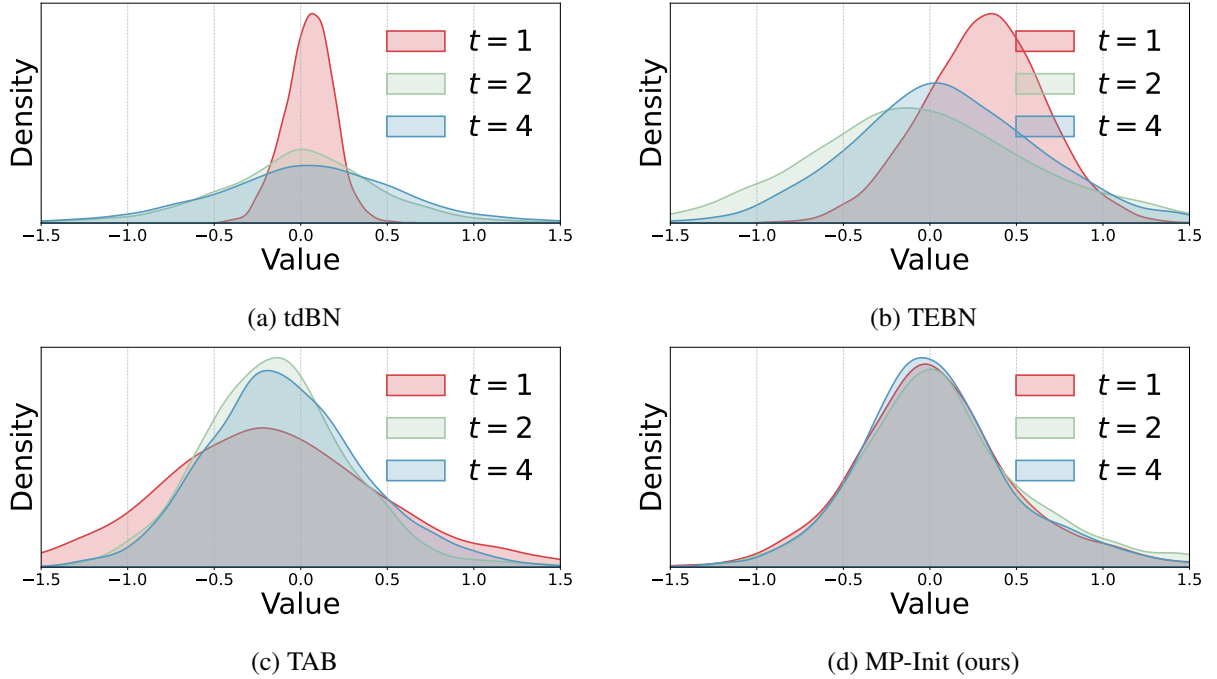
Figure 4.2: Activation (presynaptic input) distributions of the convolutional layer following the third spiking layer of ResNet-19 on CIFAR-100. The drift visible in TEBN and TAB collapses under MP-Init.
