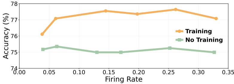
Figure 6.11: Accuracy vs. firing rate under TrSG. We sweep a sparsity loss [49] to match global firing rates and compare Training (learn V_{\text{thr}} and \tau with TrSG) against No Training (both frozen).
