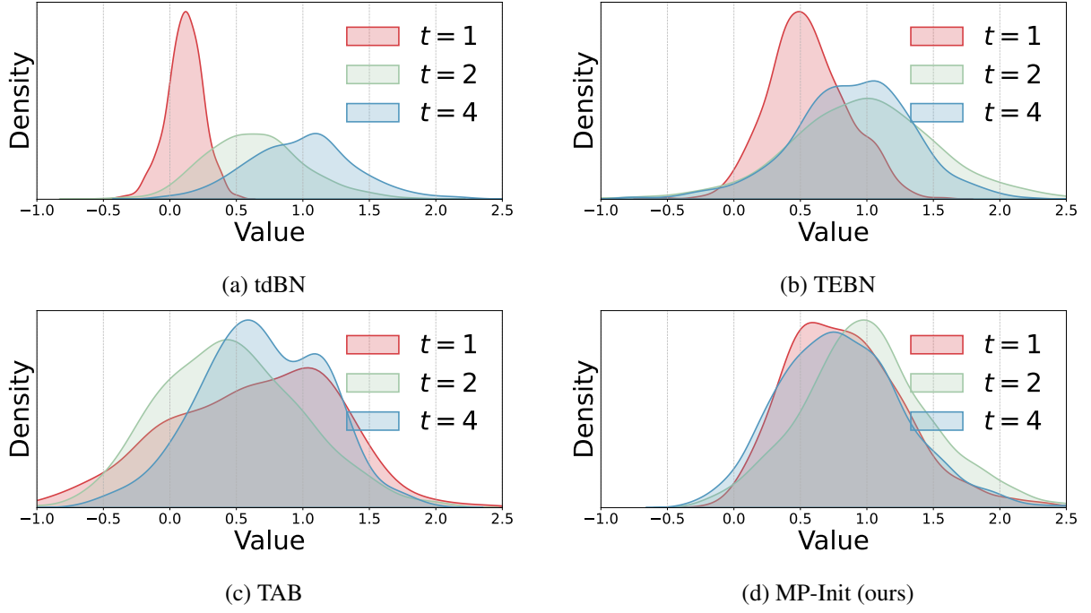
Figure 4.1: Membrane potential distributions across timesteps at the third spiking layer of ResNet-19 on CIFAR-100. Existing TCS-aware normalizations (TEBN, TAB) still leave a temporal drift in the membrane potential, while MP-Init aligns the per-timestep distributions.
