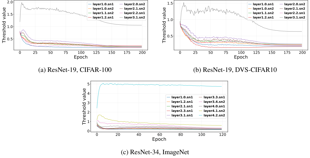
Figure 6.8: Trajectories of trainable V_{\text{thr}} during training. Early layers tend to settle at lower thresholds, while late or deep layers move toward larger thresholds.
