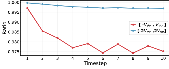
(a) CIFAR-100
