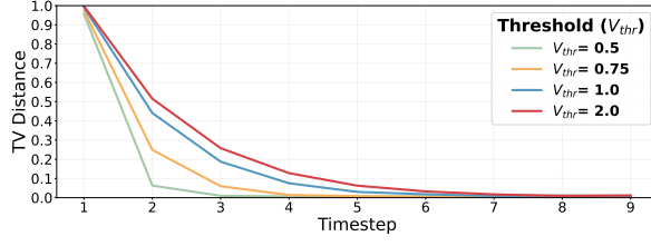
(a) Impact of varying V_{thr} on convergence speed.
