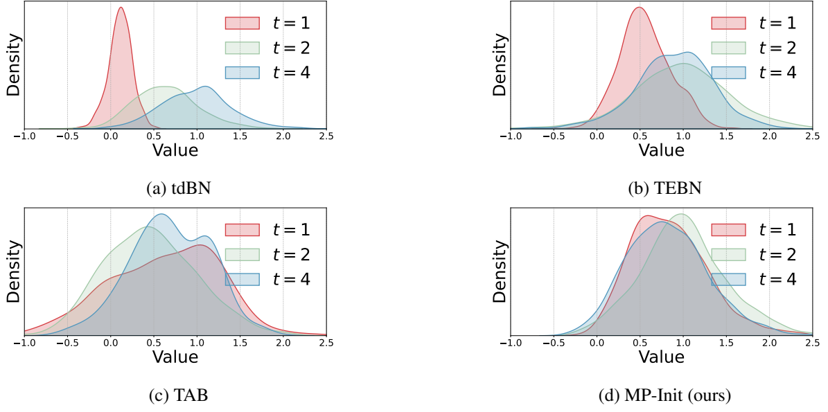
Figure 4.1: Membrane potential distributions across timesteps at the third spiking layer of ResNet-19 on CIFAR-100. Existing TCS-aware normalizations (TEBN, TAB) still leave a temporal drift in the membrane potential, while MP-Init aligns the per-timestep distributions.
