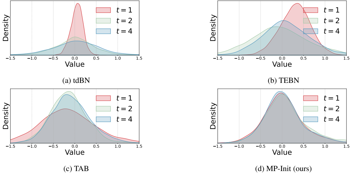
Figure 4.2: Activation (presynaptic input) distributions of the convolutional layer following the third spiking layer of ResNet-19 on CIFAR-100. The drift visible in TEBN and TAB collapses under MP-Init.
