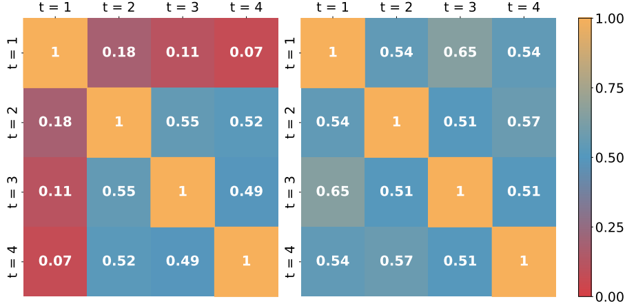
Figure 6.7: Gradient conflicts across timesteps with and without MP-Init. Cosine similarity of gradients across timesteps in ResNet-19 on CIFAR-100. Left: Without MP-Init, the gradient from t = 1 strongly conflicts with later timesteps, reflecting the temporal inconsistency highlighted by MPS [32]. Right: With MP-Init, conflicts are largely resolved and similarities improve, indicating that MP-Init aligns temporal ensemble members and stabilizes training.
