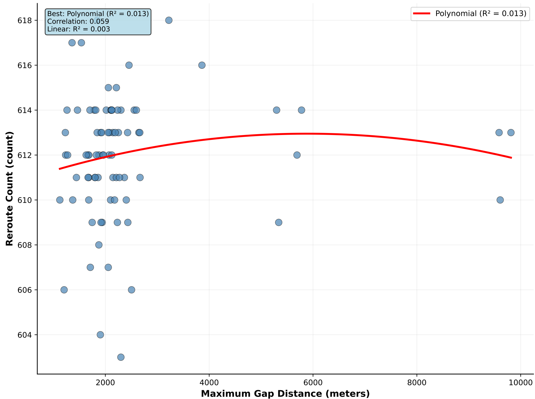
Maximum Gap Distance vs Reroute Count
