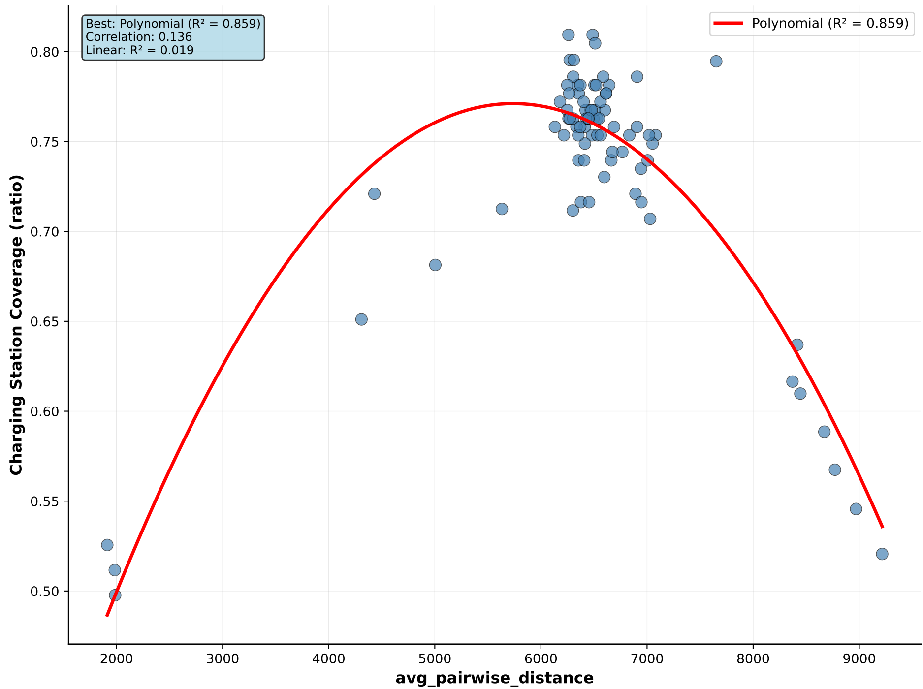
avg_pairwise_distance vs Charging Station Coverage
