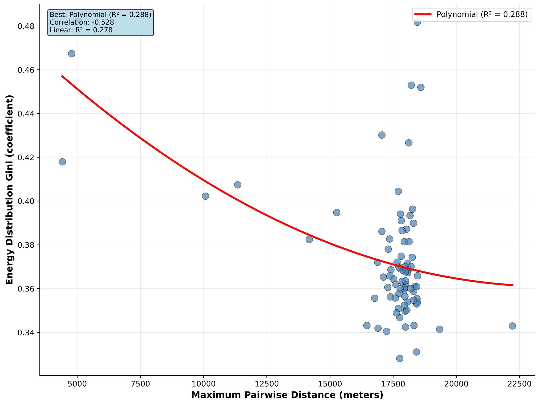
Maximum Pairwise Distance vs Energy Distribution Gini
