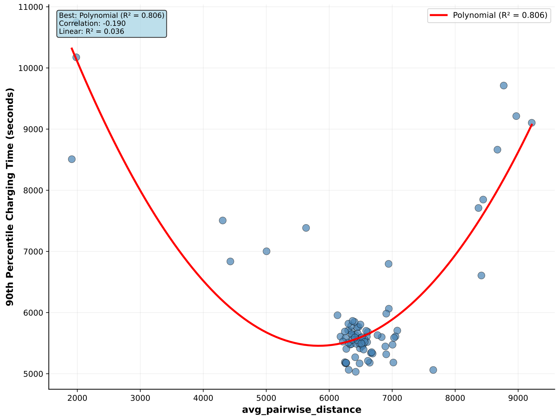
avg_pairwise_distance vs 90th Percentile Charging Time
