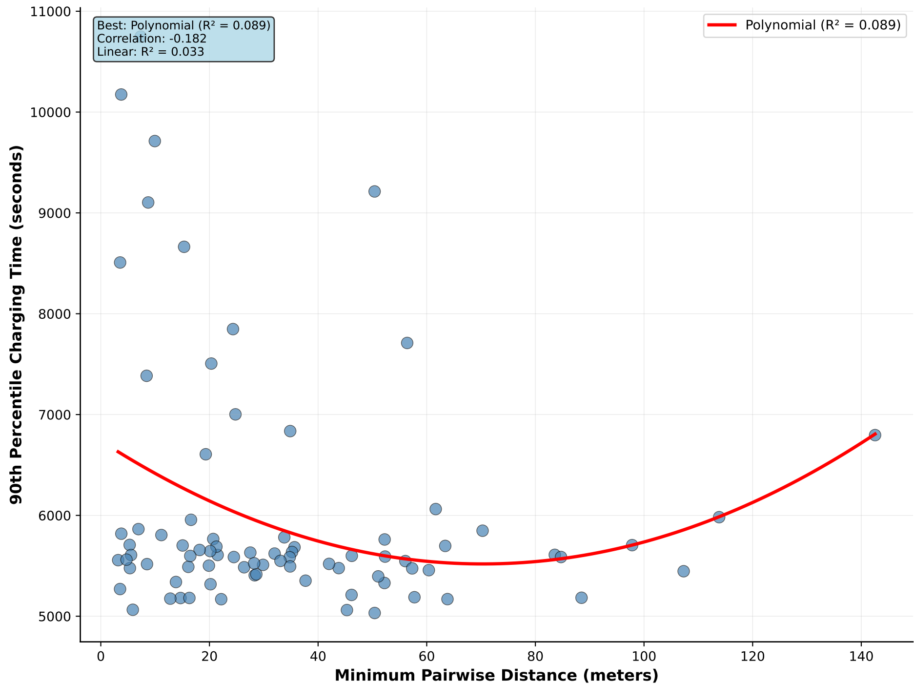
Minimum Pairwise Distance vs 90th Percentile Charging Time
