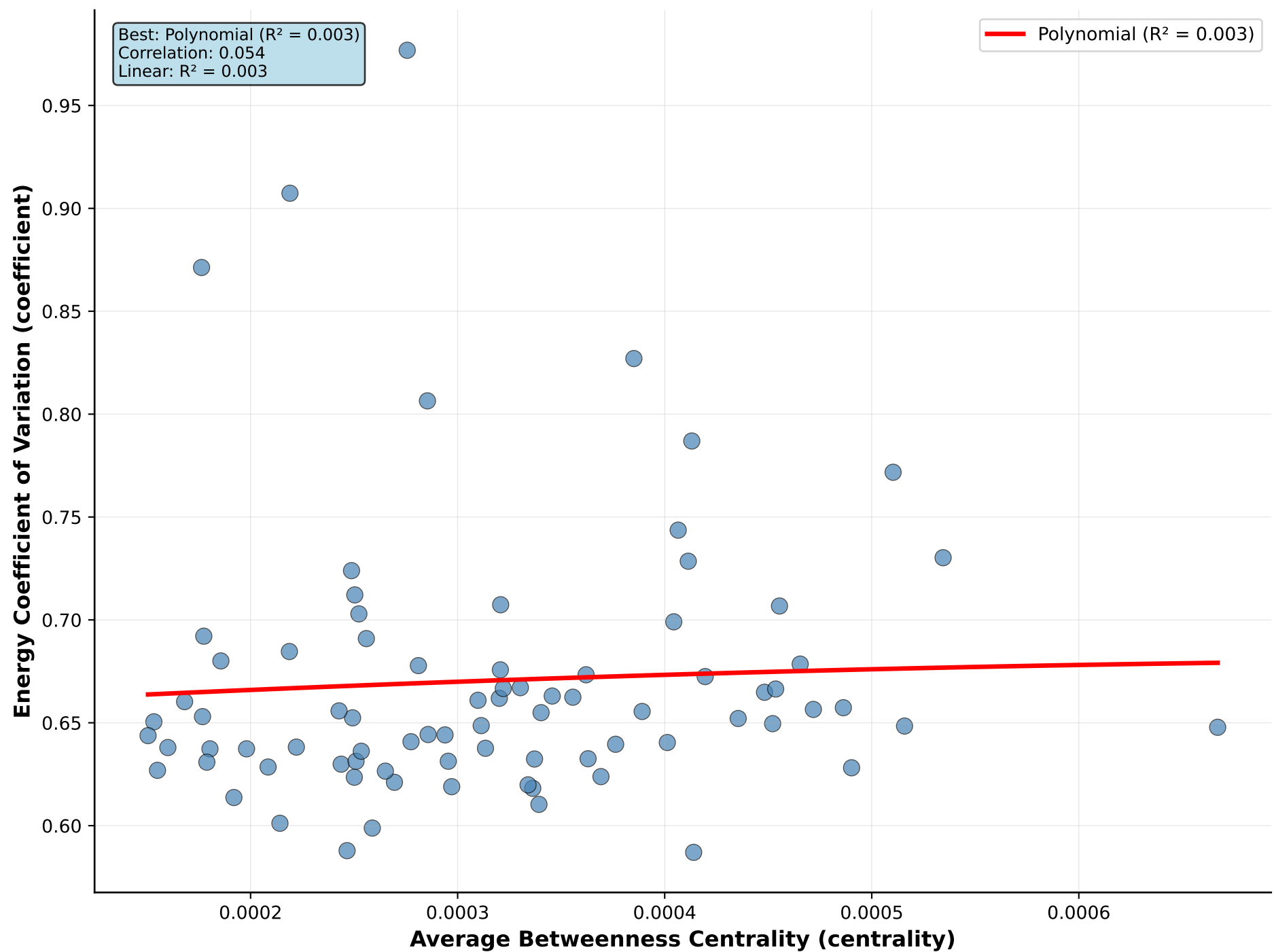
Average Betweenness Centrality vs Energy Coefficient of Variation
