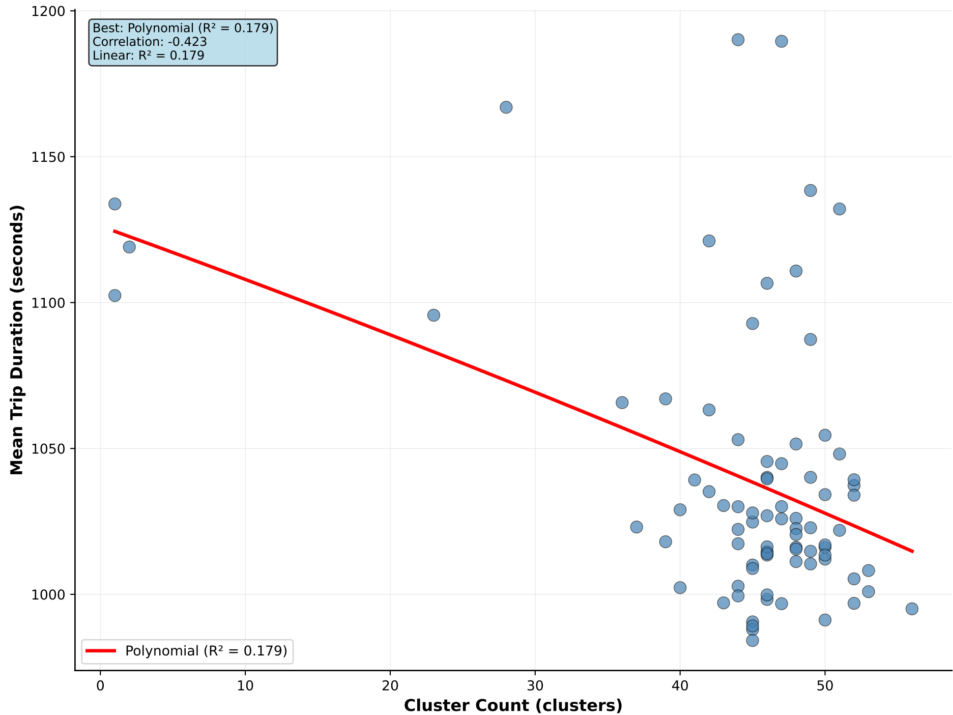
Cluster Count vs Mean Trip Duration
