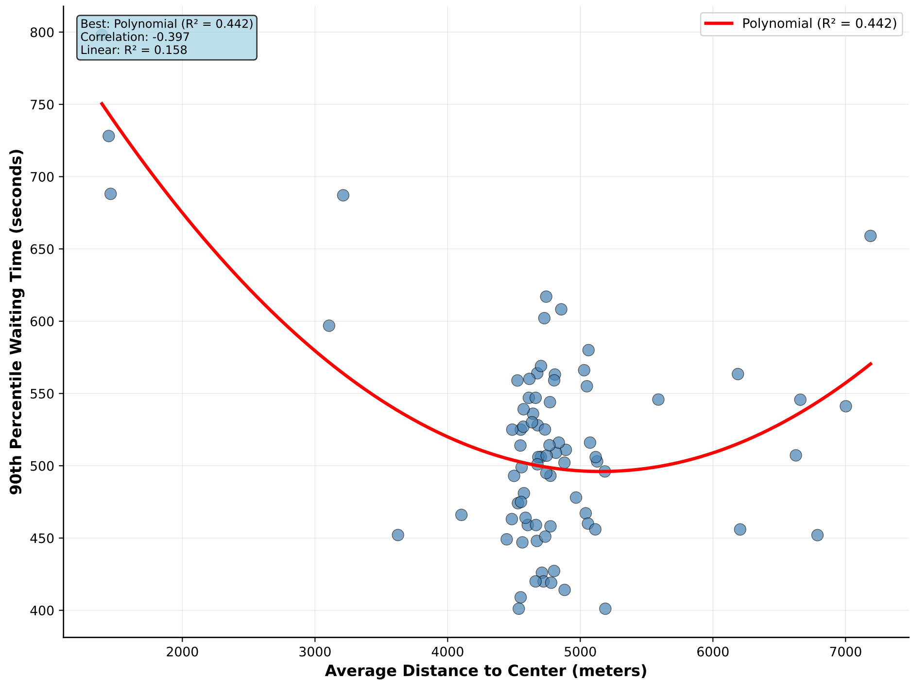
Average Distance to Center vs 90th Percentile Waiting Time
