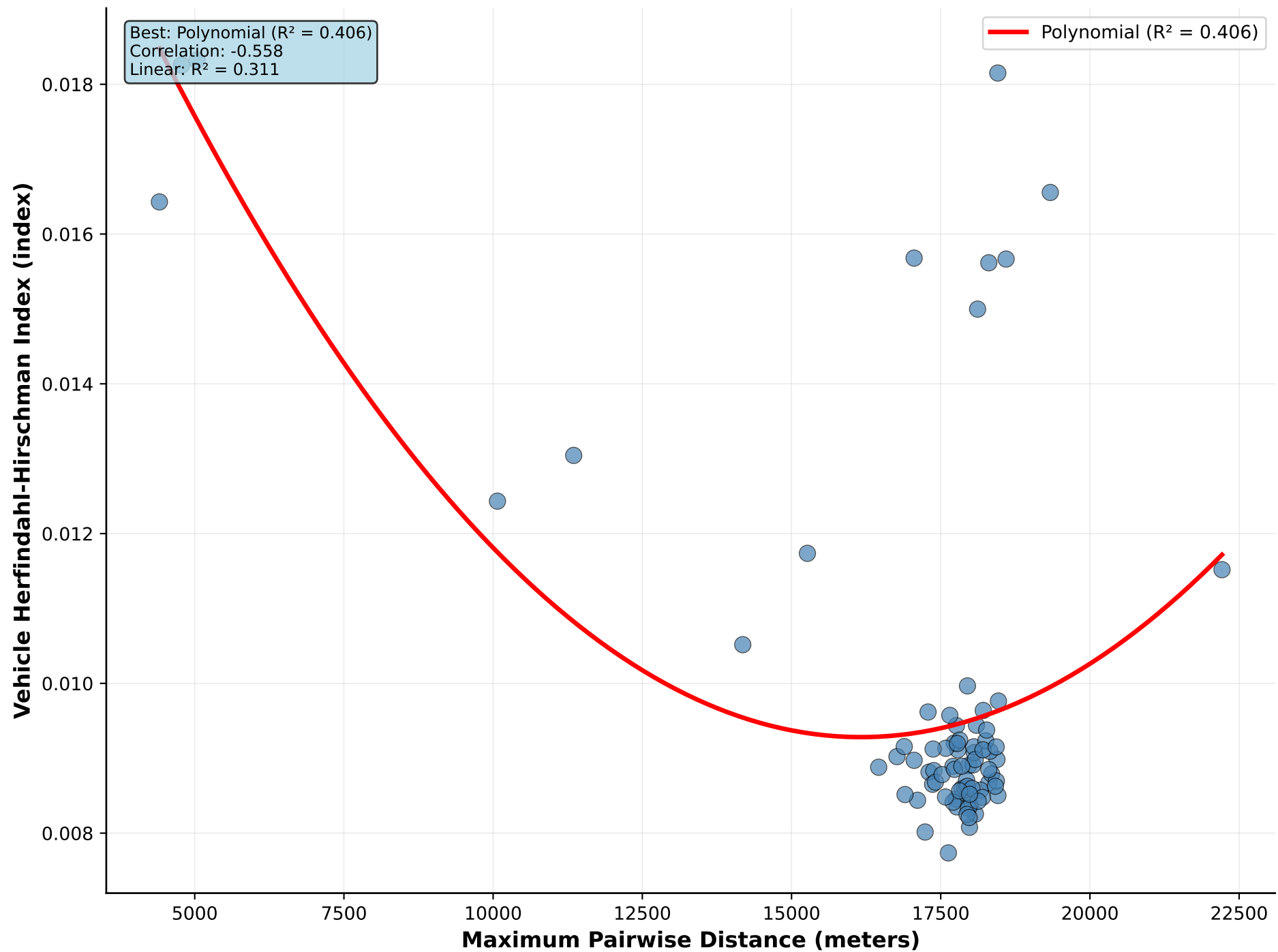
Maximum Pairwise Distance vs Vehicle Herfindahl-Hirschman Index
