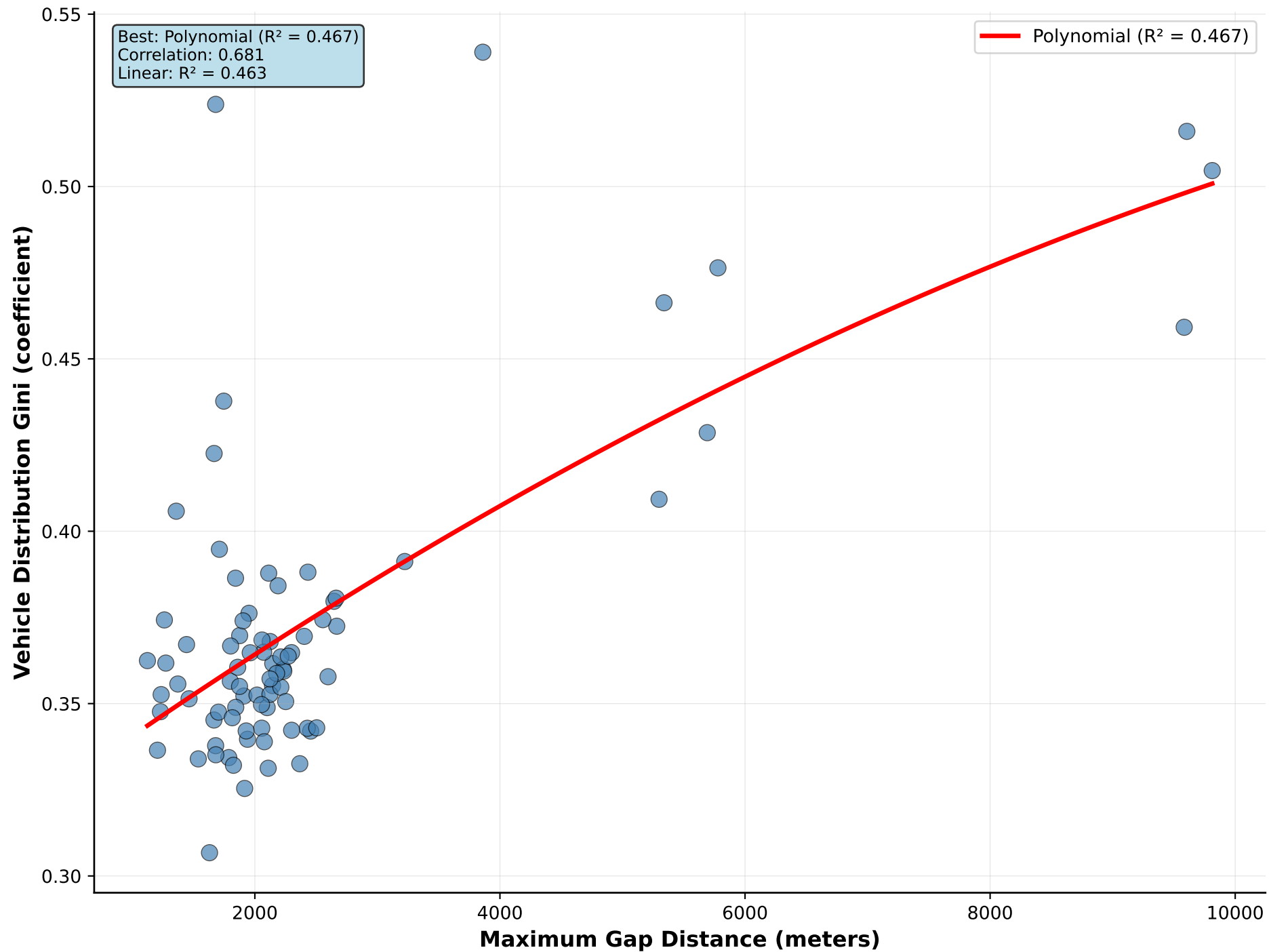
Maximum Gap Distance vs Vehicle Distribution Gini
