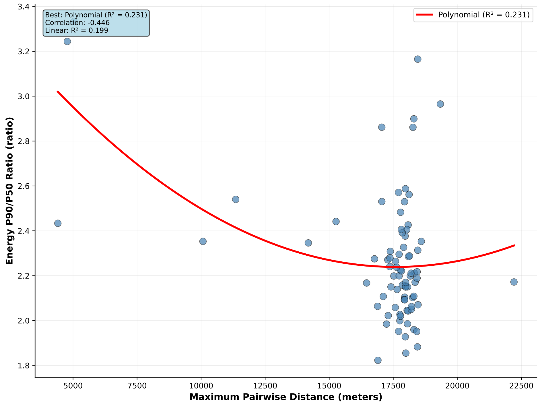
Maximum Pairwise Distance vs Energy P90/P50 Ratio
