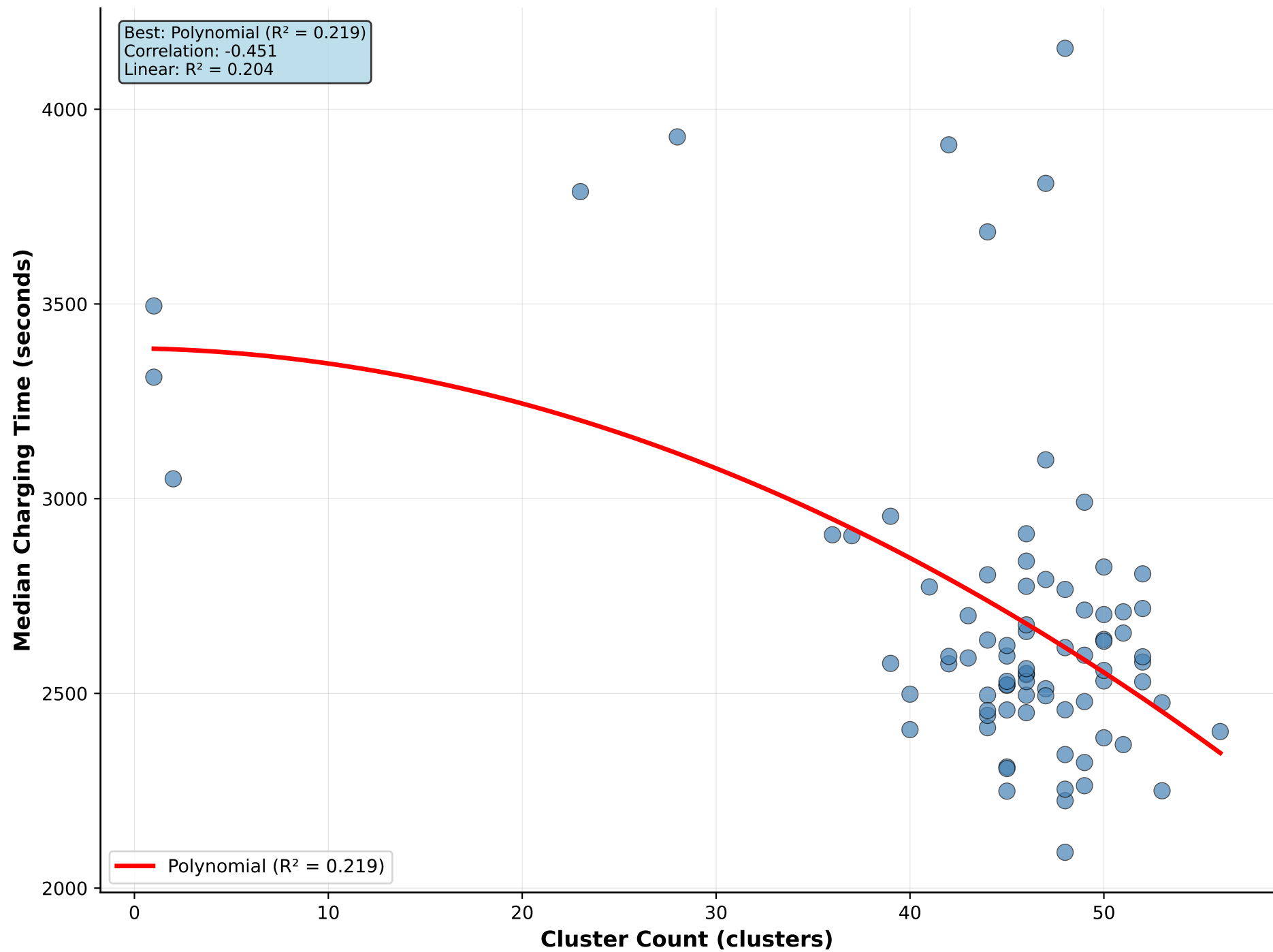
Cluster Count vs Median Charging Time
