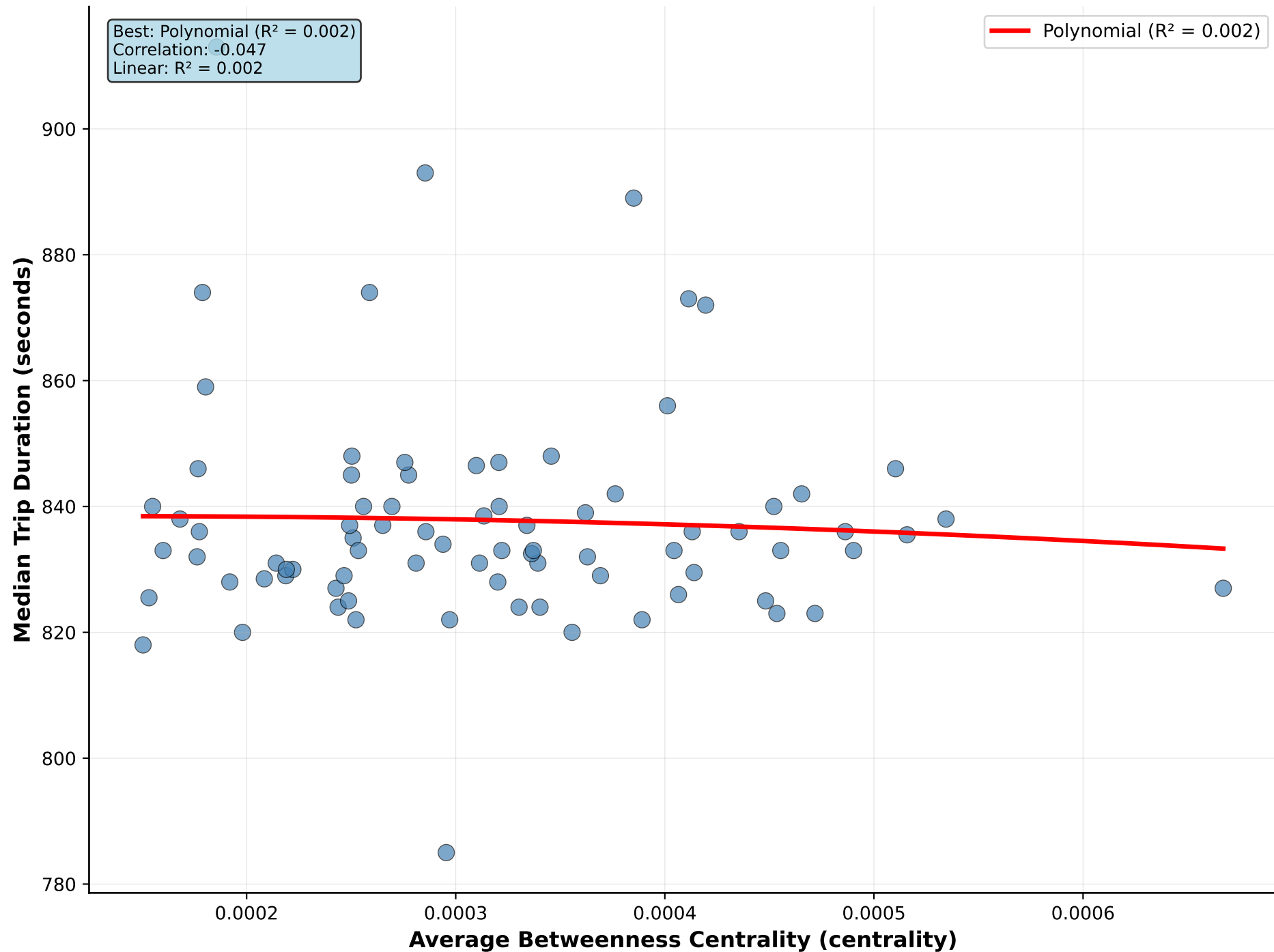
Average Betweenness Centrality vs Median Trip Duration
