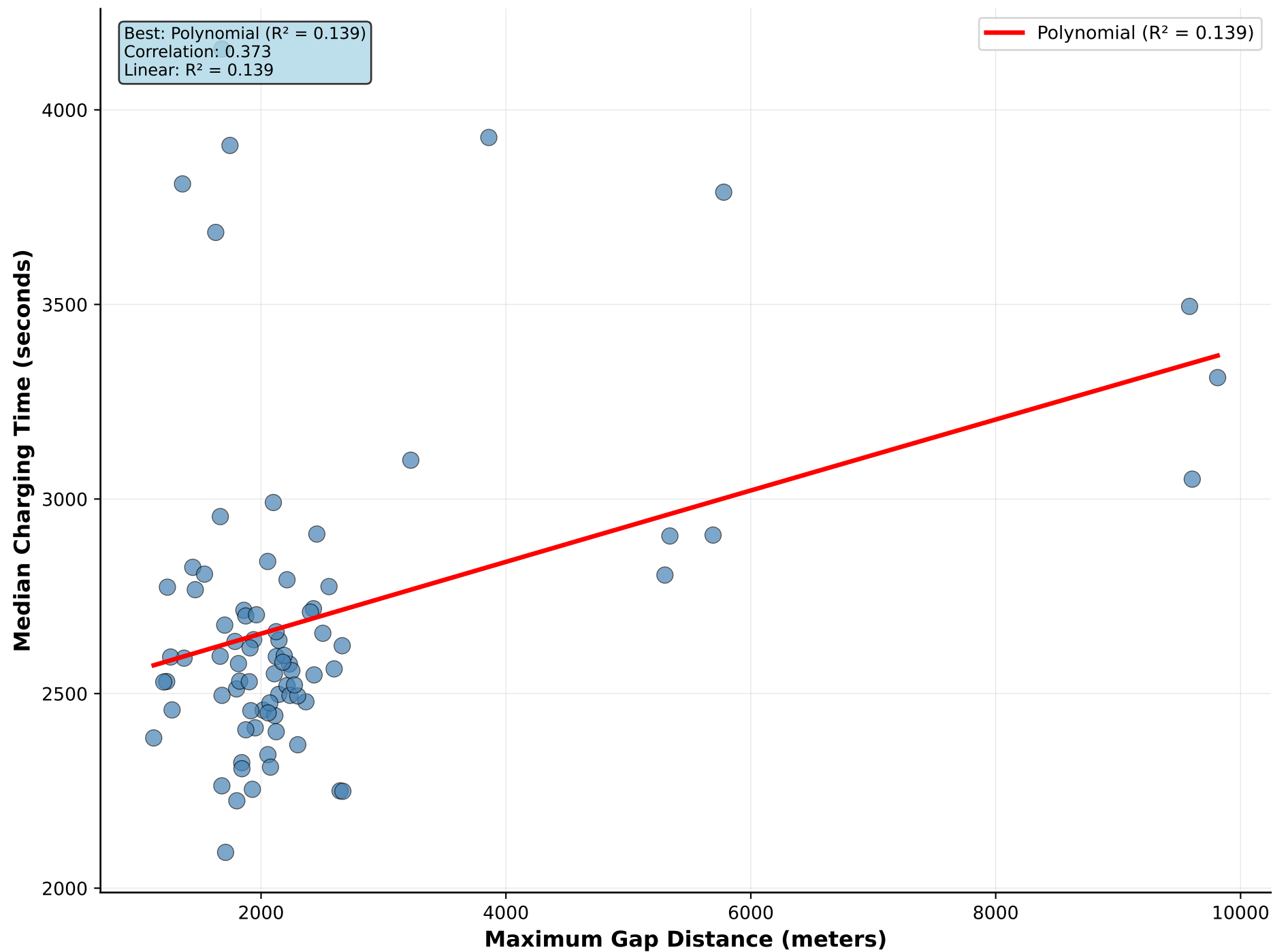
Maximum Gap Distance vs Median Charging Time
