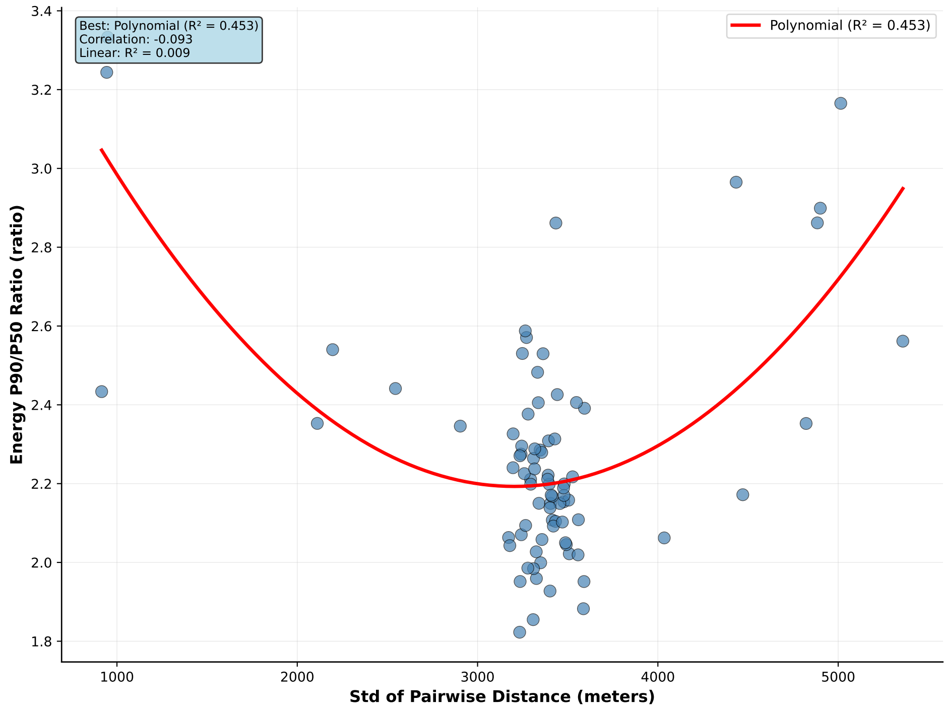
Std of Pairwise Distance vs Energy P90/P50 Ratio
