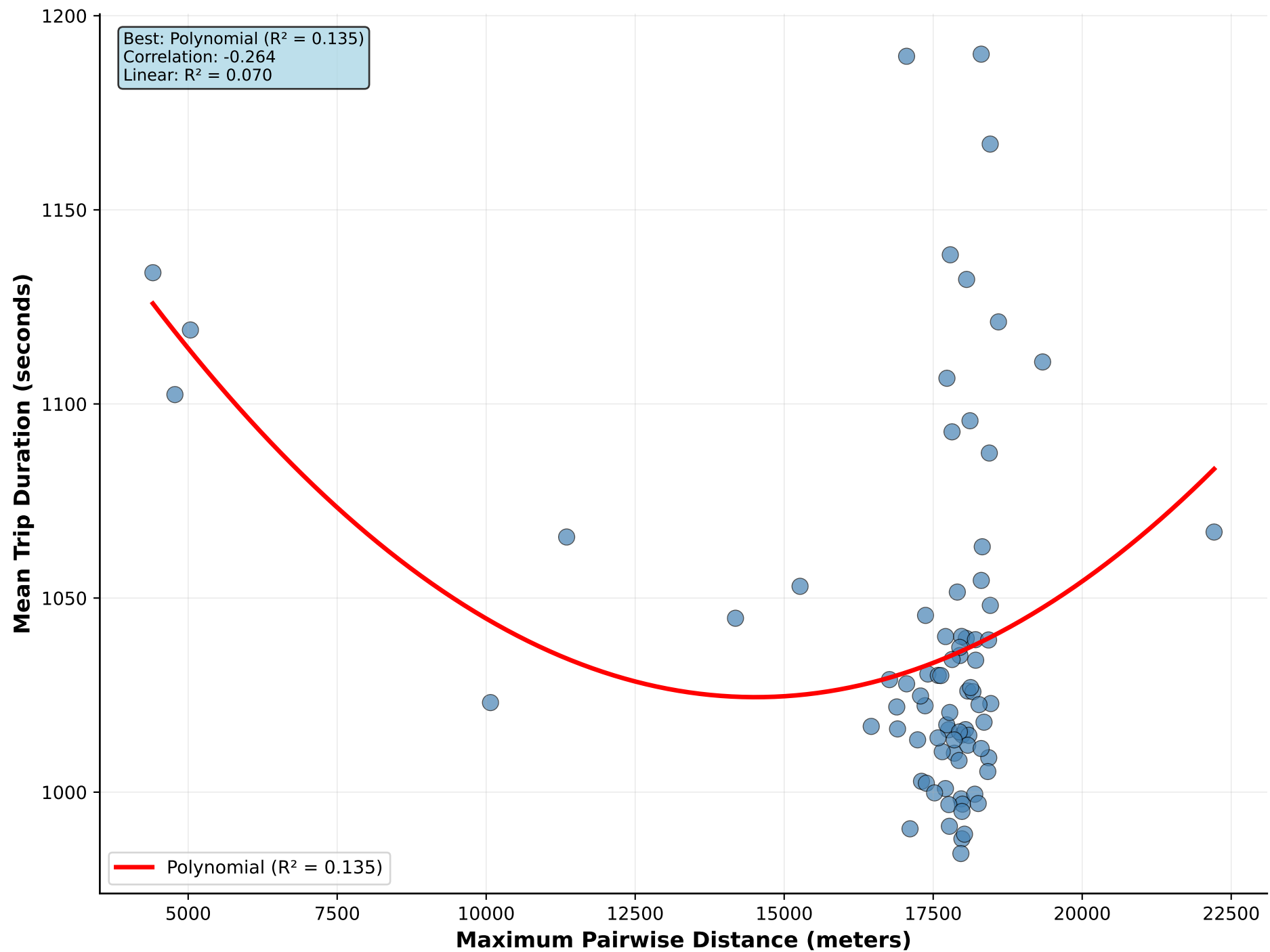
Maximum Pairwise Distance vs Mean Trip Duration
