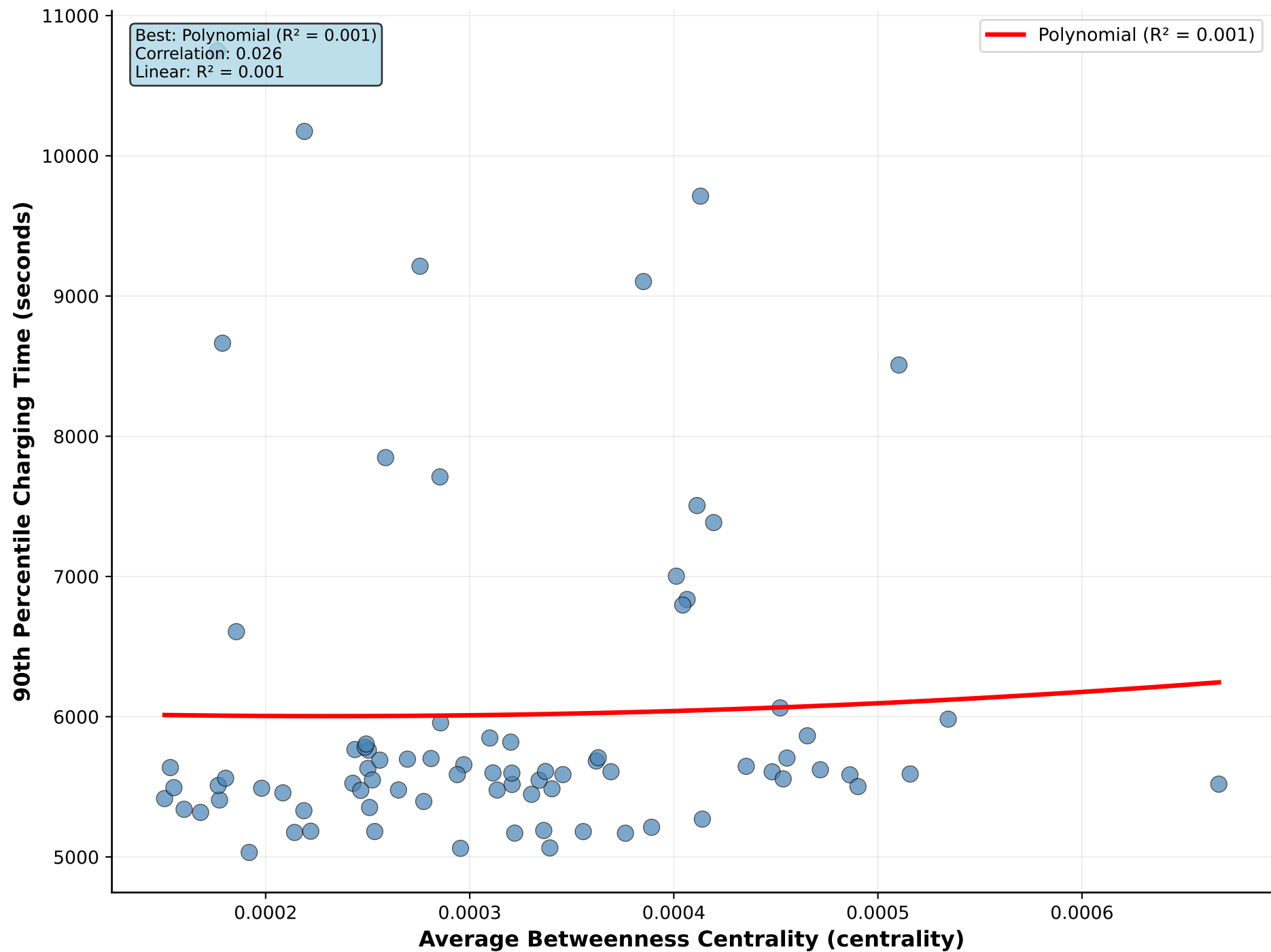
Average Betweenness Centrality vs 90th Percentile Charging Time
