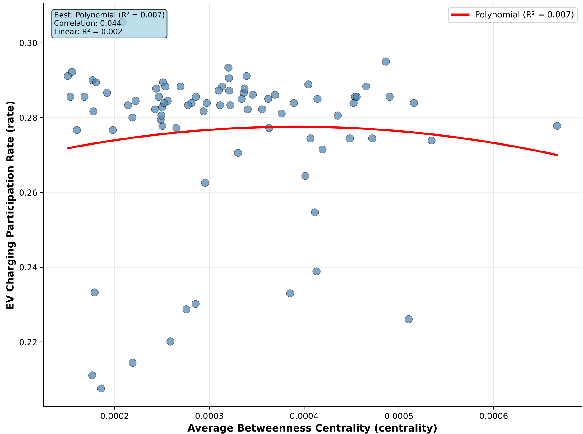
Average Betweenness Centrality vs EV Charging Participation Rate
