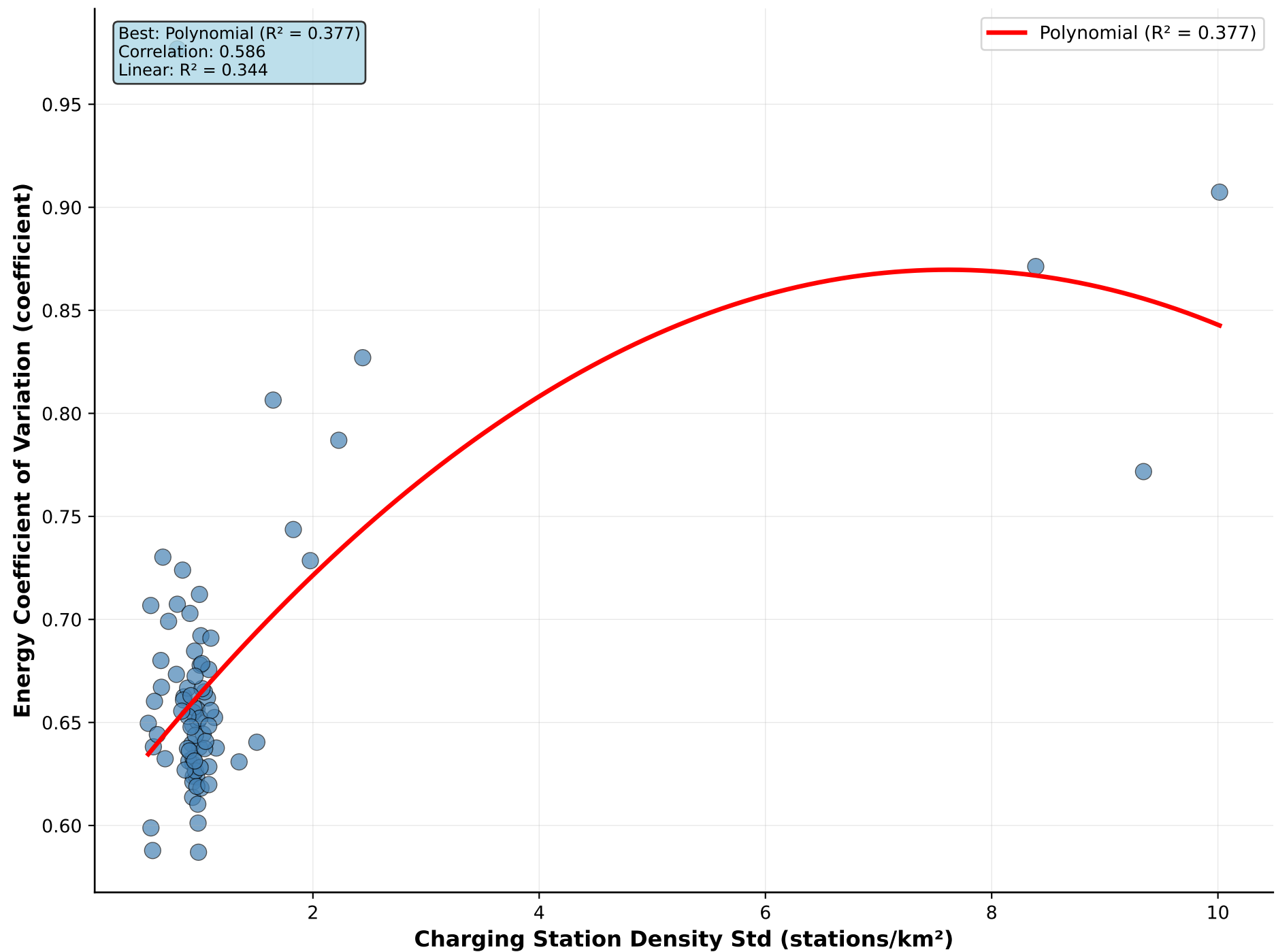
Charging Station Density Std vs Energy Coefficient of Variation
