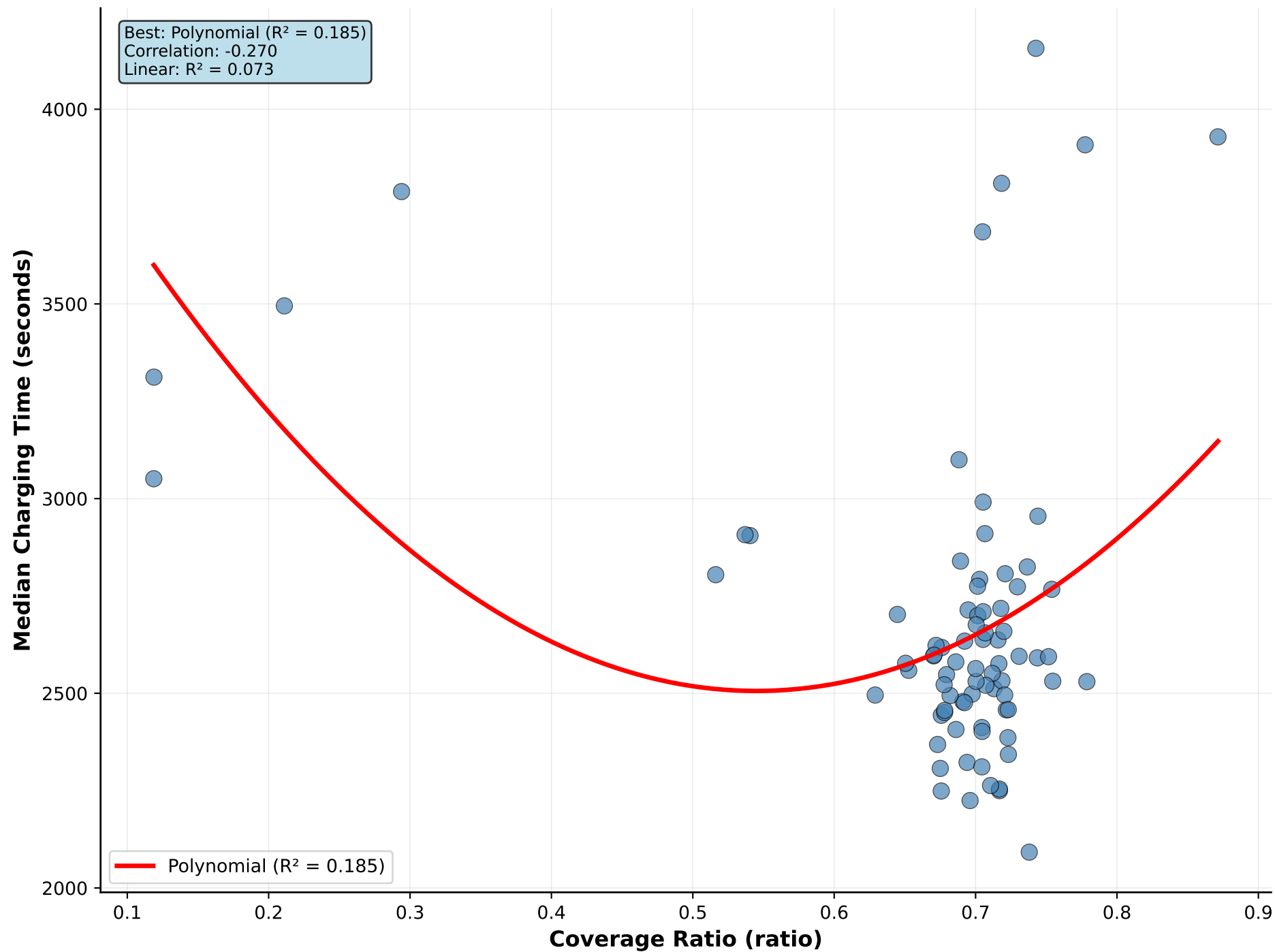
Coverage Ratio vs Median Charging Time
