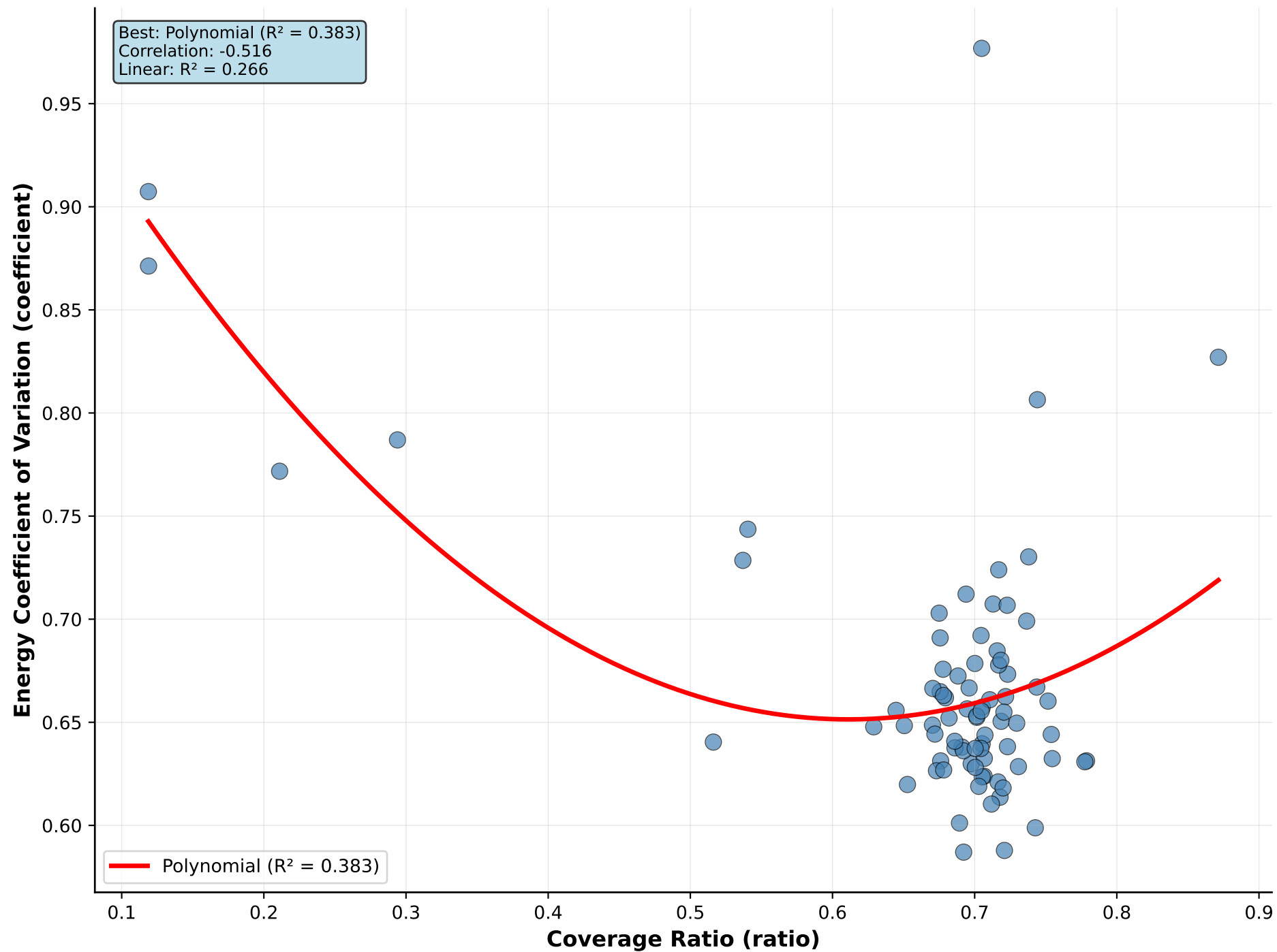
Coverage Ratio vs Energy Coefficient of Variation
