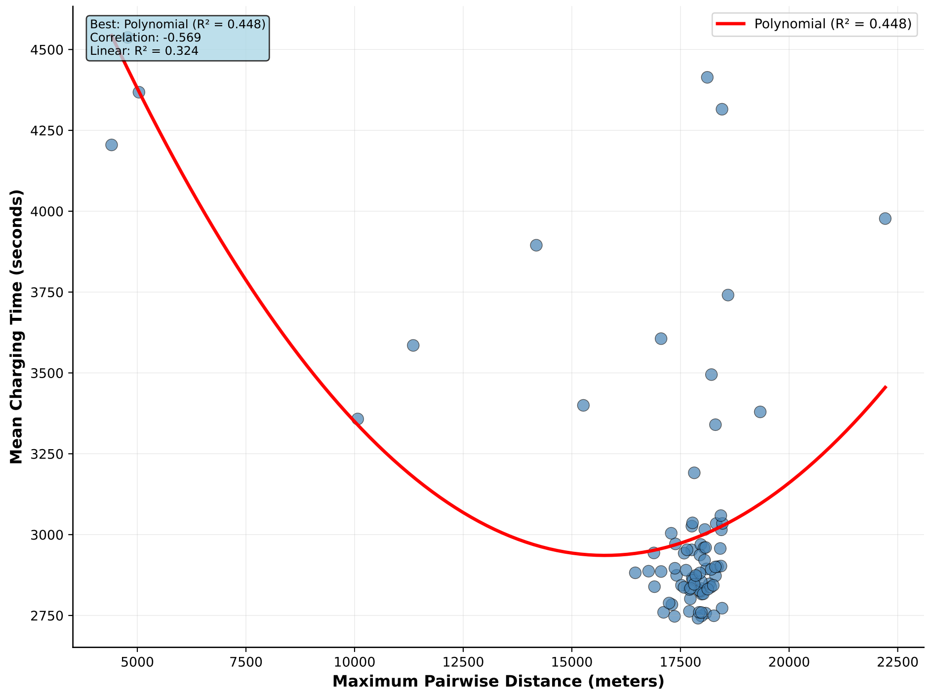
Maximum Pairwise Distance vs Mean Charging Time
