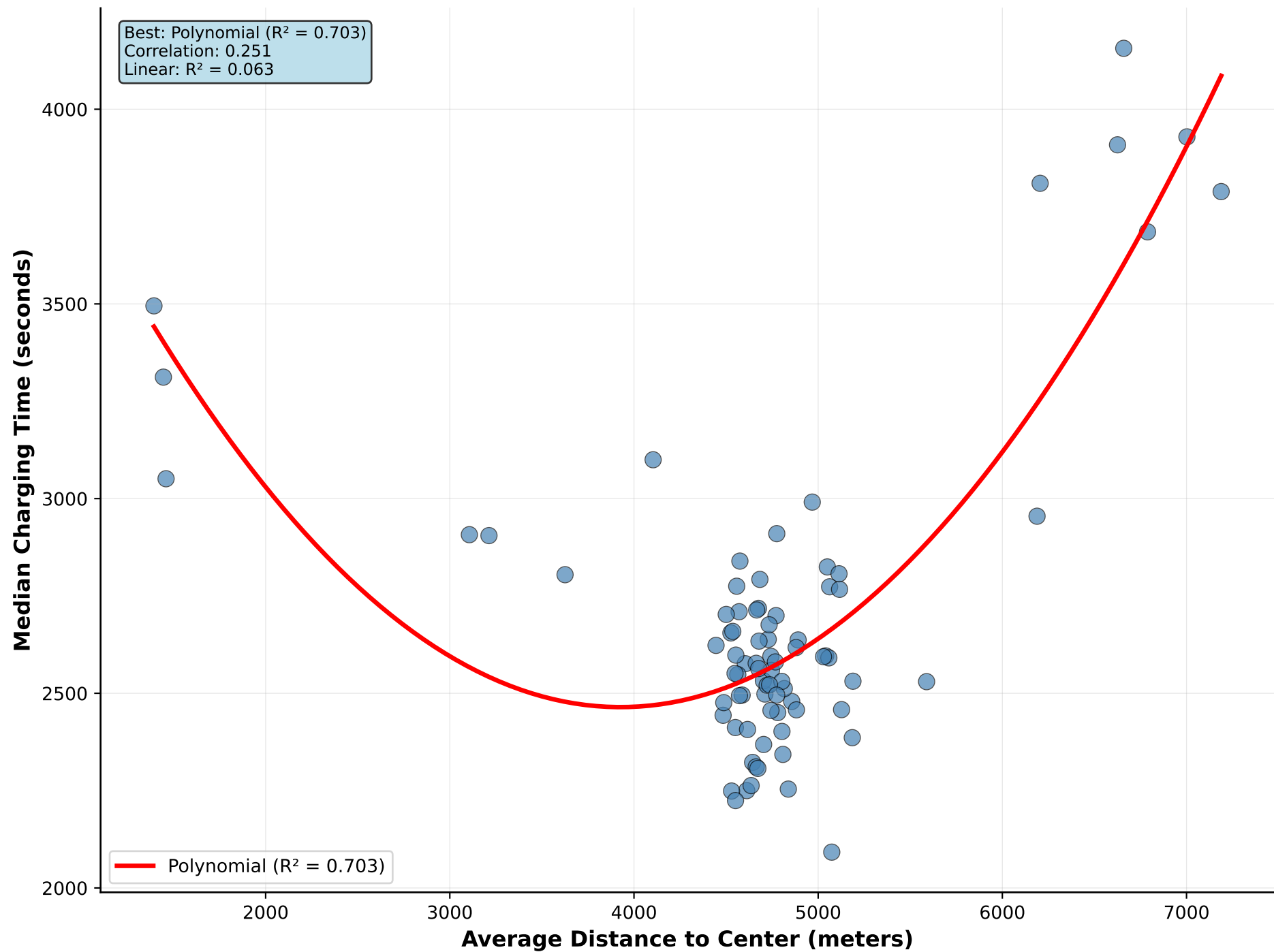
Average Distance to Center vs Median Charging Time
