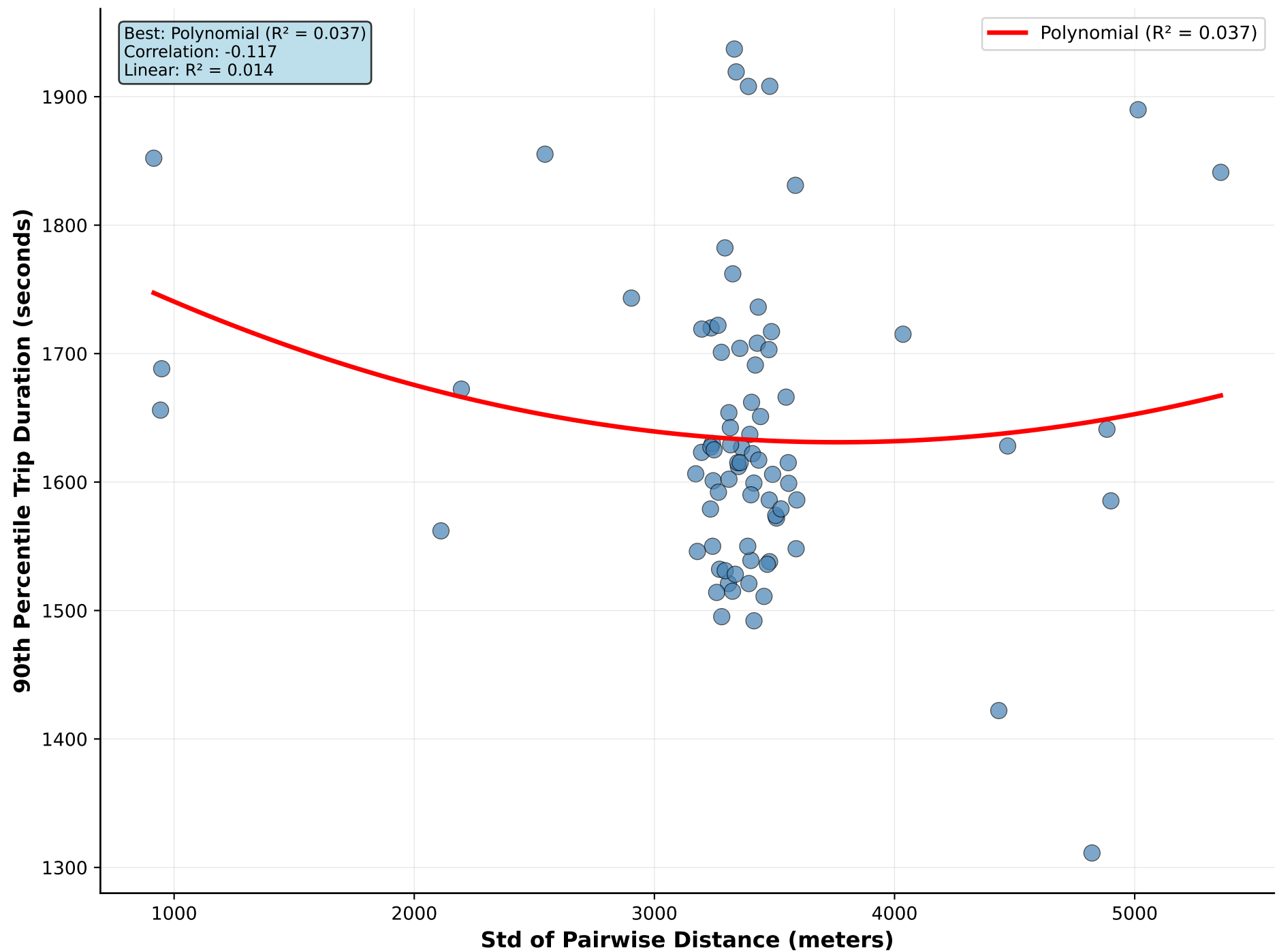
Std of Pairwise Distance vs 90th Percentile Trip Duration
