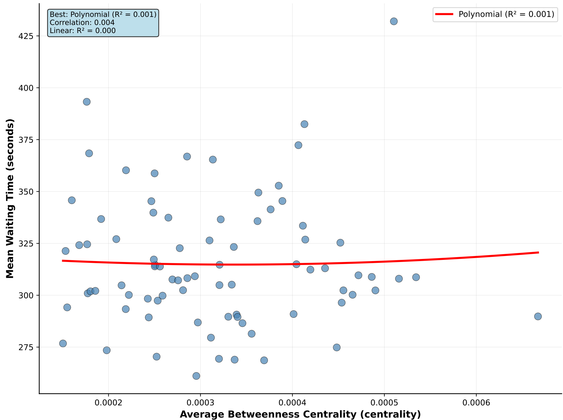
Average Betweenness Centrality vs Mean Waiting Time
