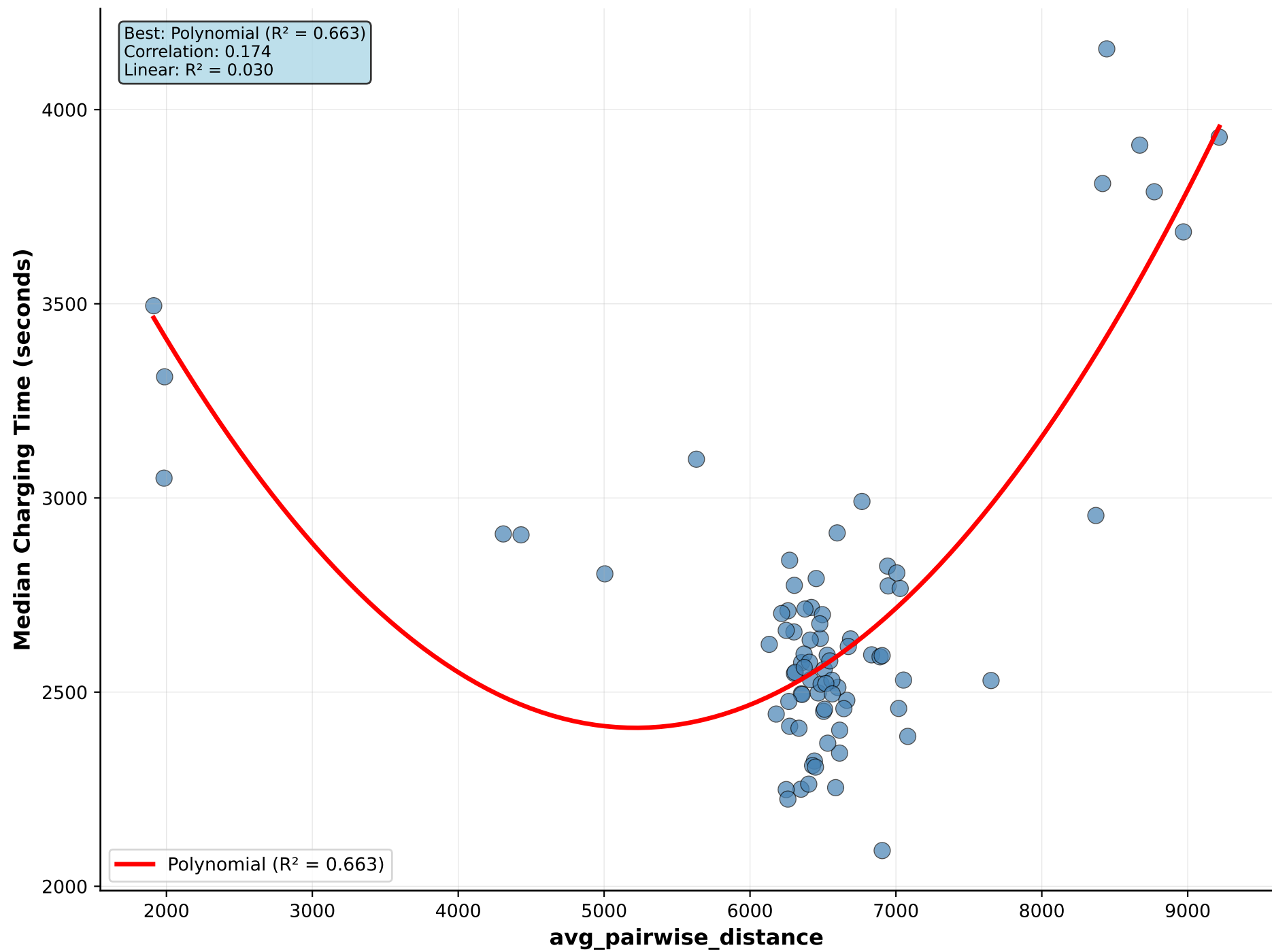
avg_pairwise_distance vs Median Charging Time
