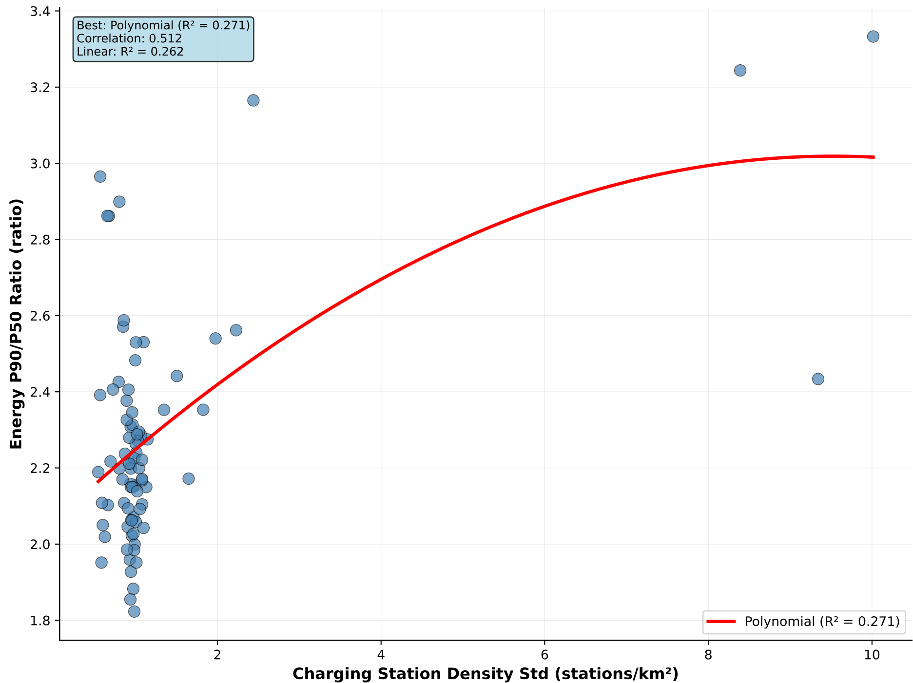
Charging Station Density Std vs Energy P90/P50 Ratio
