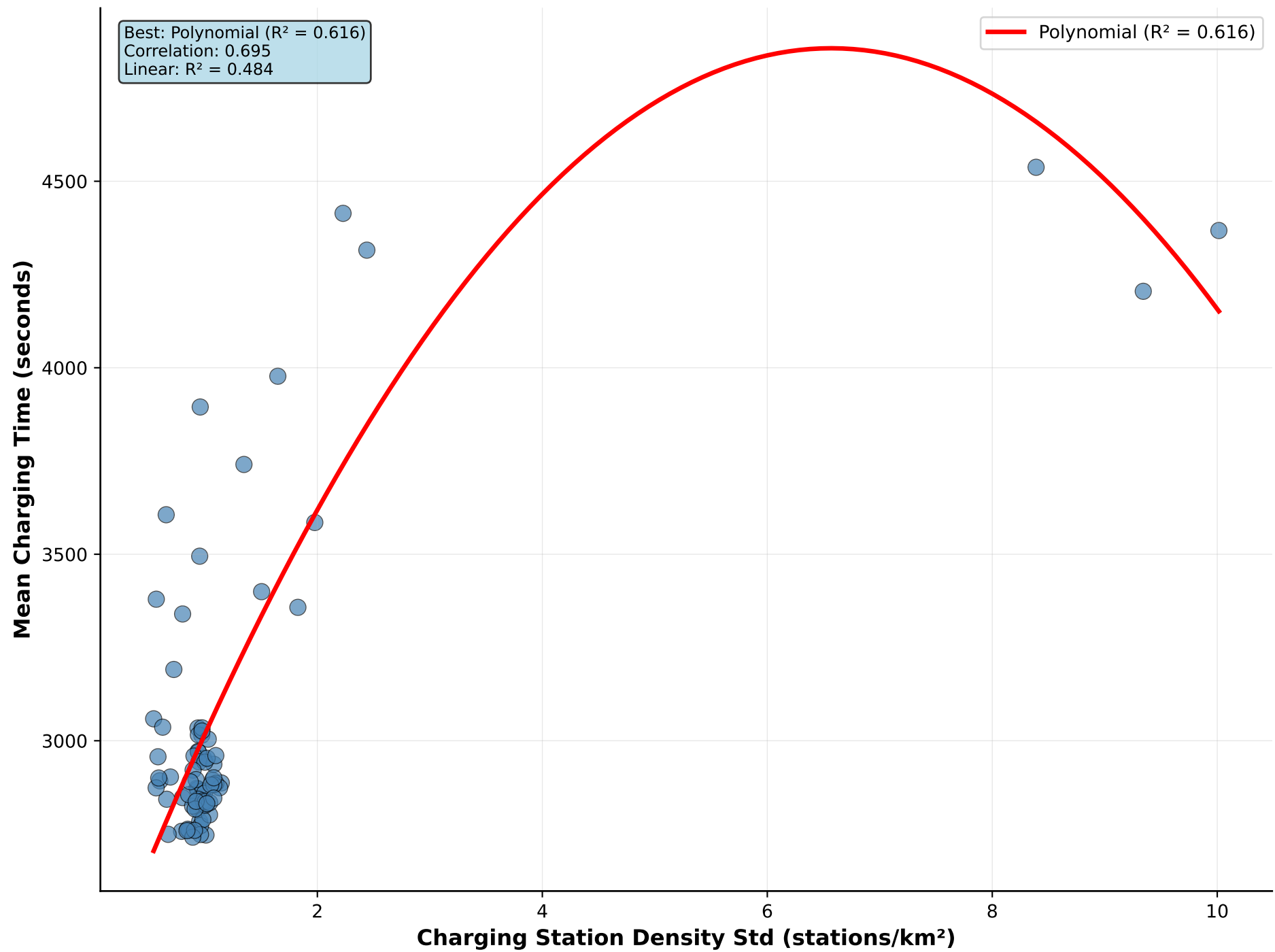
Charging Station Density Std vs Mean Charging Time
