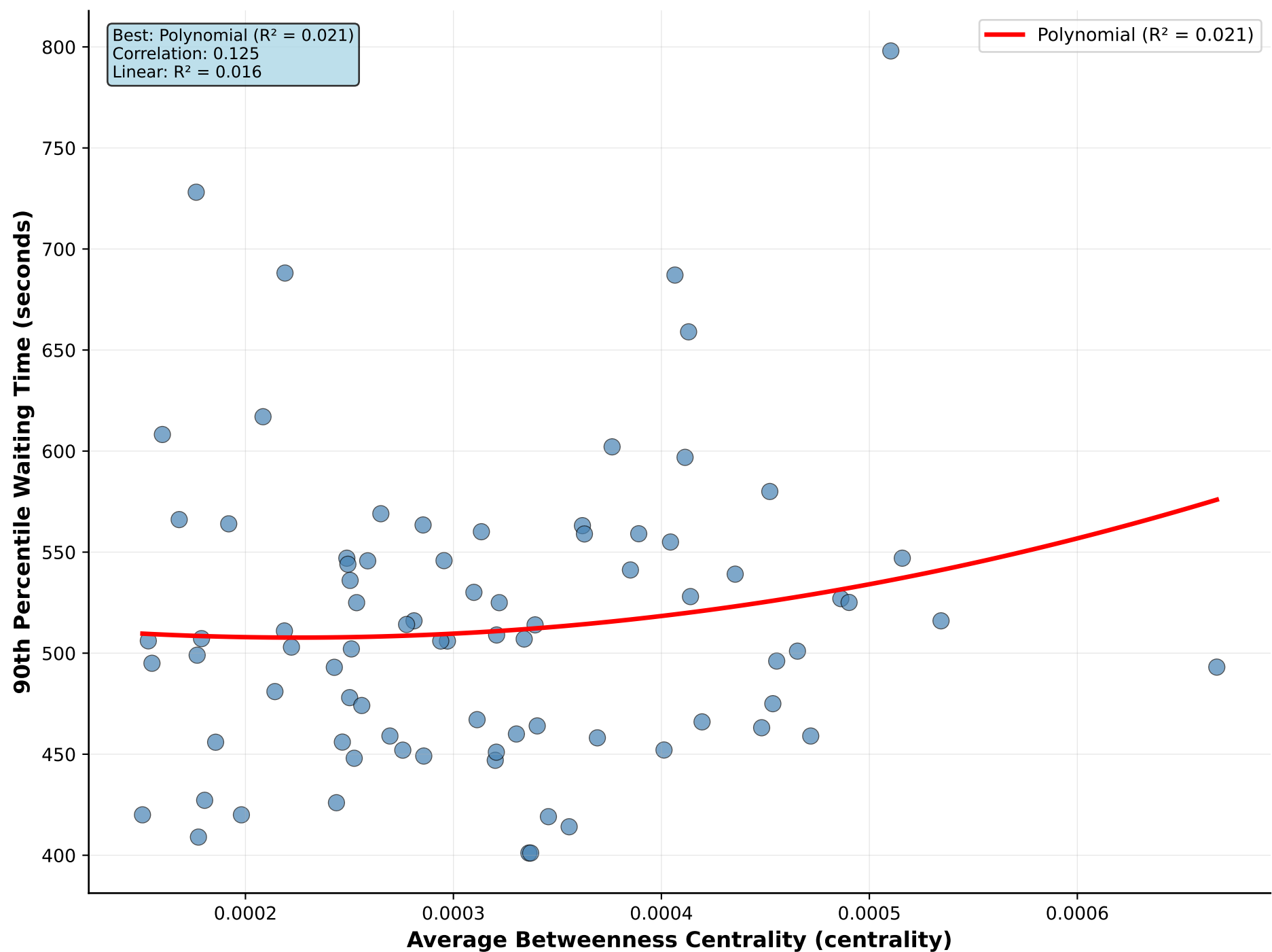
Average Betweenness Centrality vs 90th Percentile Waiting Time
