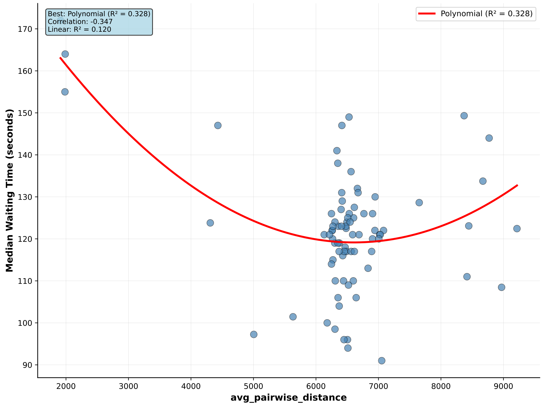
avg_pairwise_distance vs Median Waiting Time
