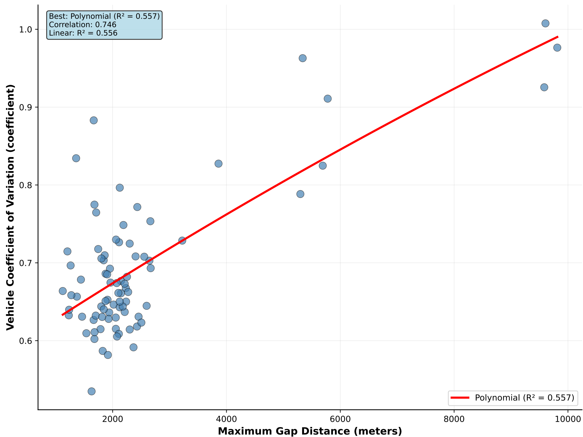
Maximum Gap Distance vs Vehicle Coefficient of Variation
