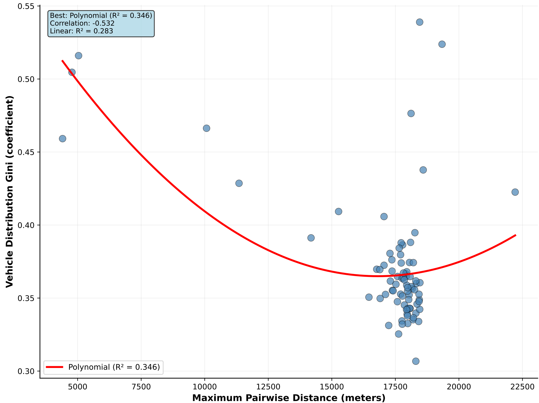
Maximum Pairwise Distance vs Vehicle Distribution Gini
