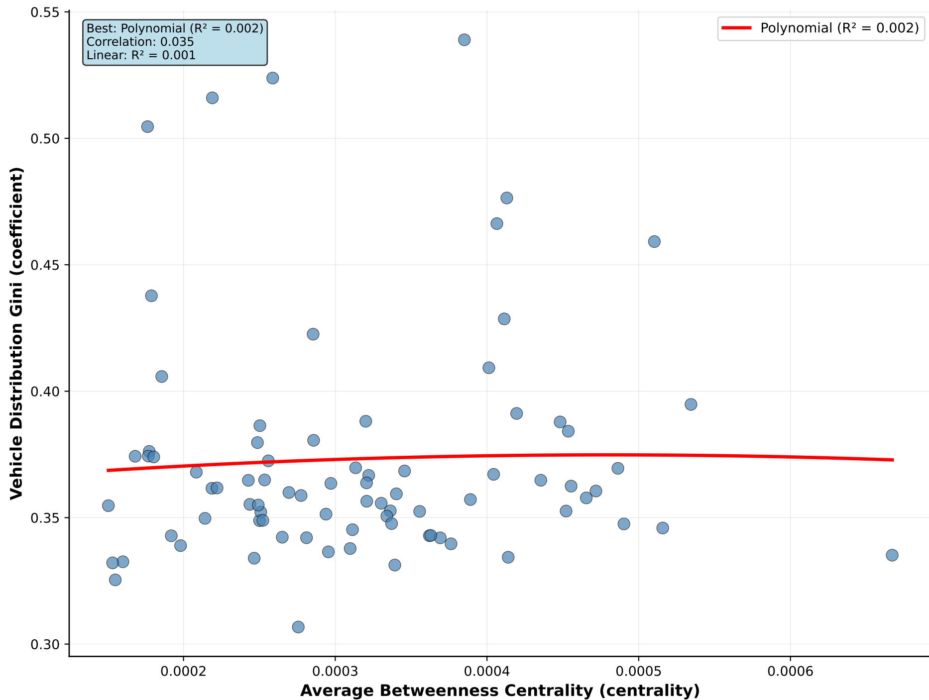
Average Betweenness Centrality vs Vehicle Distribution Gini
