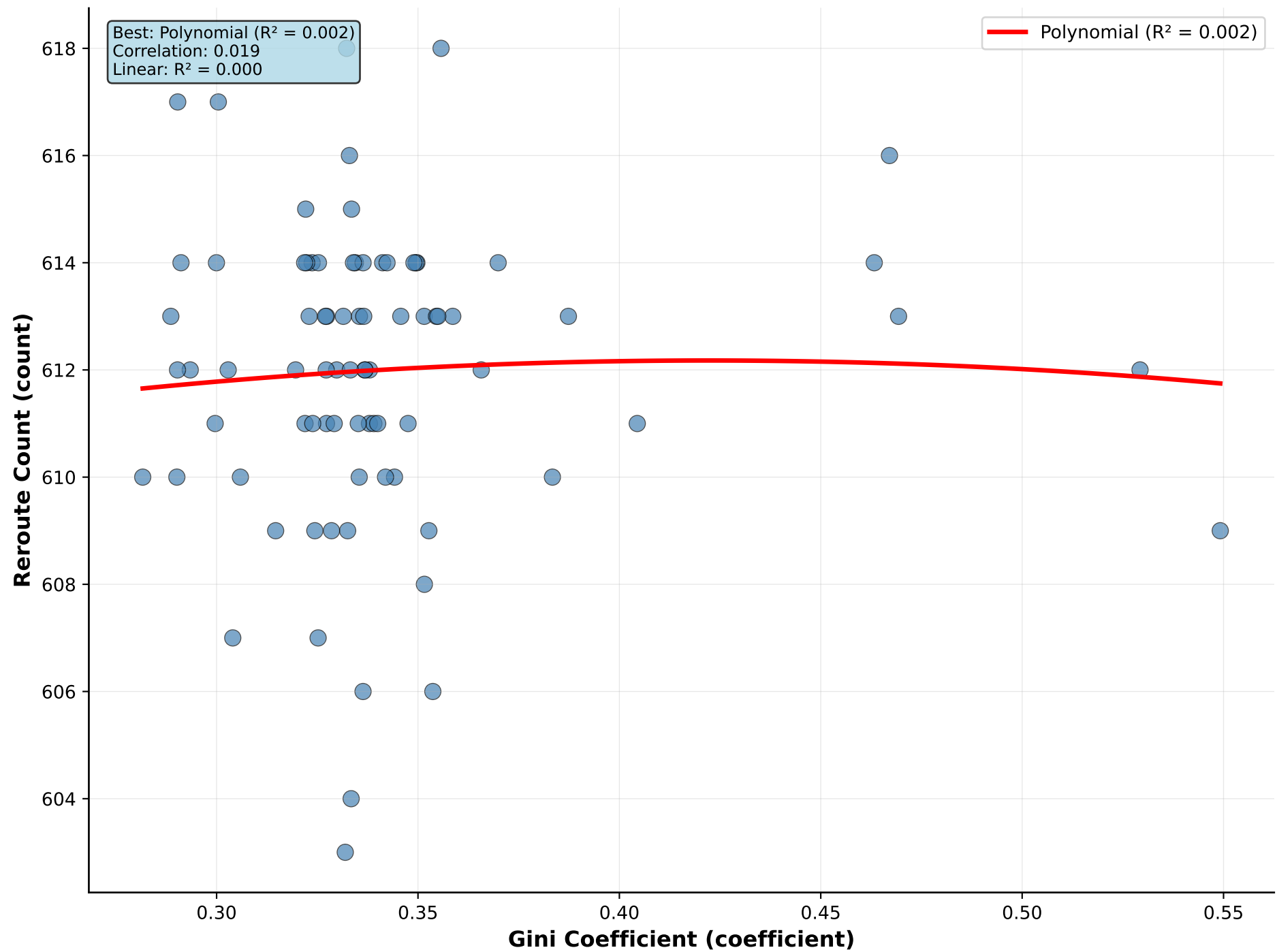
Gini Coefficient vs Reroute Count
