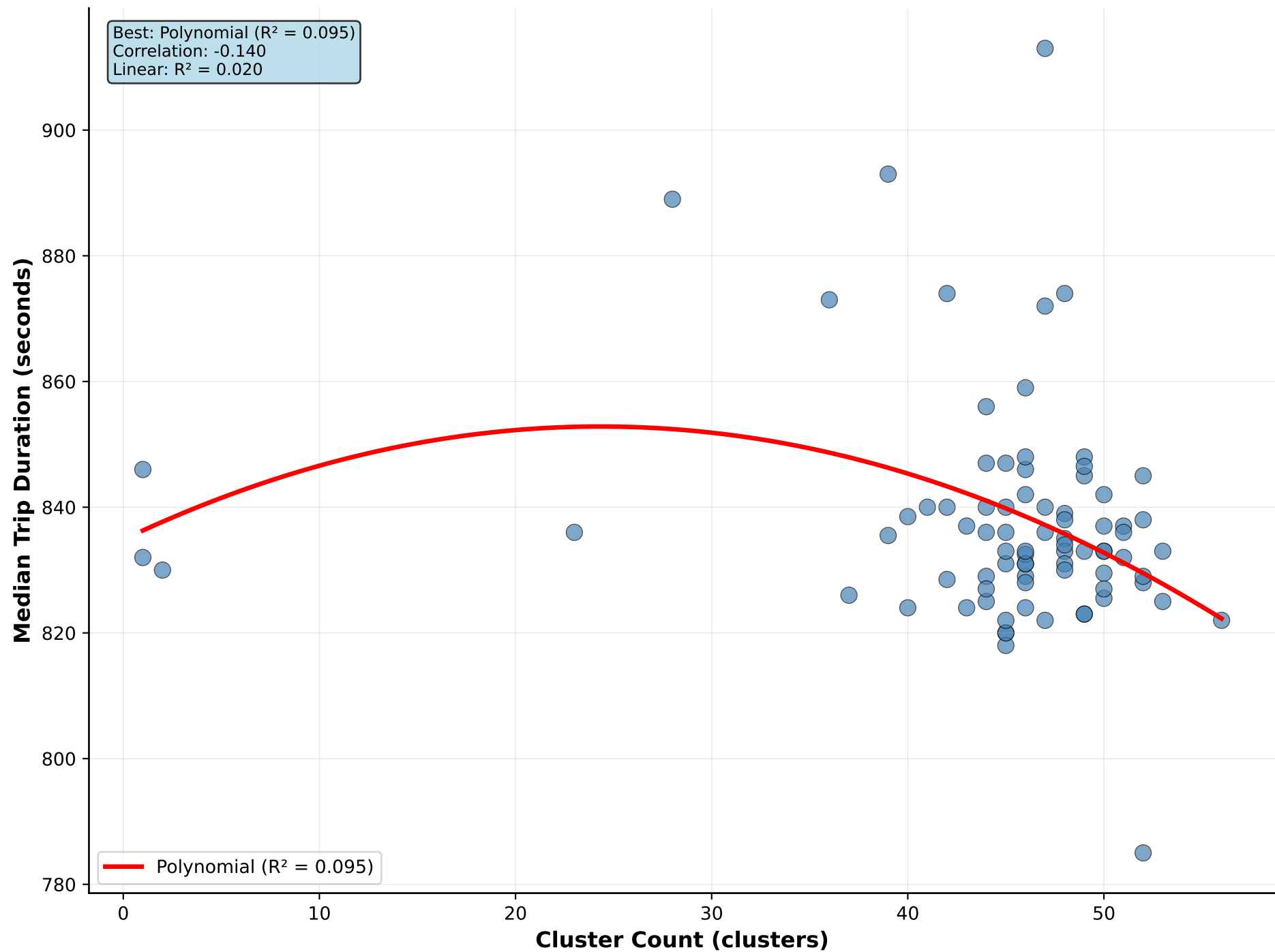
Cluster Count vs Median Trip Duration
