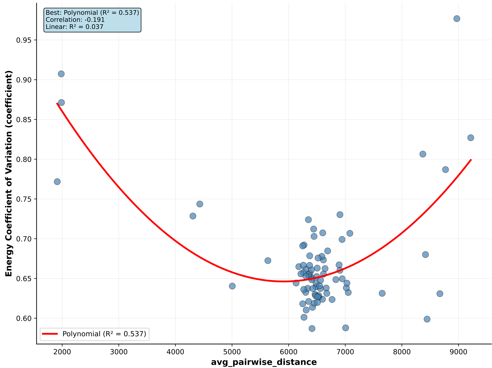
avg_pairwise_distance vs Energy Coefficient of Variation
