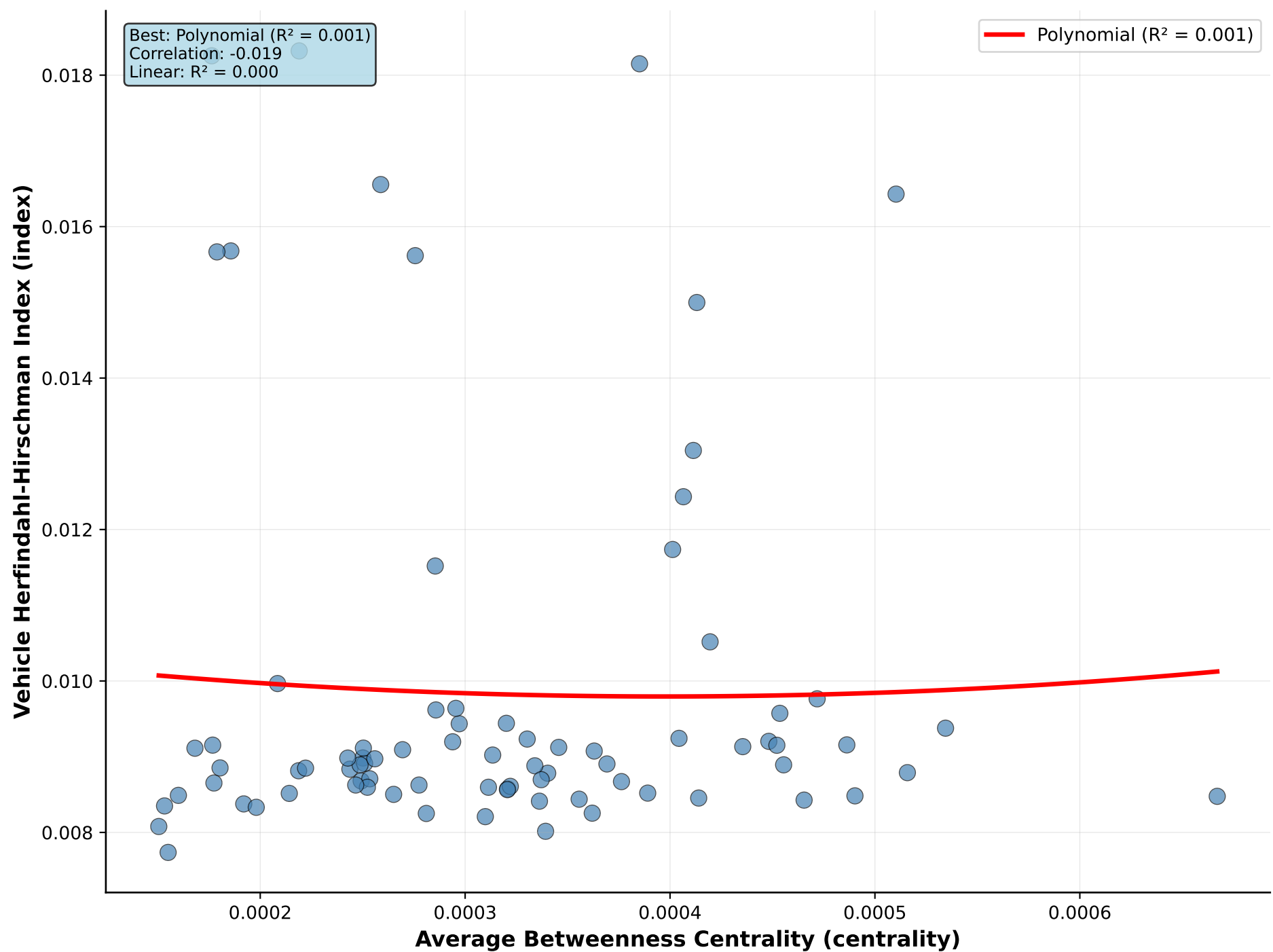
Average Betweenness Centrality vs Vehicle Herfindahl-Hirschman Index
