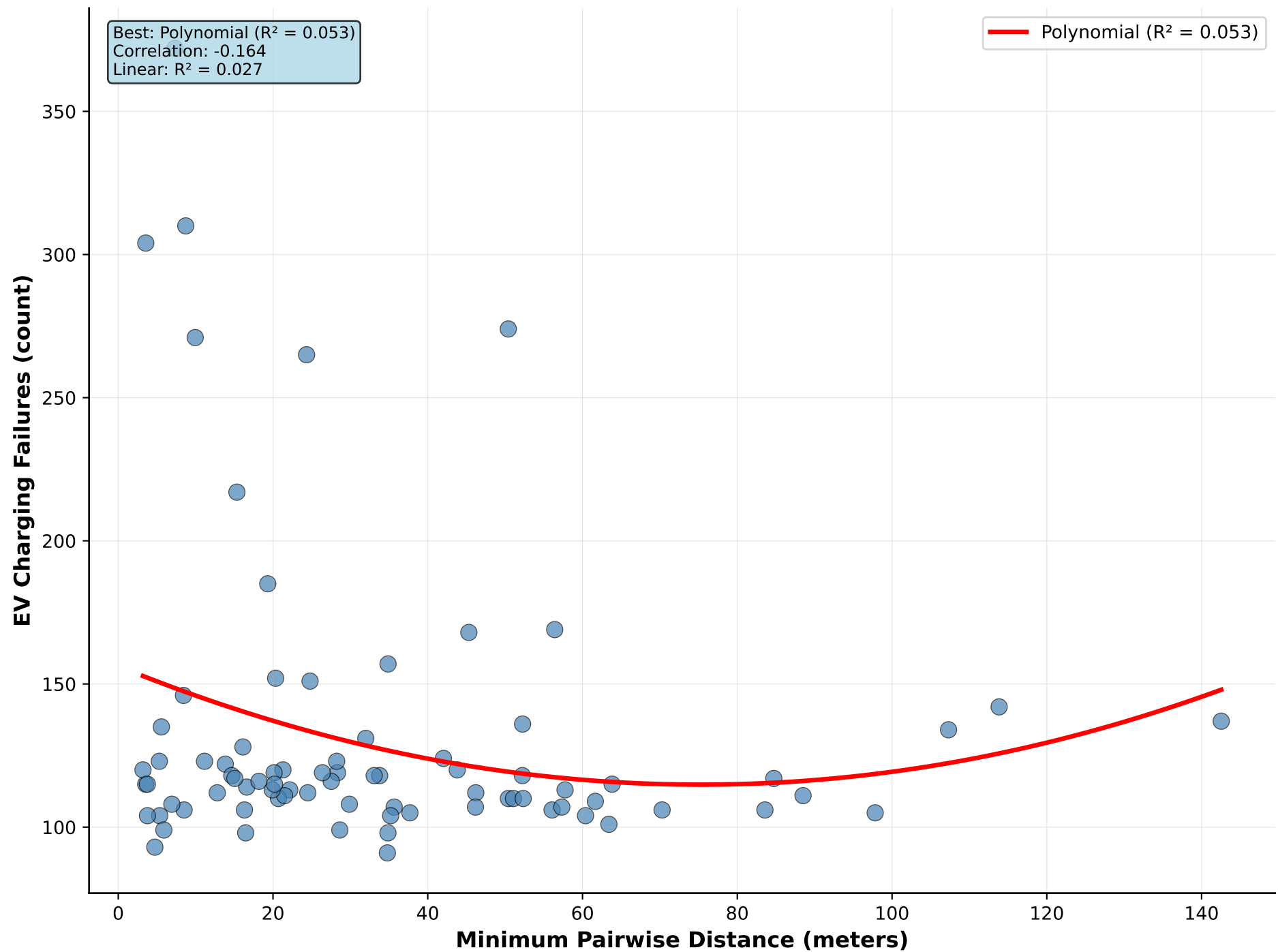
Minimum Pairwise Distance vs EV Charging Failures
