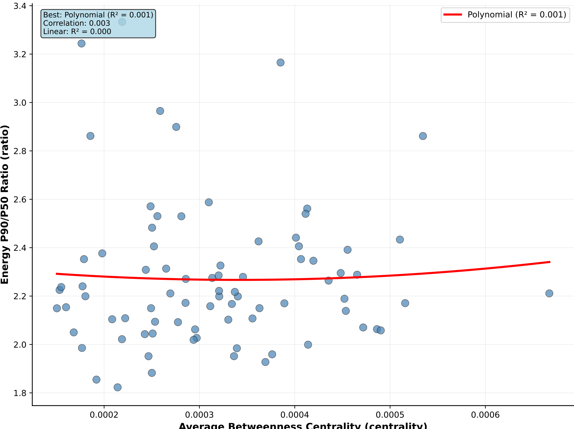
Average Betweenness Centrality vs Energy P90/P50 Ratio
