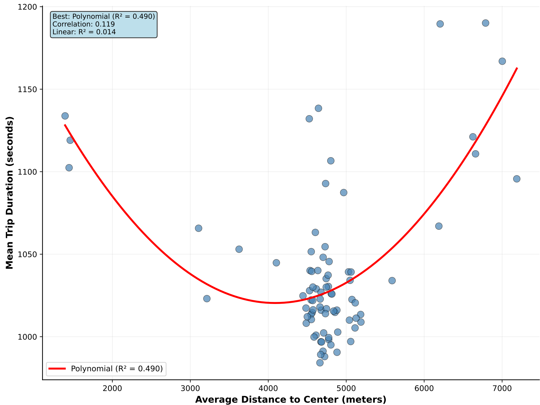
Average Distance to Center vs Mean Trip Duration
