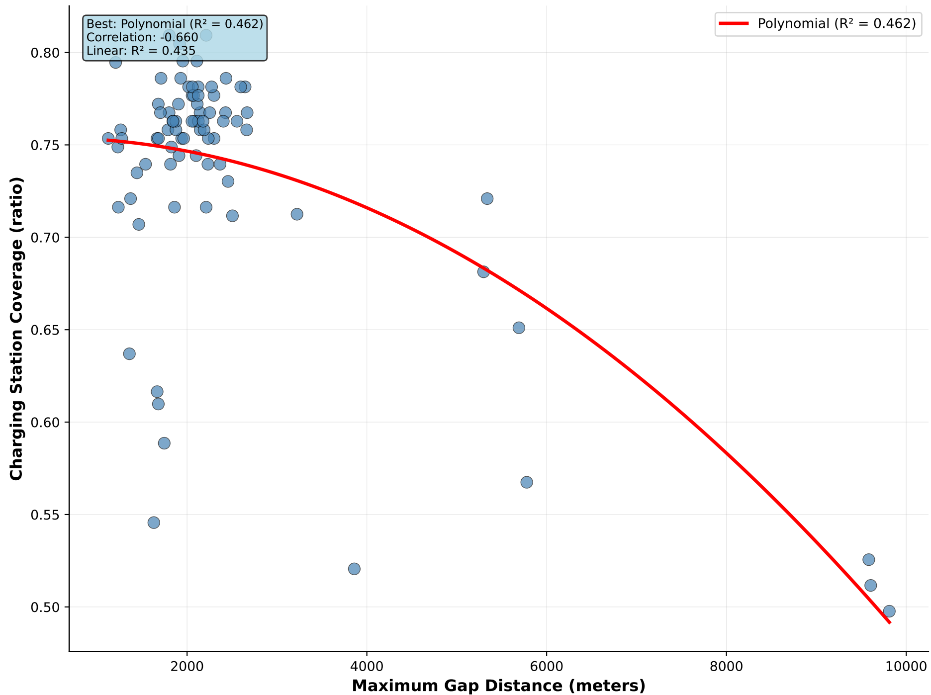
Maximum Gap Distance vs Charging Station Coverage
