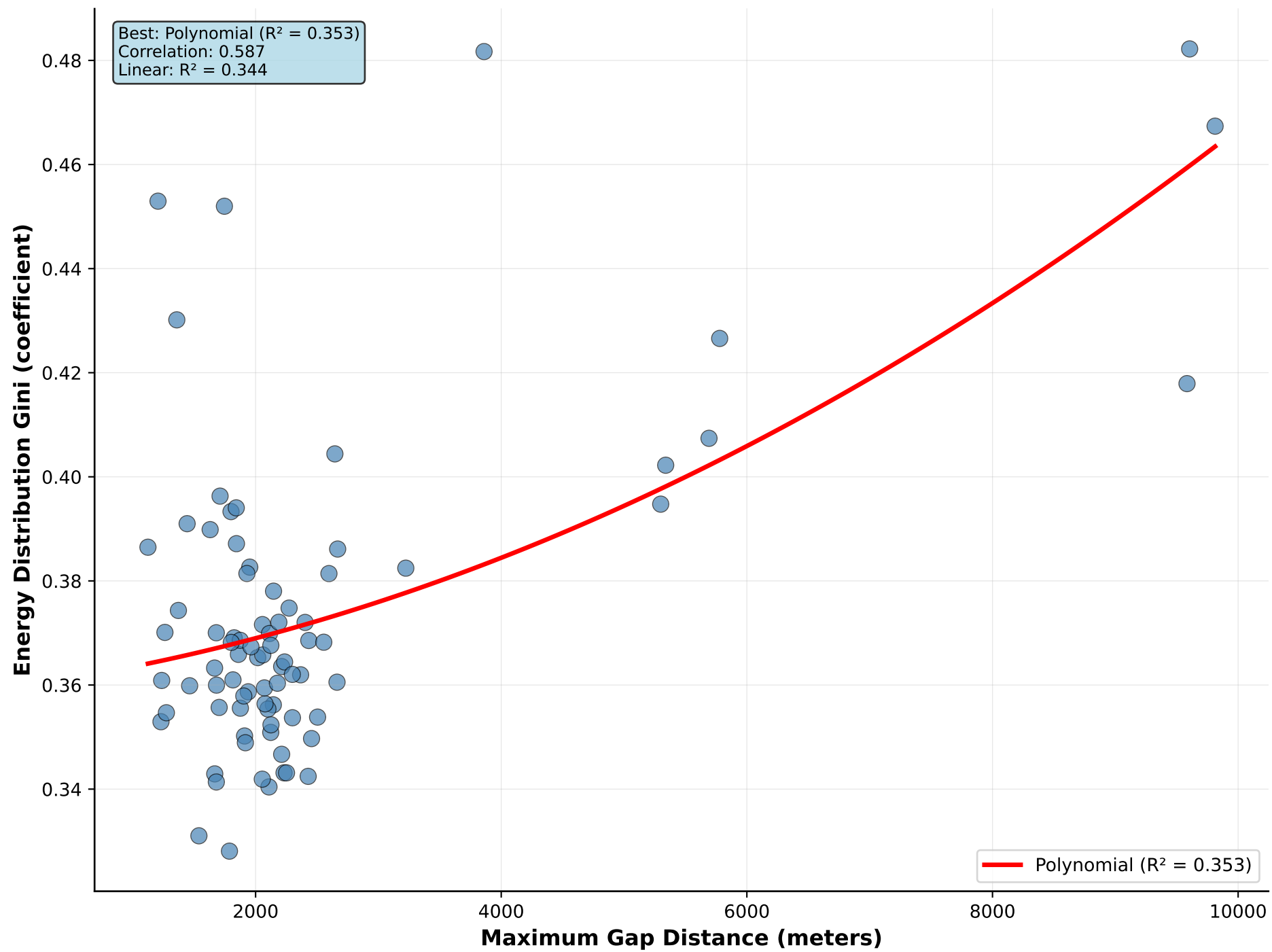
Maximum Gap Distance vs Energy Distribution Gini
