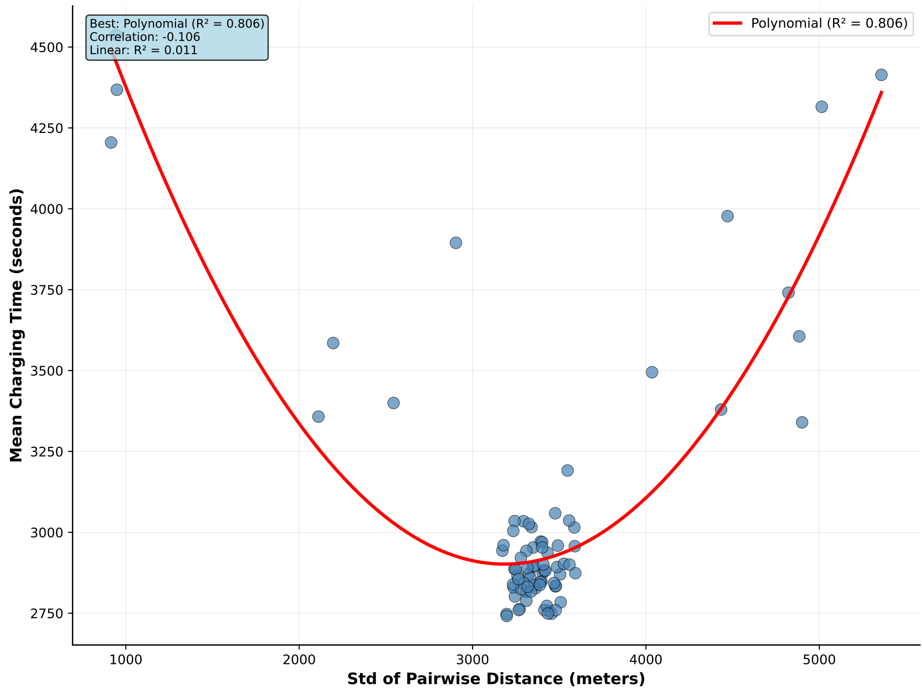
Std of Pairwise Distance vs Mean Charging Time
