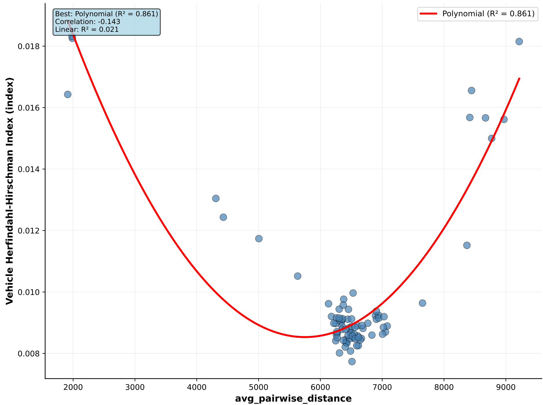
avg_pairwise_distance vs Vehicle Herfindahl-Hirschman Index
