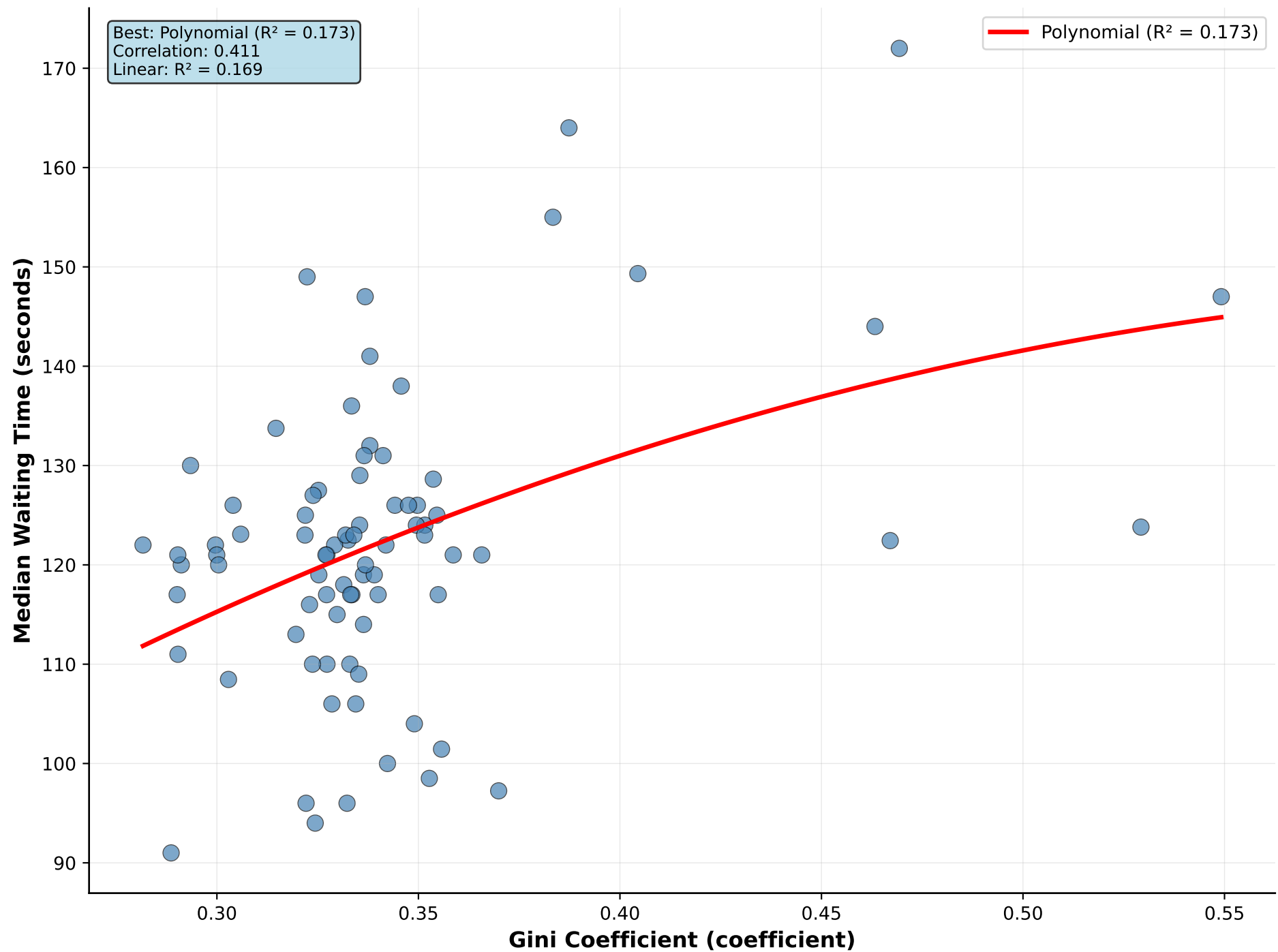
Gini Coefficient vs Median Waiting Time
