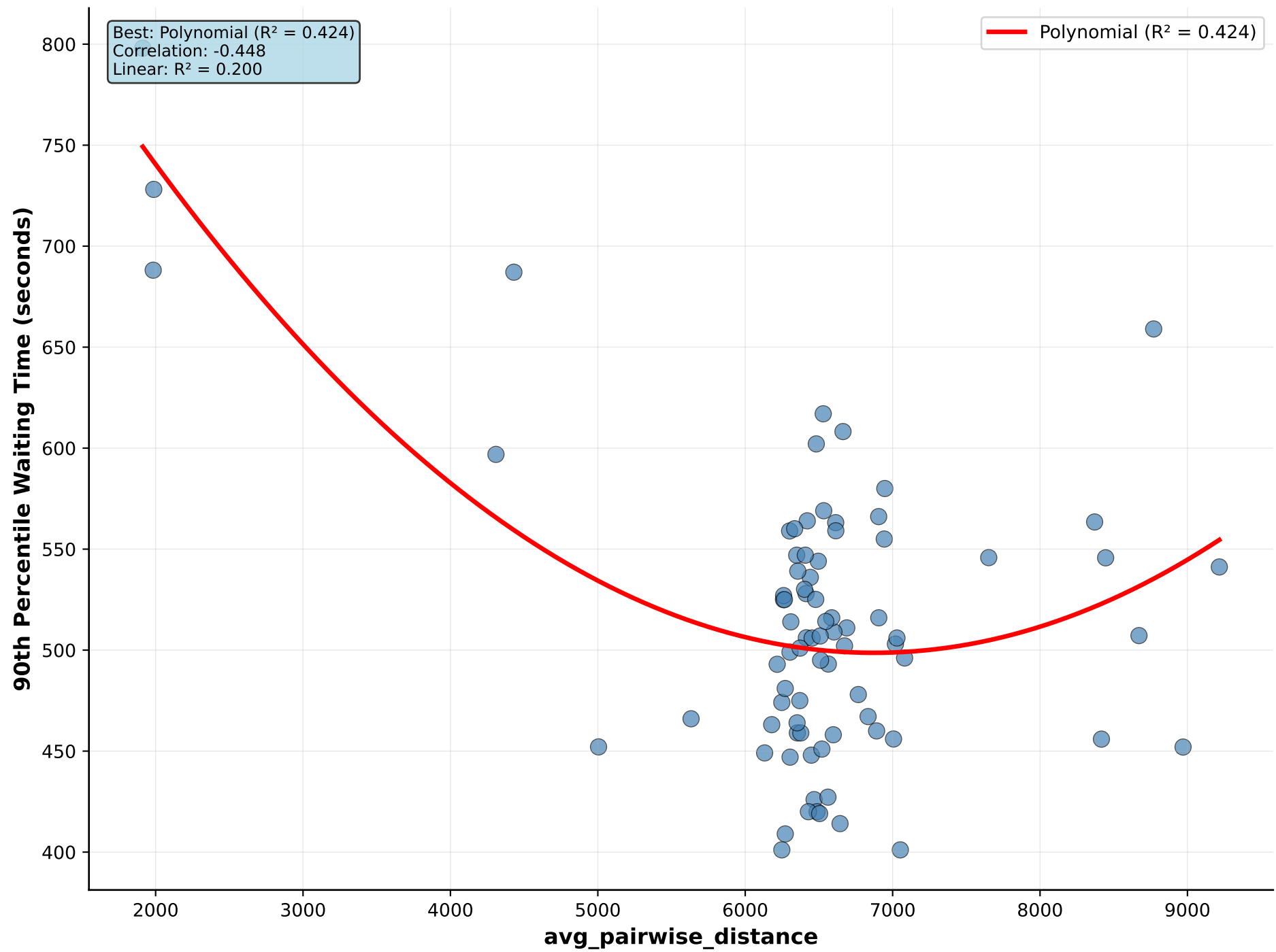
avg_pairwise_distance vs 90th Percentile Waiting Time
