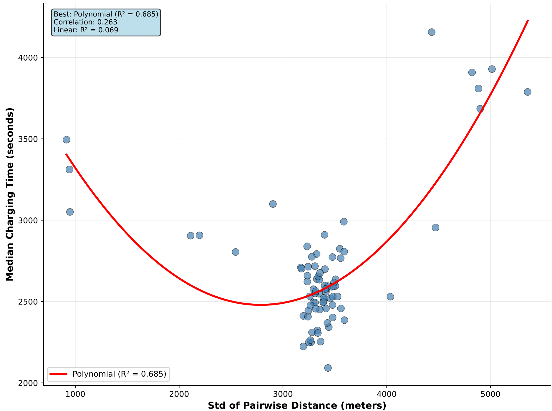
Std of Pairwise Distance vs Median Charging Time
