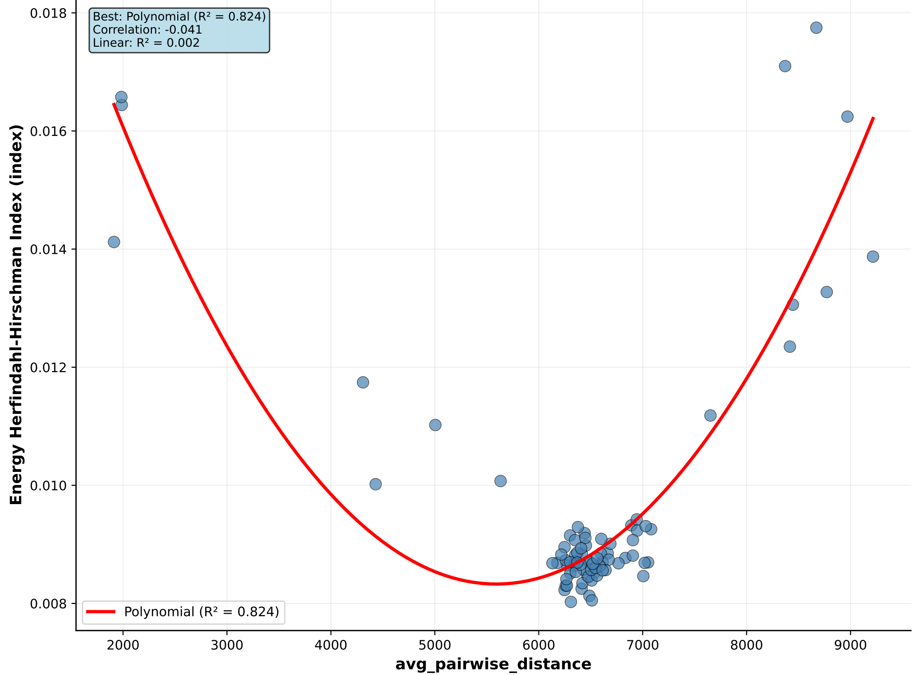
avg_pairwise_distance vs Energy Herfindahl-Hirschman Index
