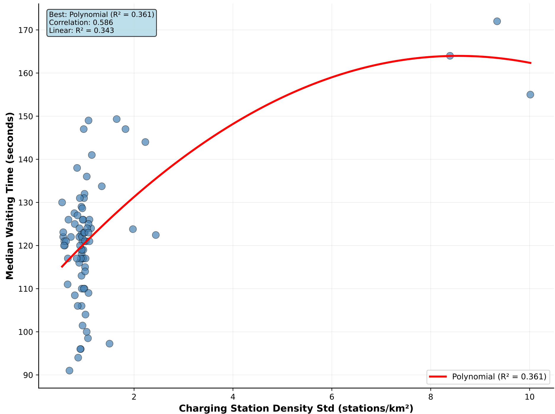
Charging Station Density Std vs Median Waiting Time
