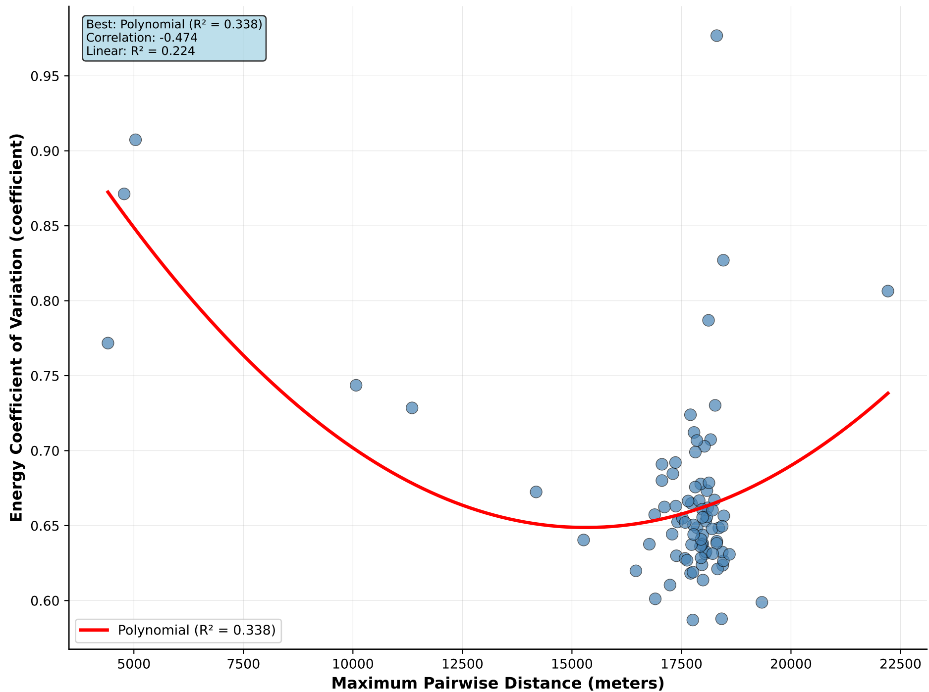
Maximum Pairwise Distance vs Energy Coefficient of Variation
