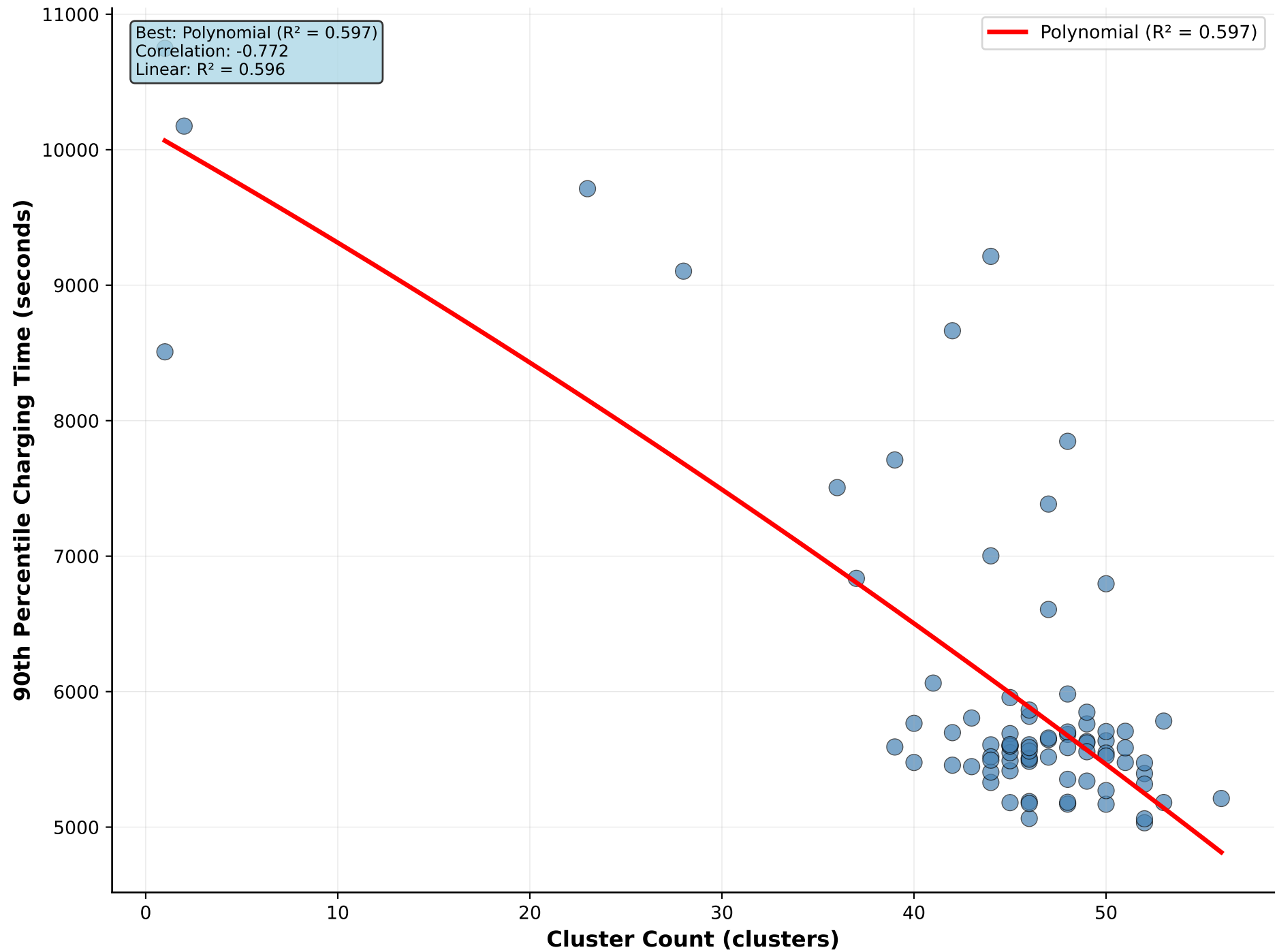
Cluster Count vs 90th Percentile Charging Time
