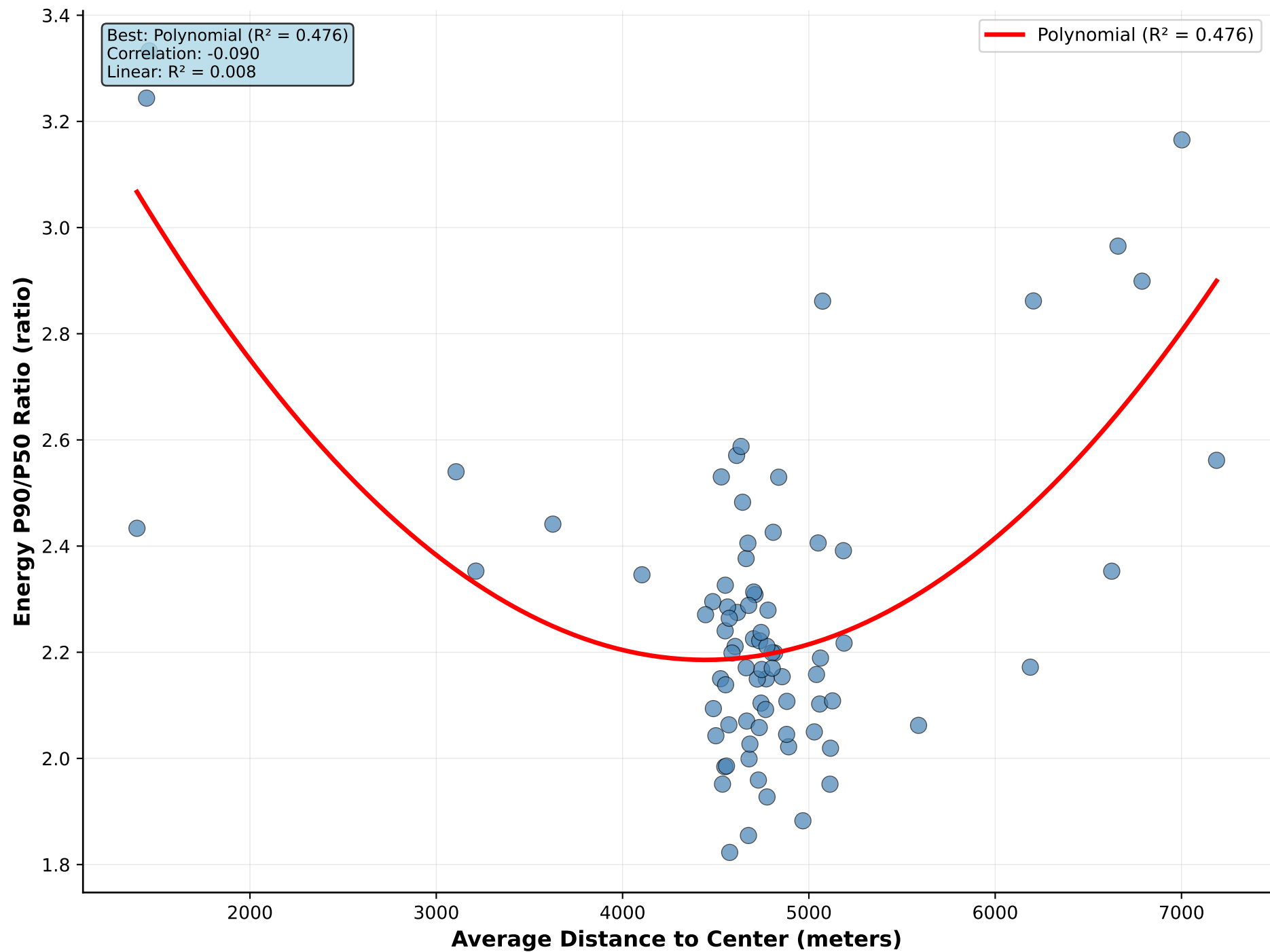
Average Distance to Center vs Energy P90/P50 Ratio
