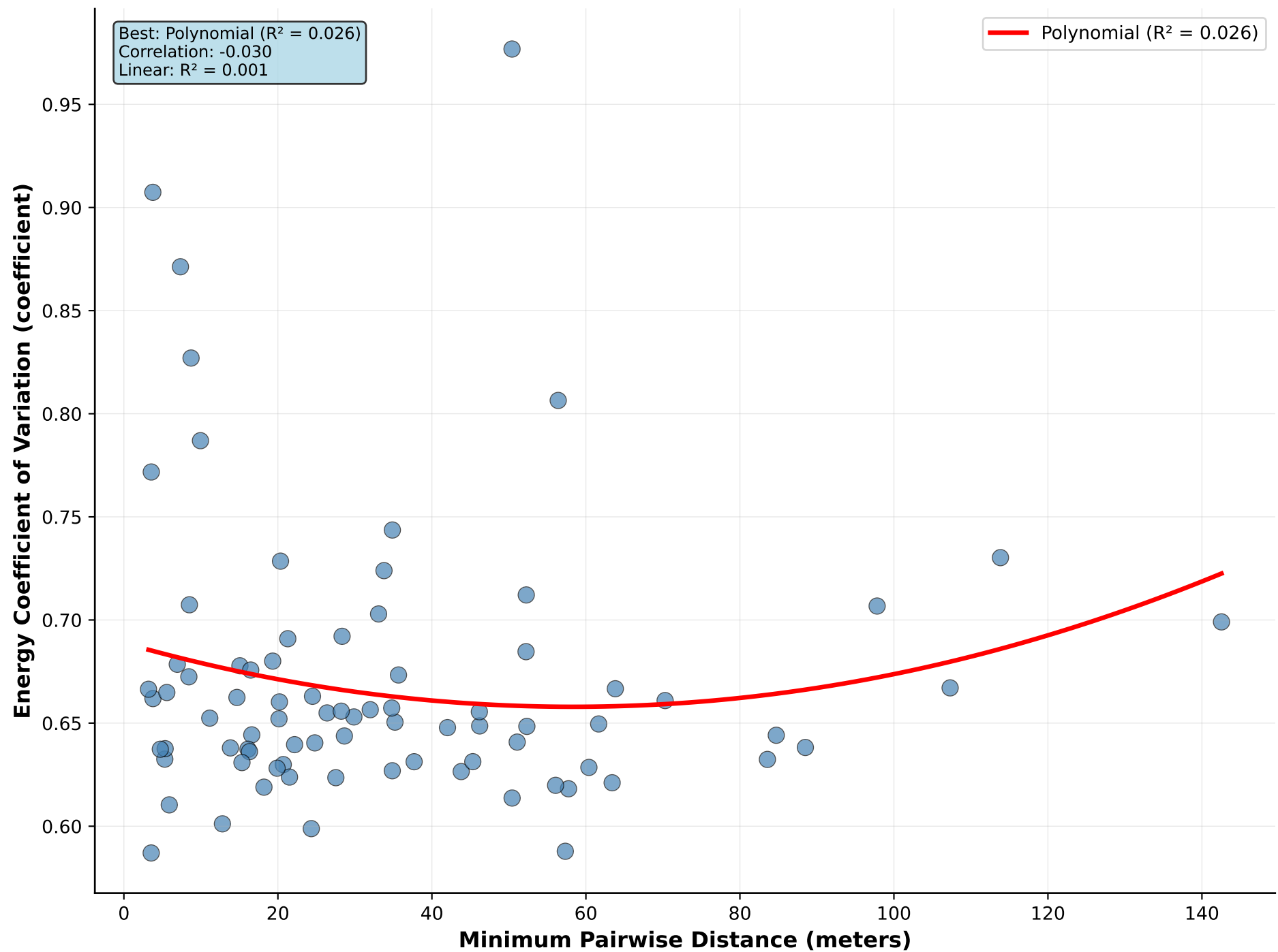
Minimum Pairwise Distance vs Energy Coefficient of Variation
