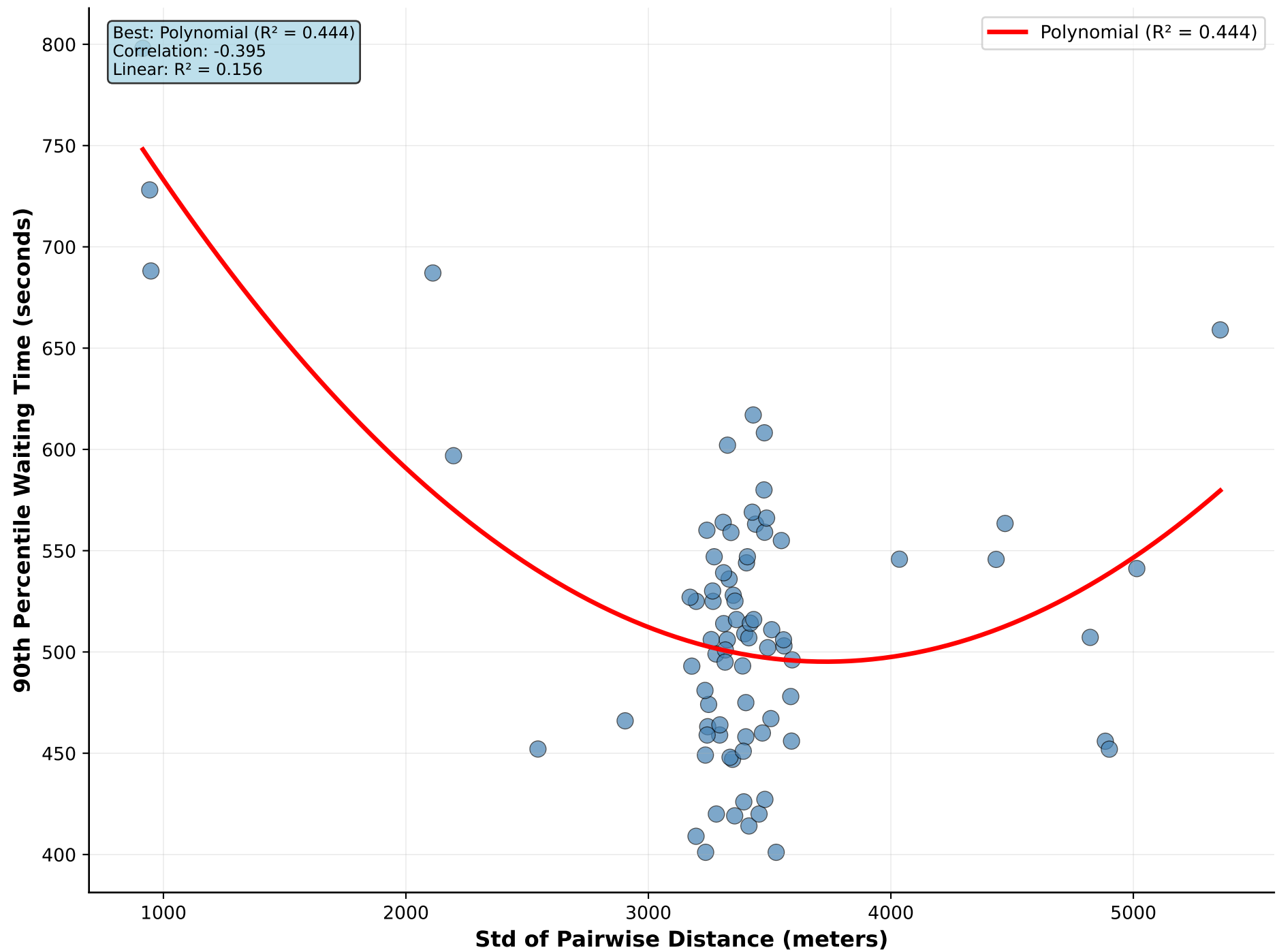
Std of Pairwise Distance vs 90th Percentile Waiting Time
