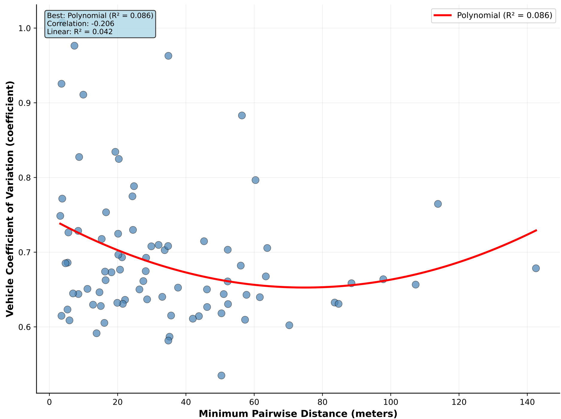
Minimum Pairwise Distance vs Vehicle Coefficient of Variation
