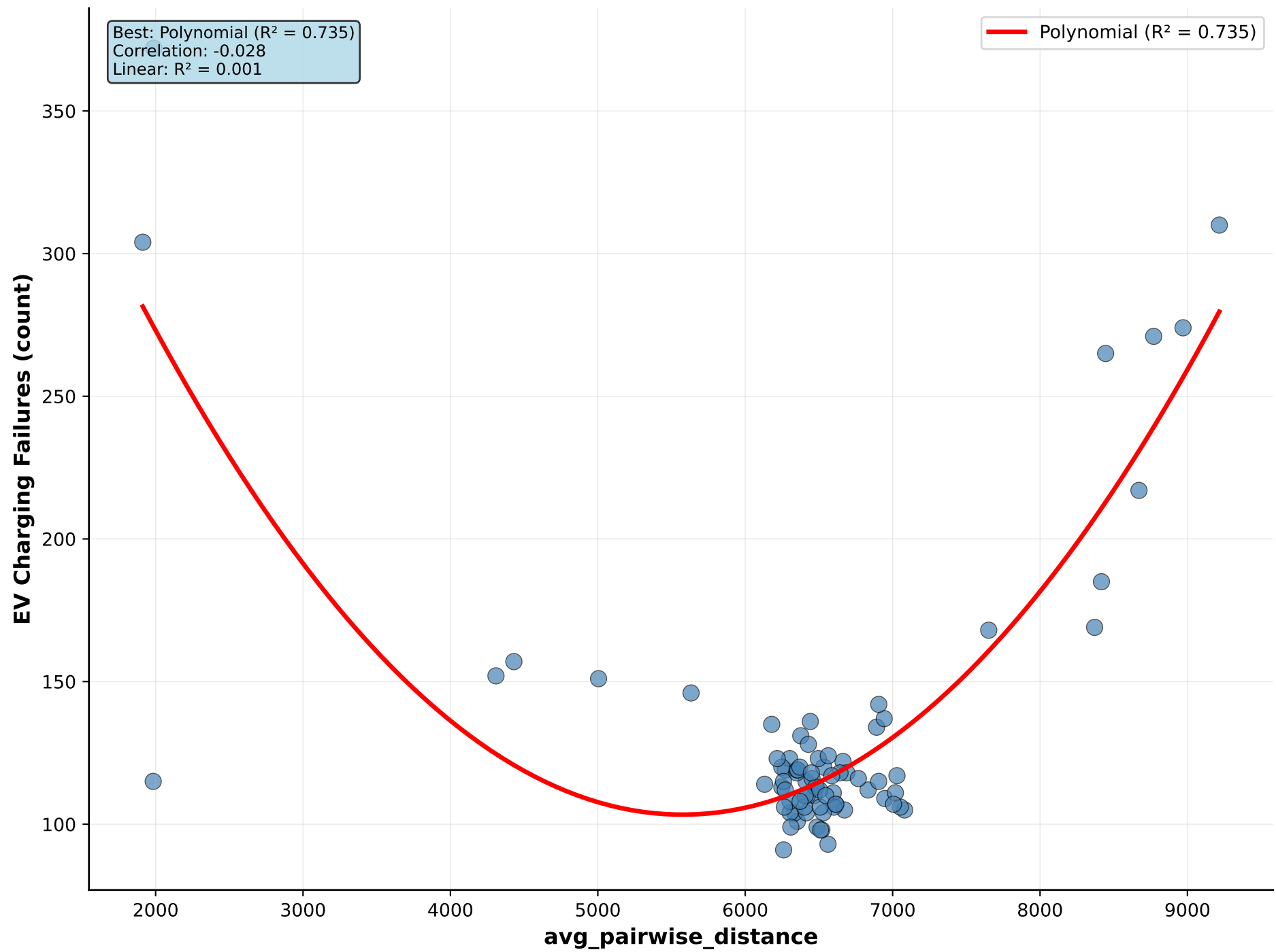
avg_pairwise_distance vs EV Charging Failures
