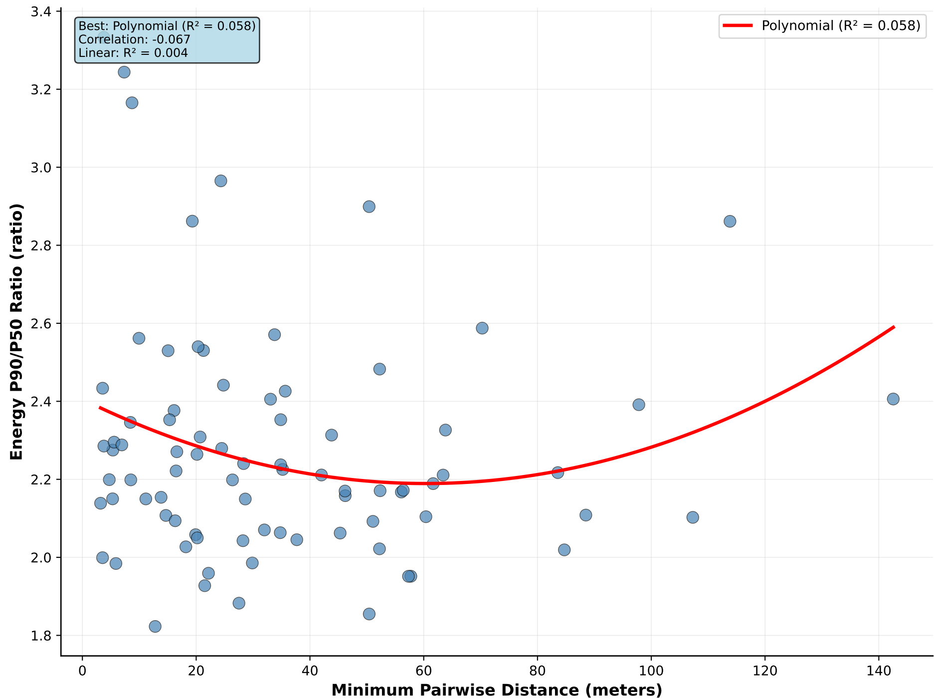
Minimum Pairwise Distance vs Energy P90/P50 Ratio
