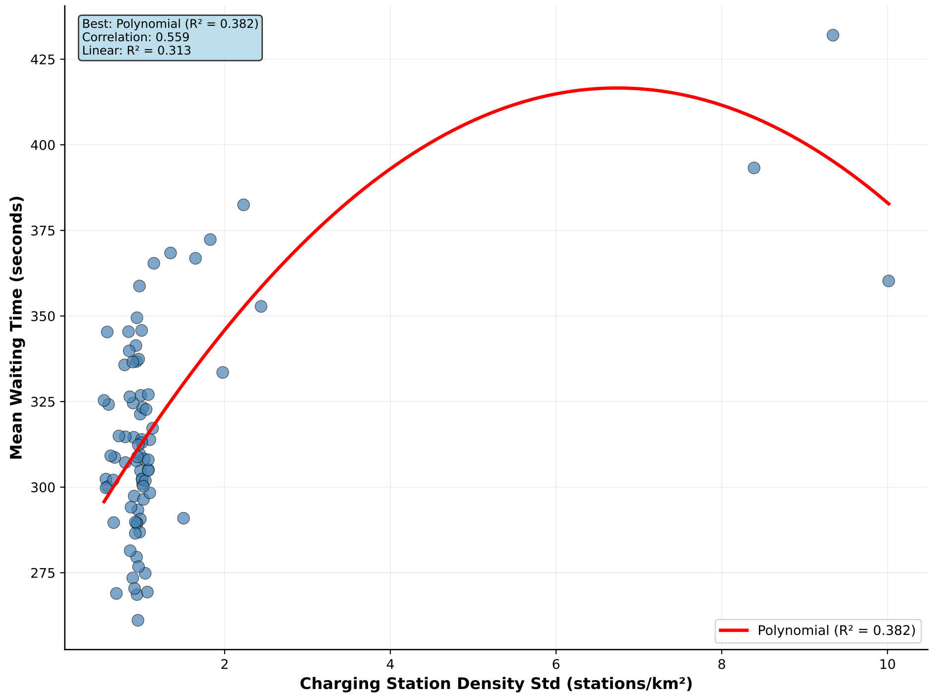
Charging Station Density Std vs Mean Waiting Time
