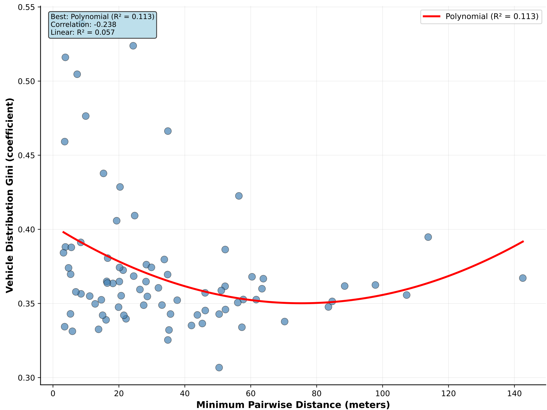
Minimum Pairwise Distance vs Vehicle Distribution Gini
