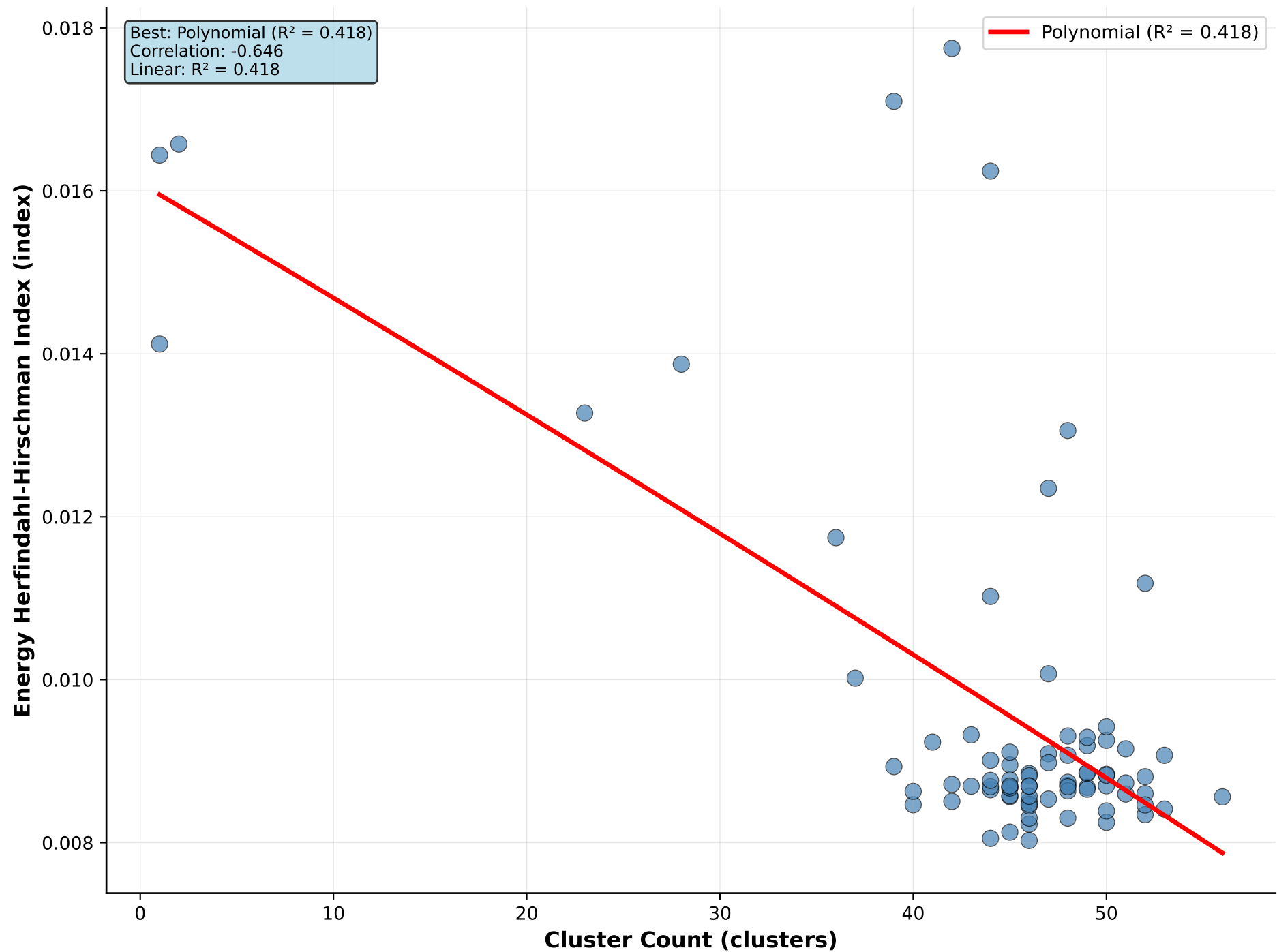
Cluster Count vs Energy Herfindahl-Hirschman Index
