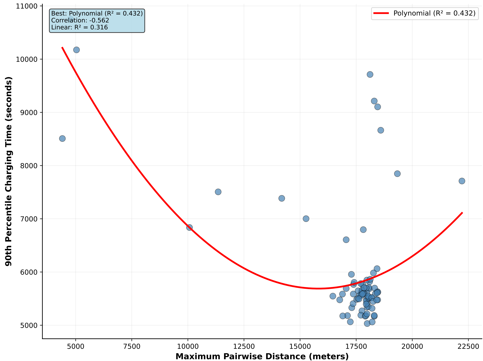
Maximum Pairwise Distance vs 90th Percentile Charging Time
