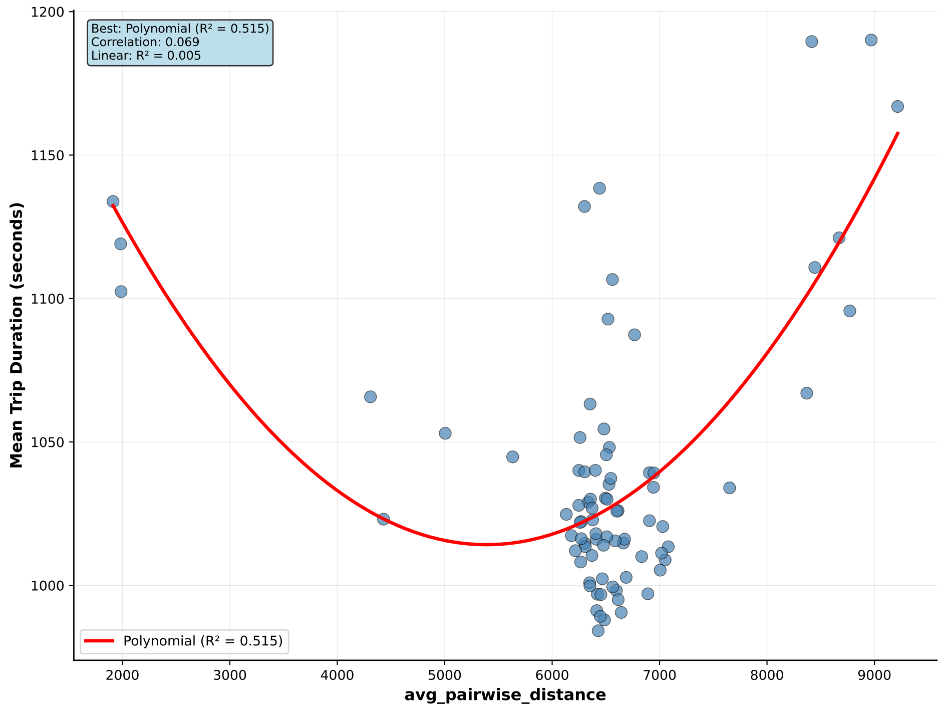
avg_pairwise_distance vs Mean Trip Duration
