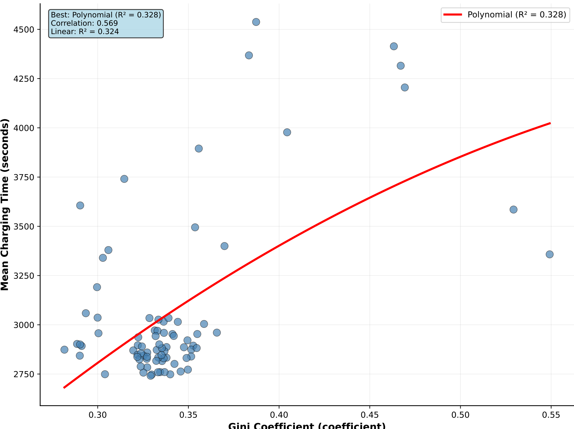
Gini Coefficient vs Mean Charging Time
