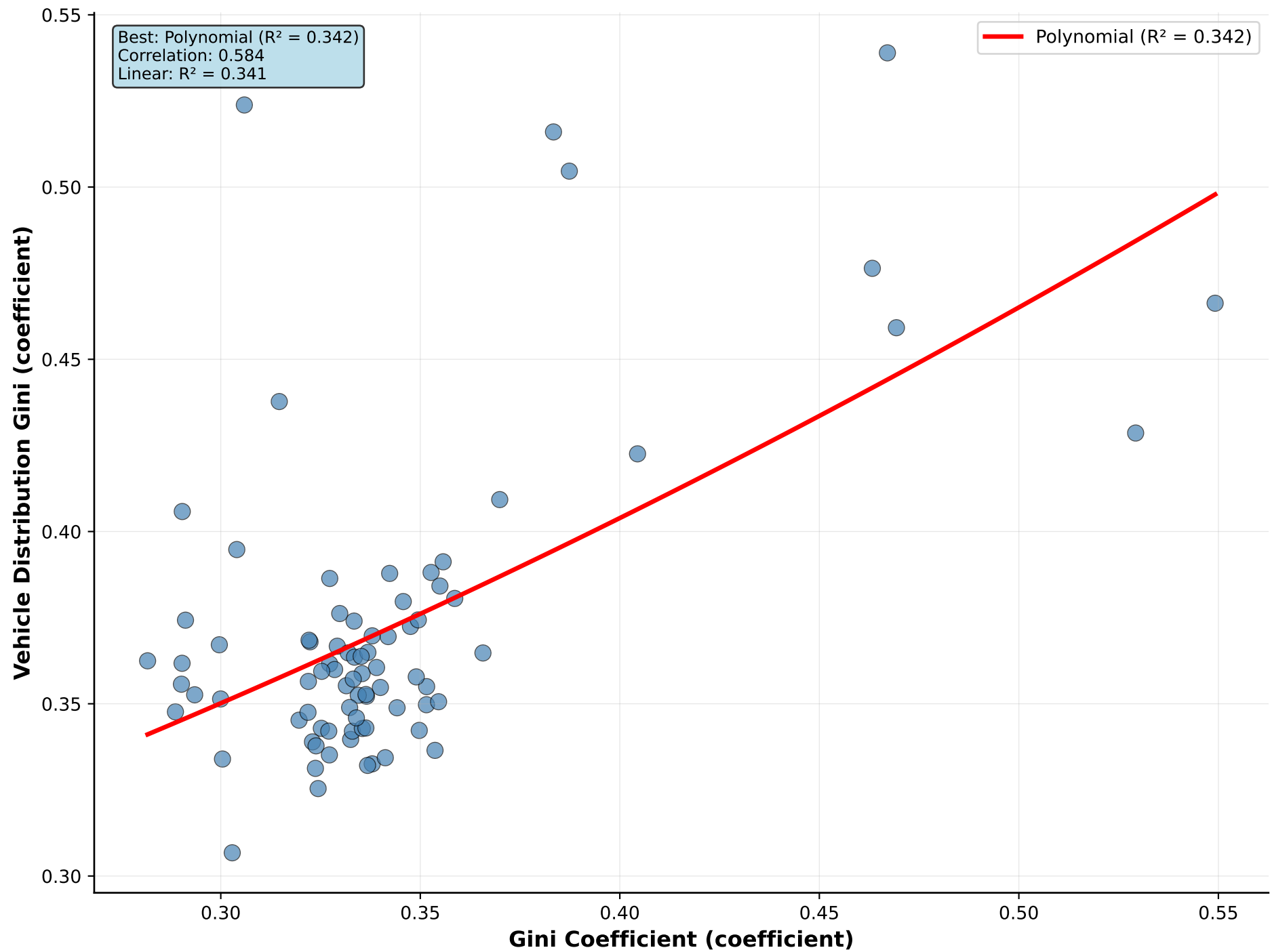
Gini Coefficient vs Vehicle Distribution Gini
