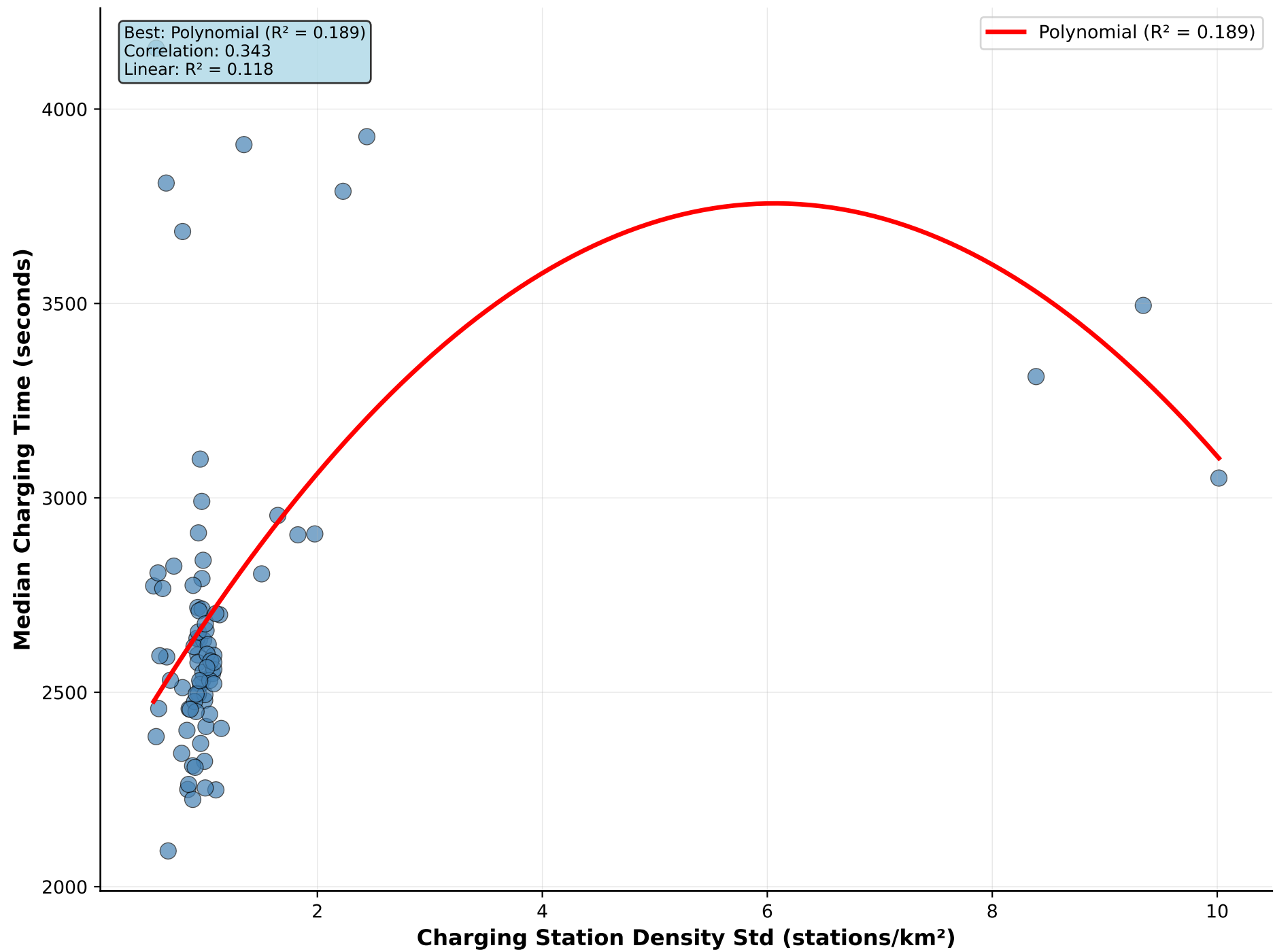
Charging Station Density Std vs Median Charging Time
