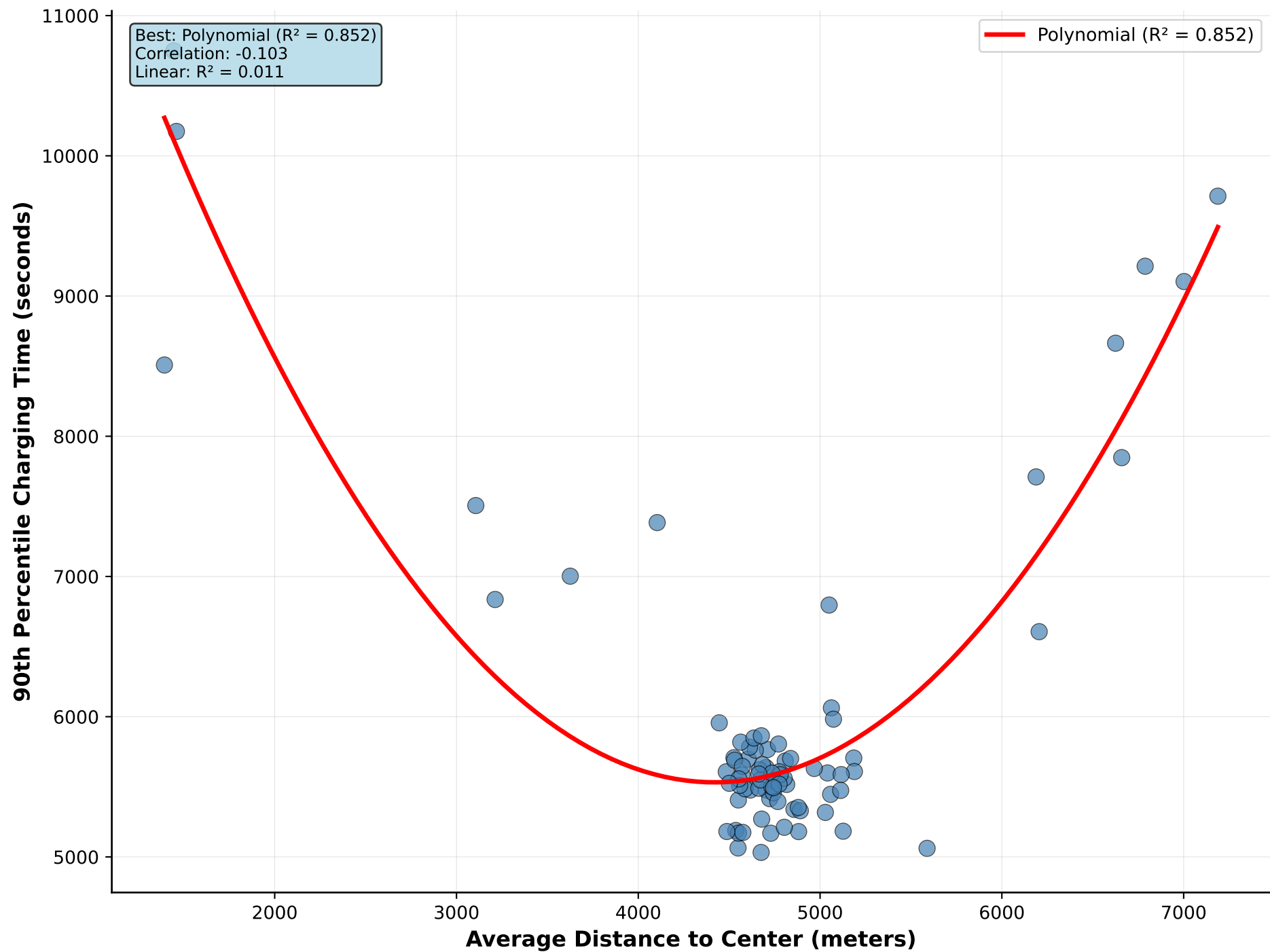
Average Distance to Center vs 90th Percentile Charging Time
