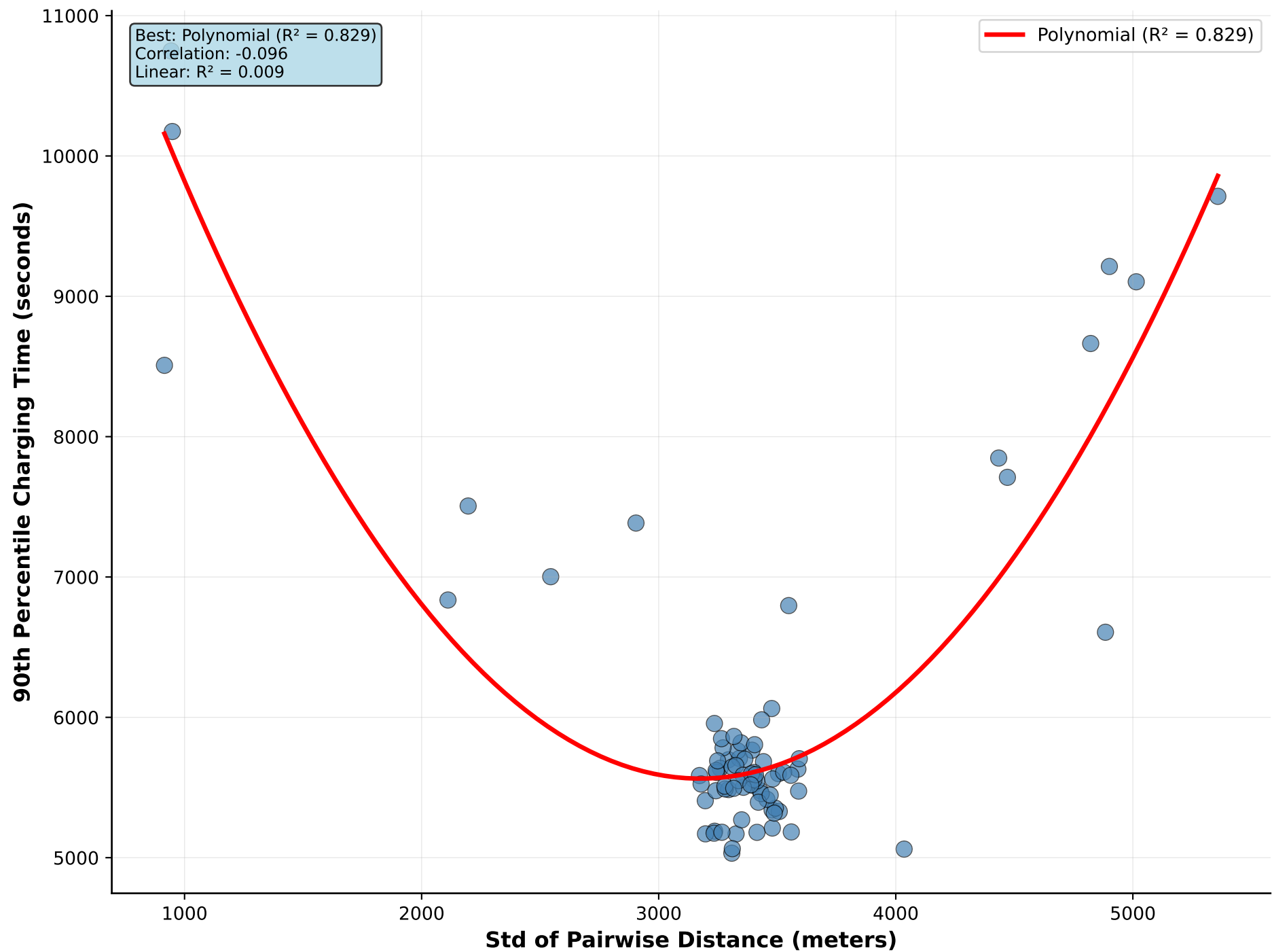
Std of Pairwise Distance vs 90th Percentile Charging Time
