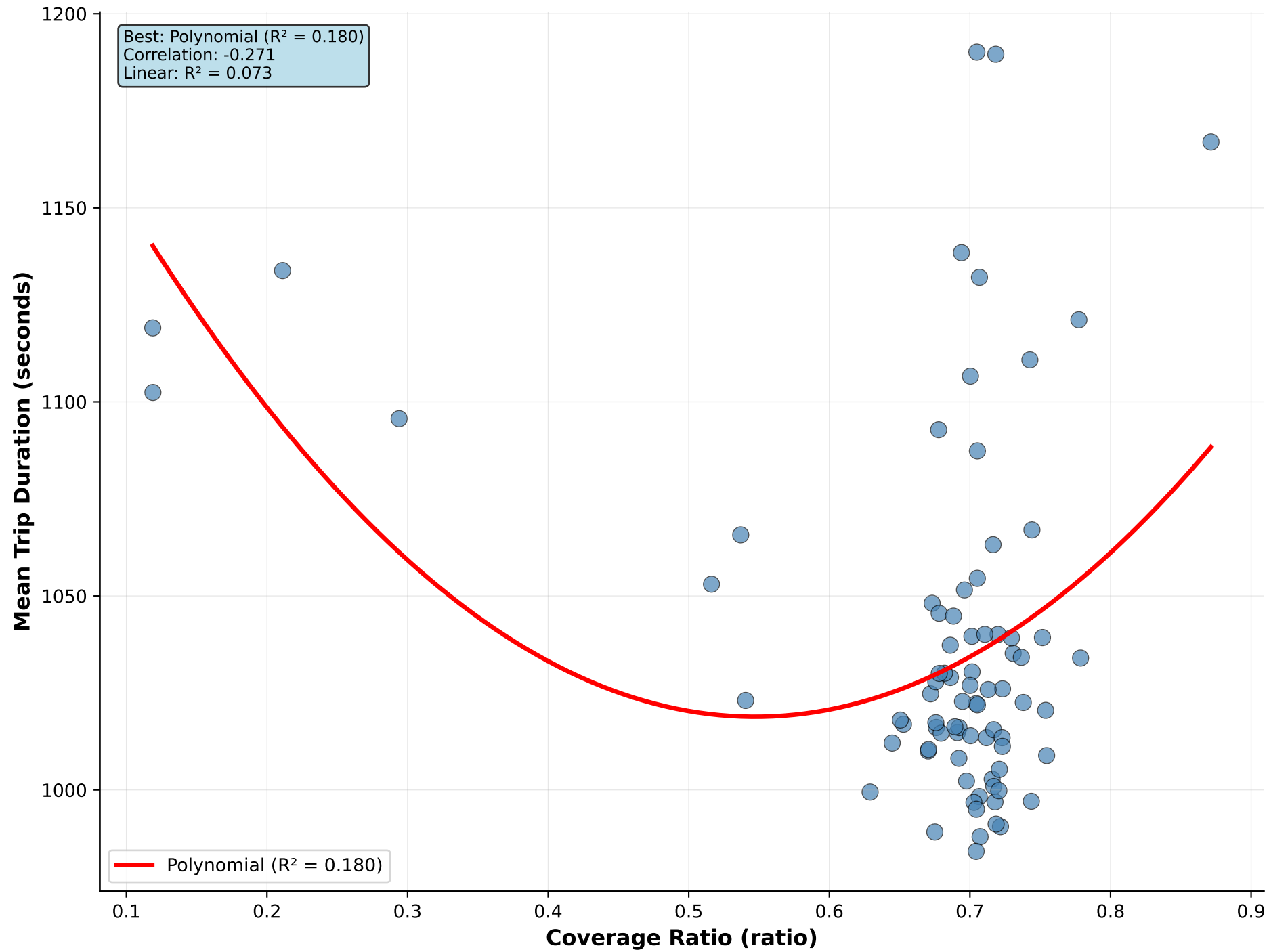
Coverage Ratio vs Mean Trip Duration
