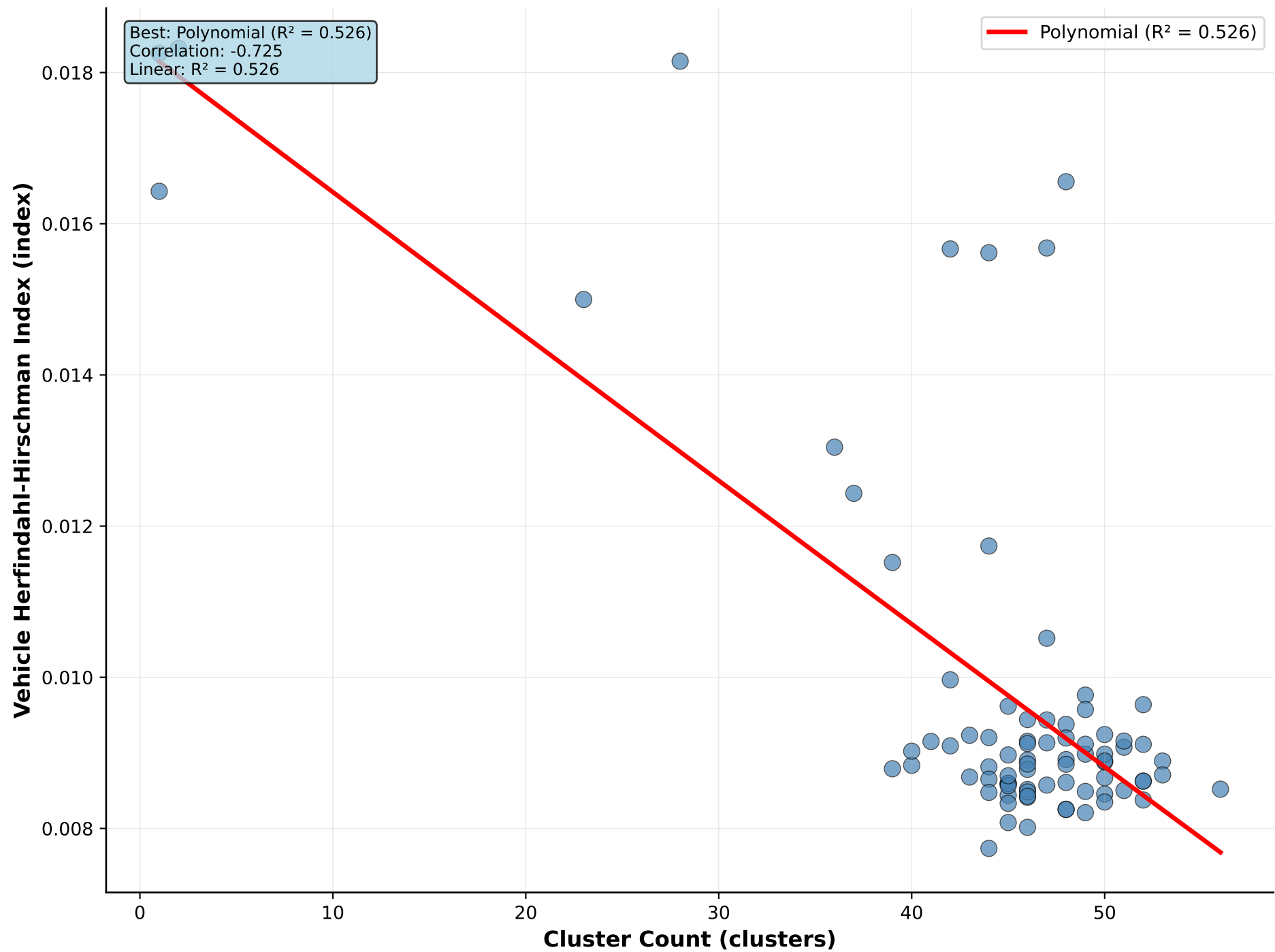
Cluster Count vs Vehicle Herfindahl-Hirschman Index
