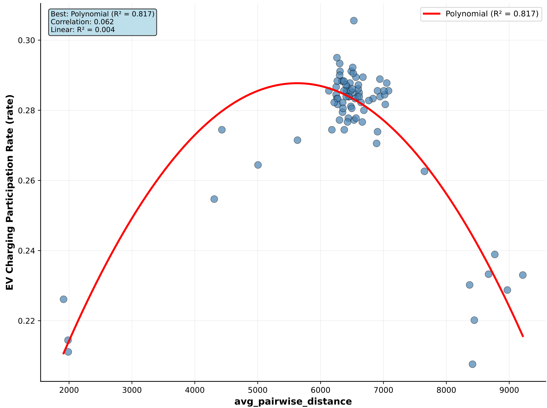
avg_pairwise_distance vs EV Charging Participation Rate
