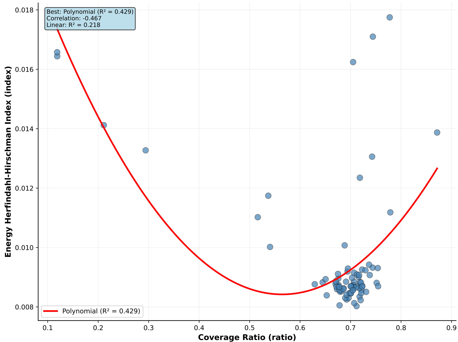
Coverage Ratio vs Energy Herfindahl-Hirschman Index
