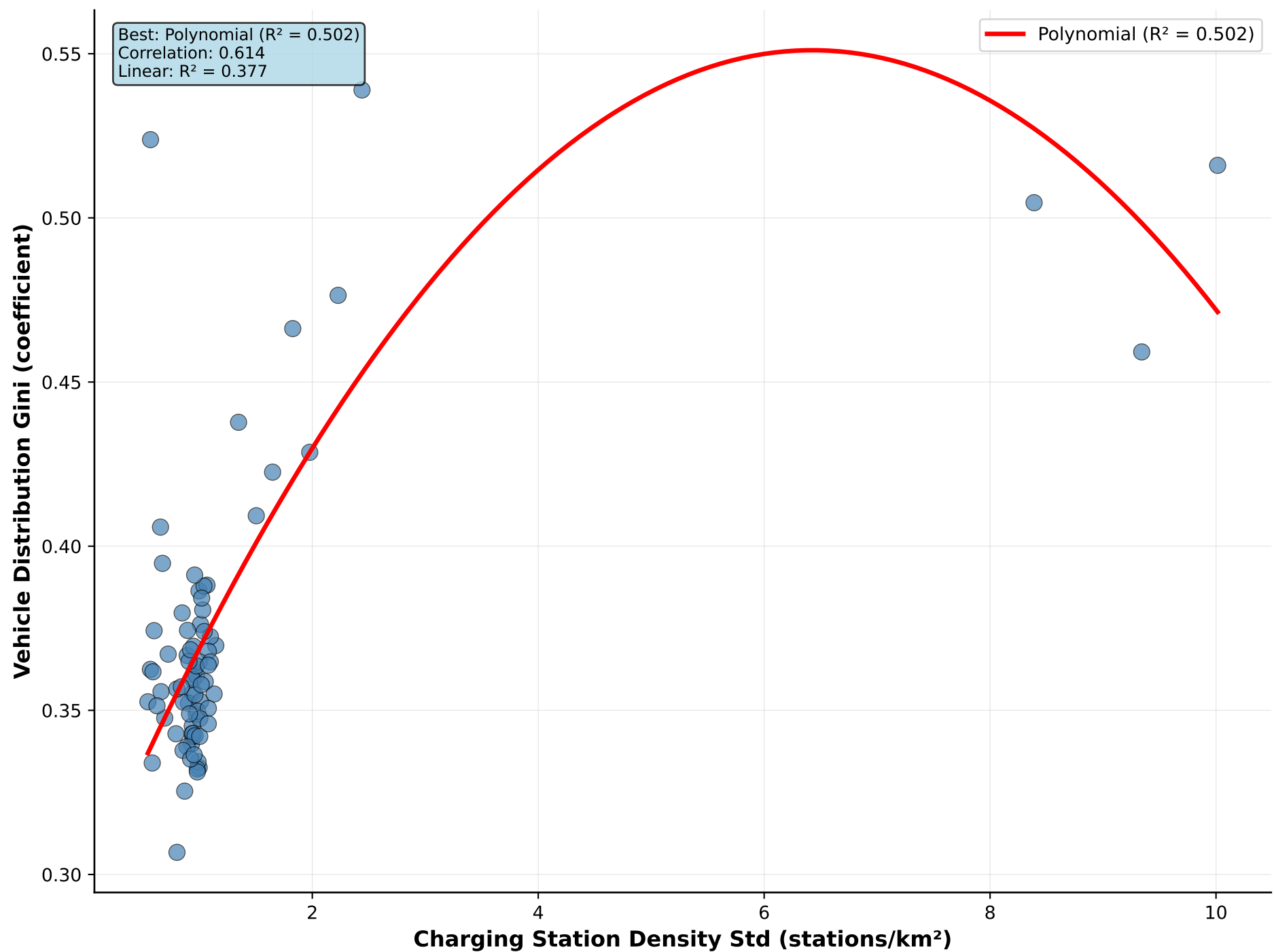
Charging Station Density Std vs Vehicle Distribution Gini
