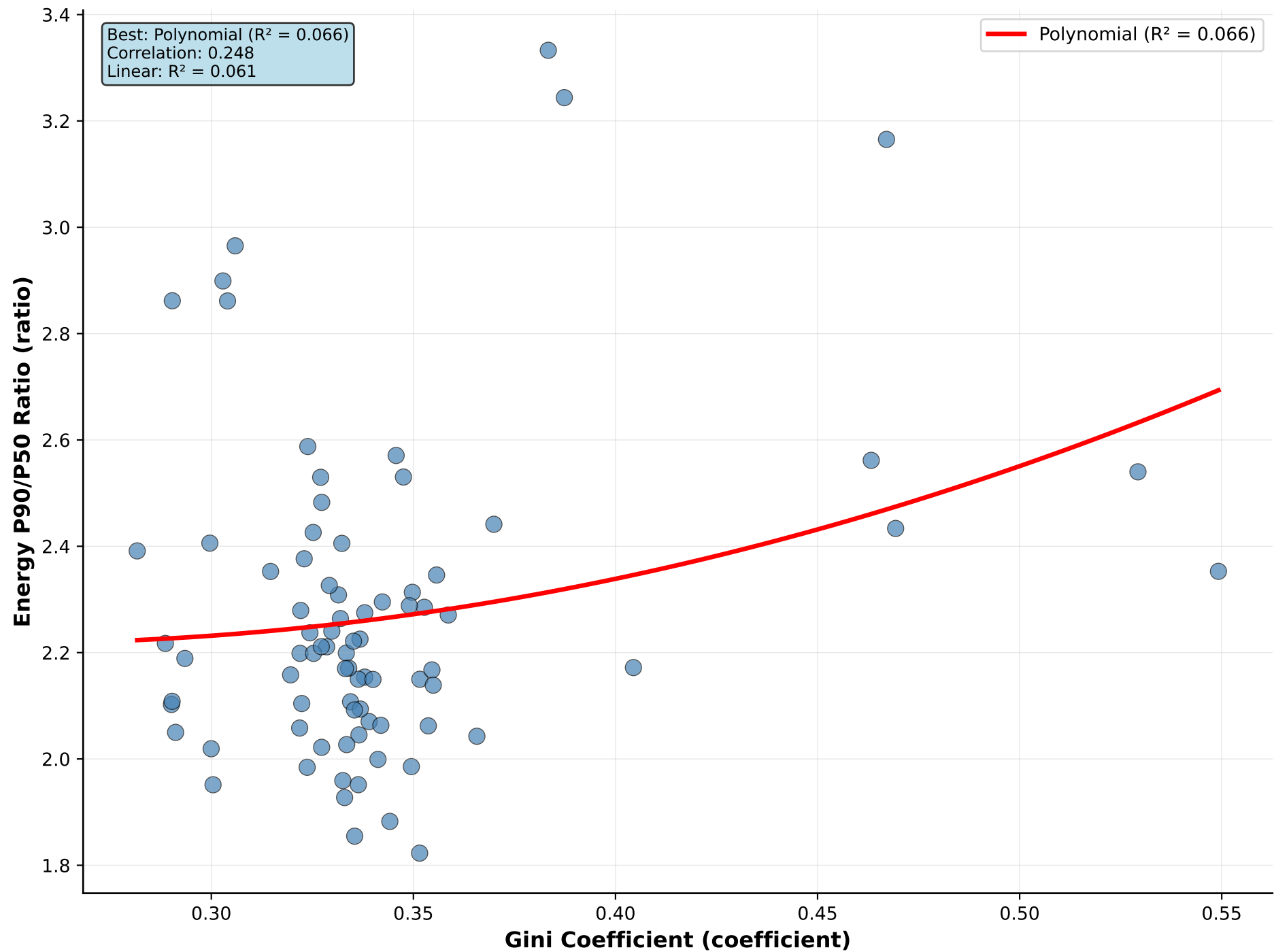
Gini Coefficient vs Energy P90/P50 Ratio
