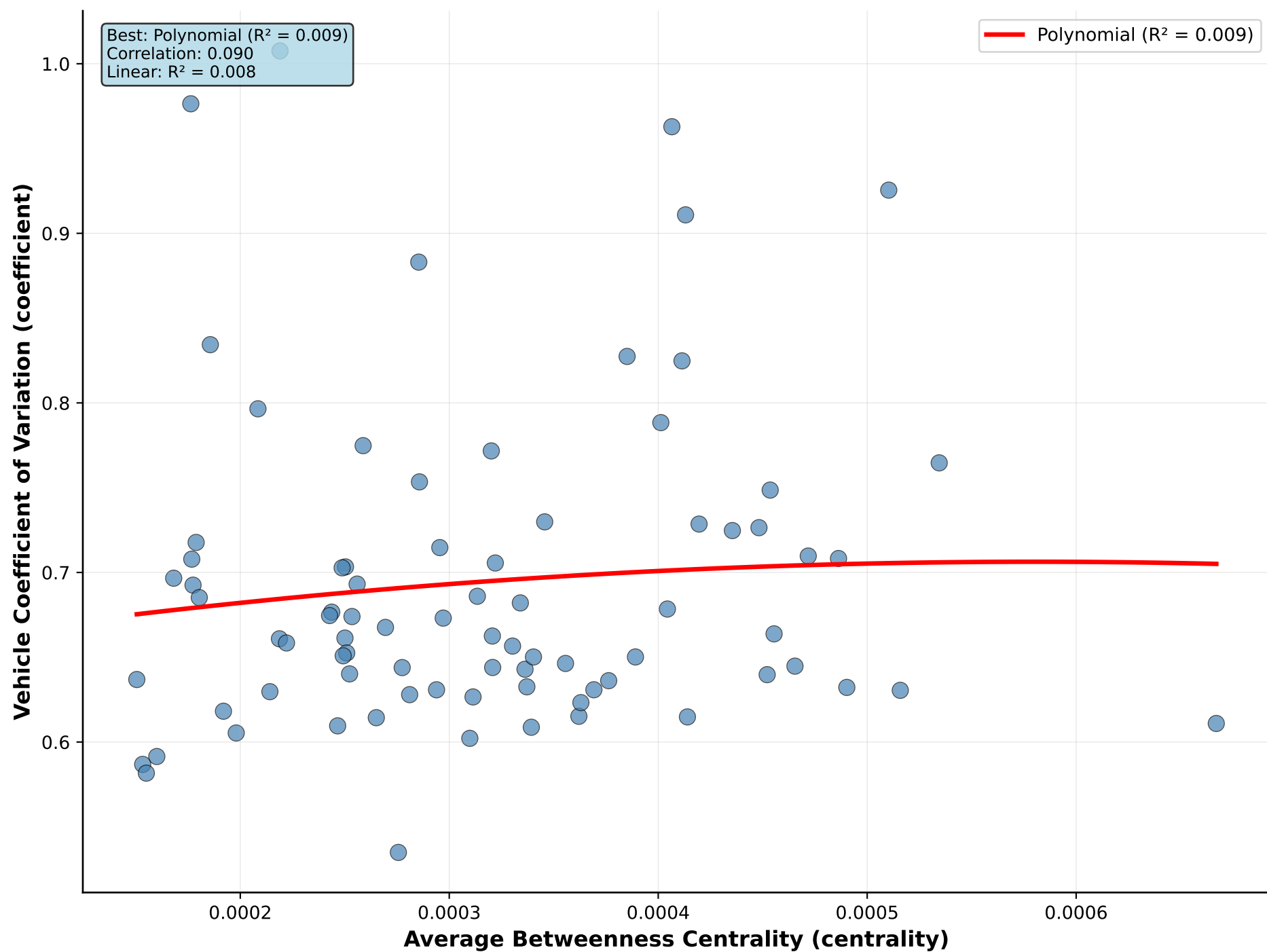
Average Betweenness Centrality vs Vehicle Coefficient of Variation
