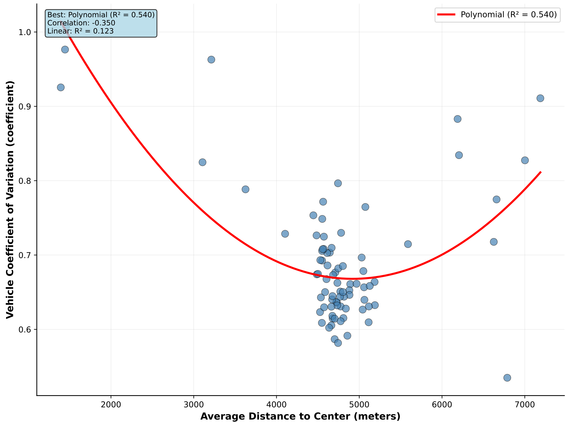
Average Distance to Center vs Vehicle Coefficient of Variation
