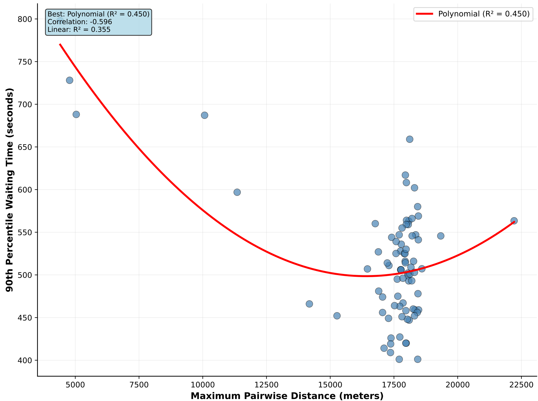
Maximum Pairwise Distance vs 90th Percentile Waiting Time
