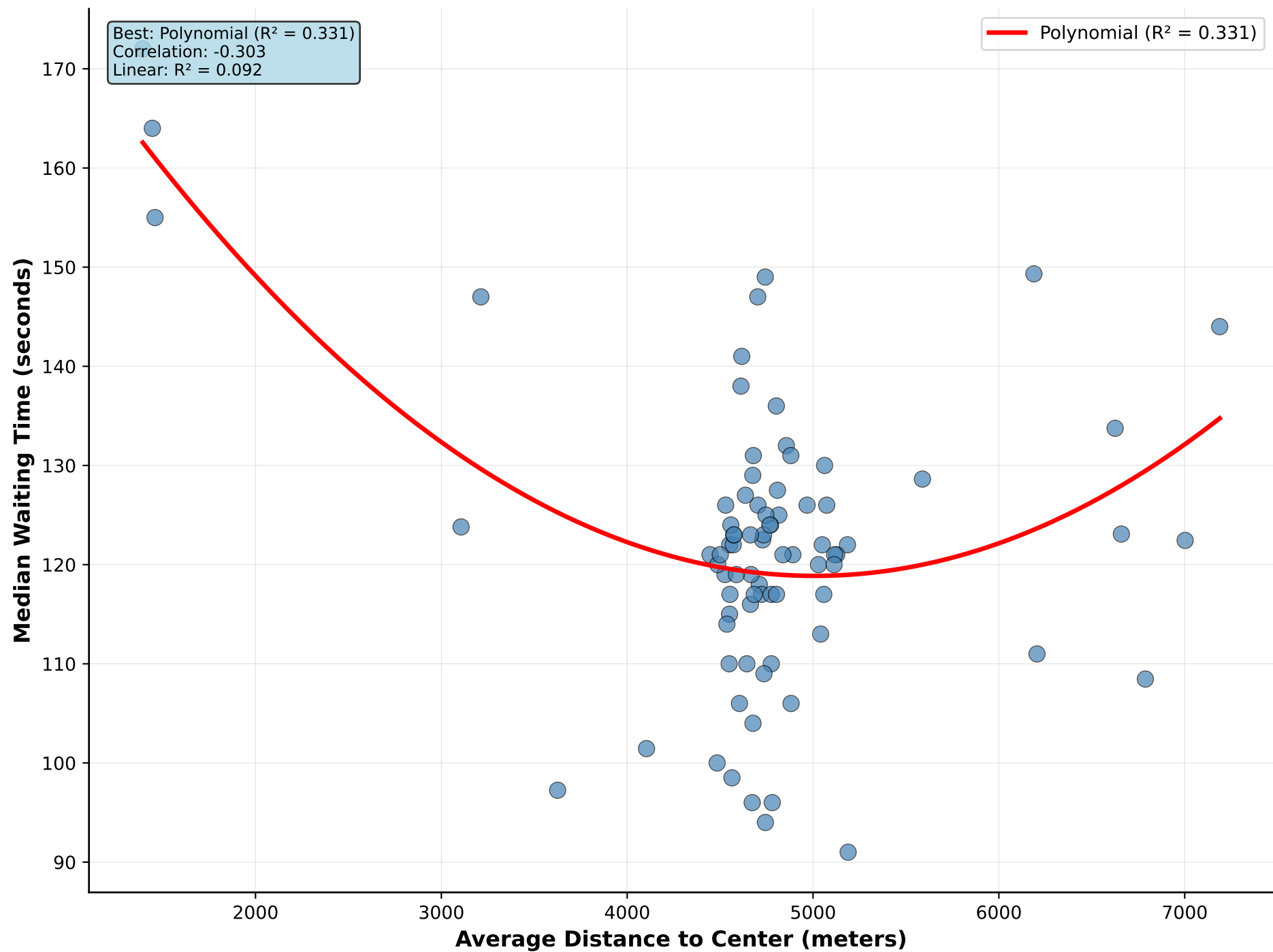
Average Distance to Center vs Median Waiting Time
