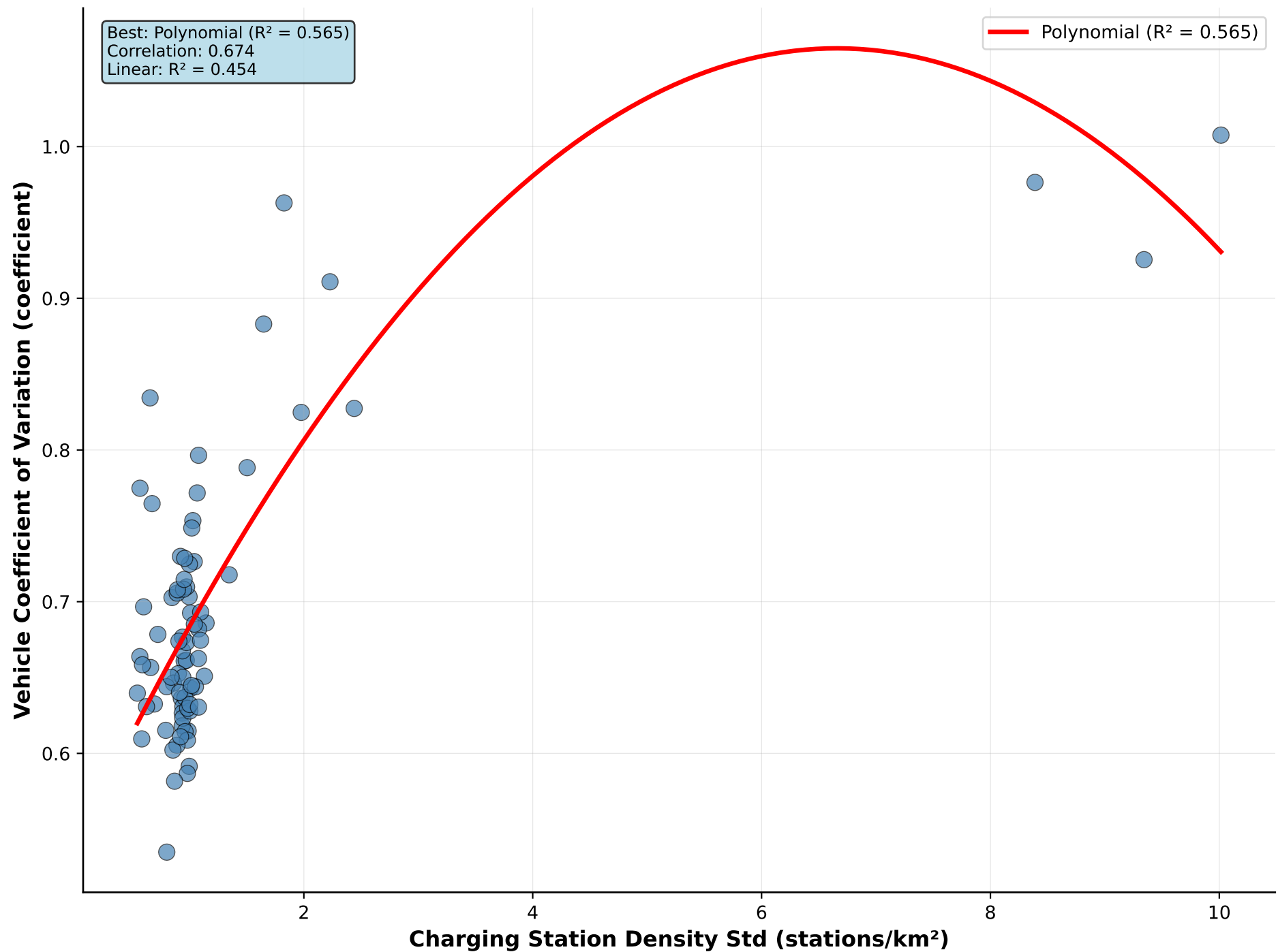
Charging Station Density Std vs Vehicle Coefficient of Variation
