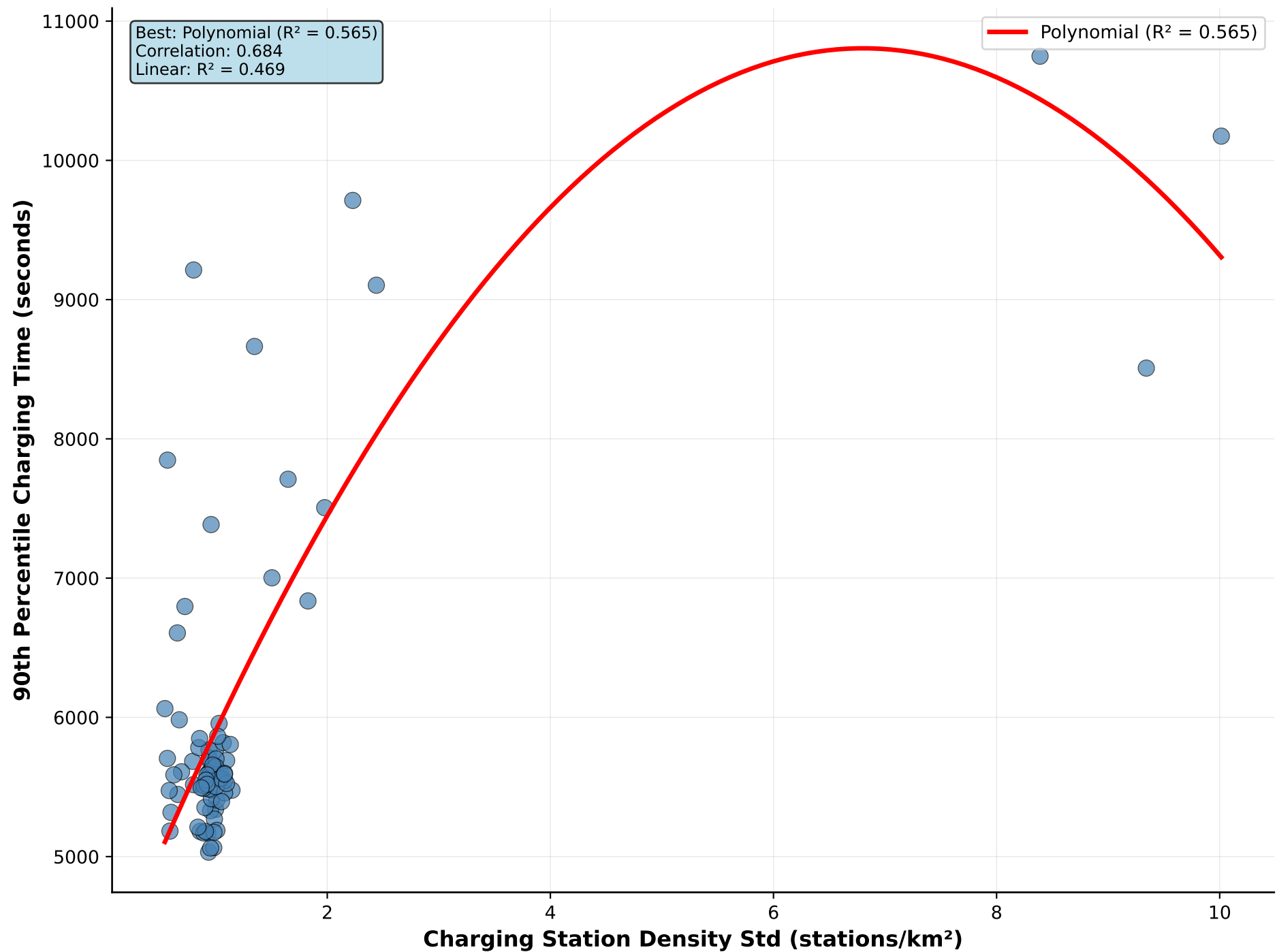
Charging Station Density Std vs 90th Percentile Charging Time
