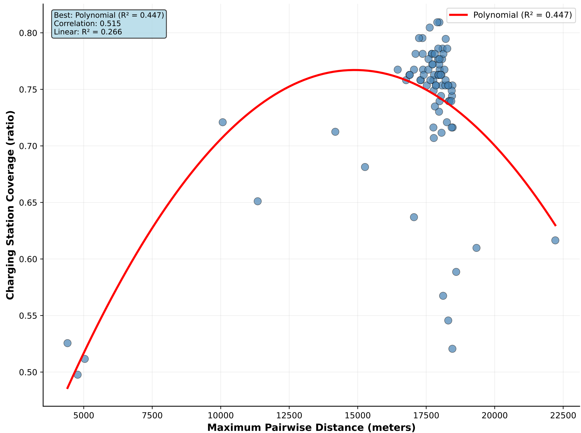
Maximum Pairwise Distance vs Charging Station Coverage
