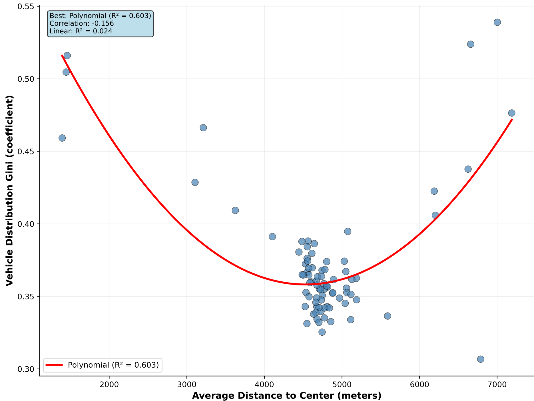
Average Distance to Center vs Vehicle Distribution Gini
