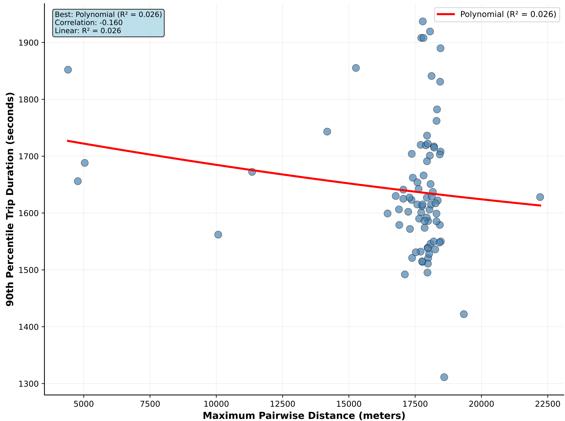
Maximum Pairwise Distances vs 90th Percentile Trip Duration
