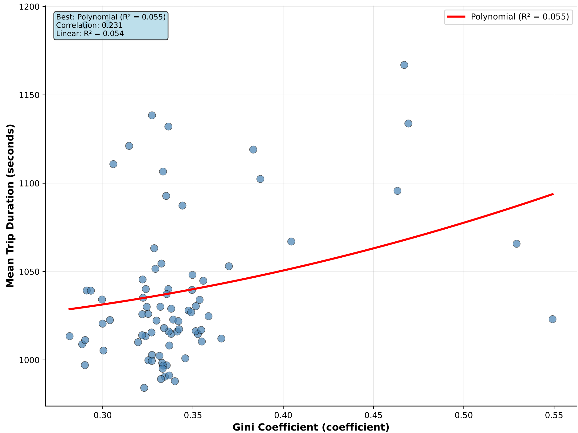
Gini Coefficient vs Mean Trip Duration
