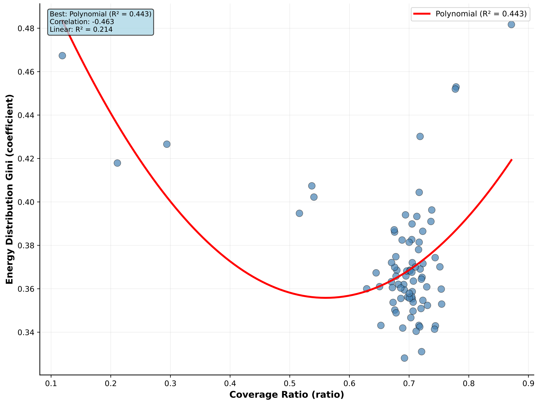
Coverage Ratio vs Energy Distribution Gini
