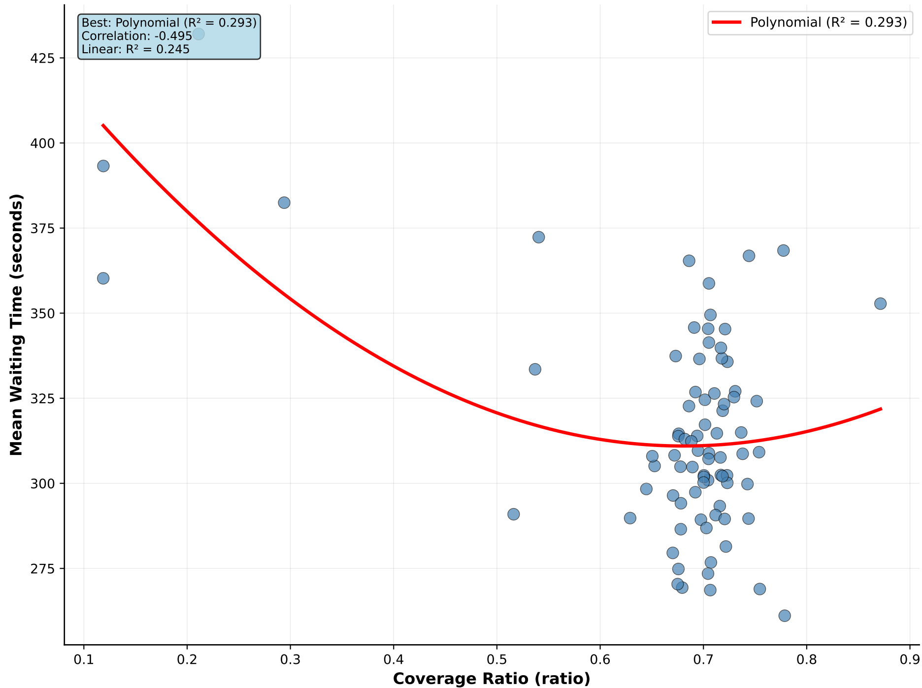
Coverage Ratio vs Mean Waiting Time
