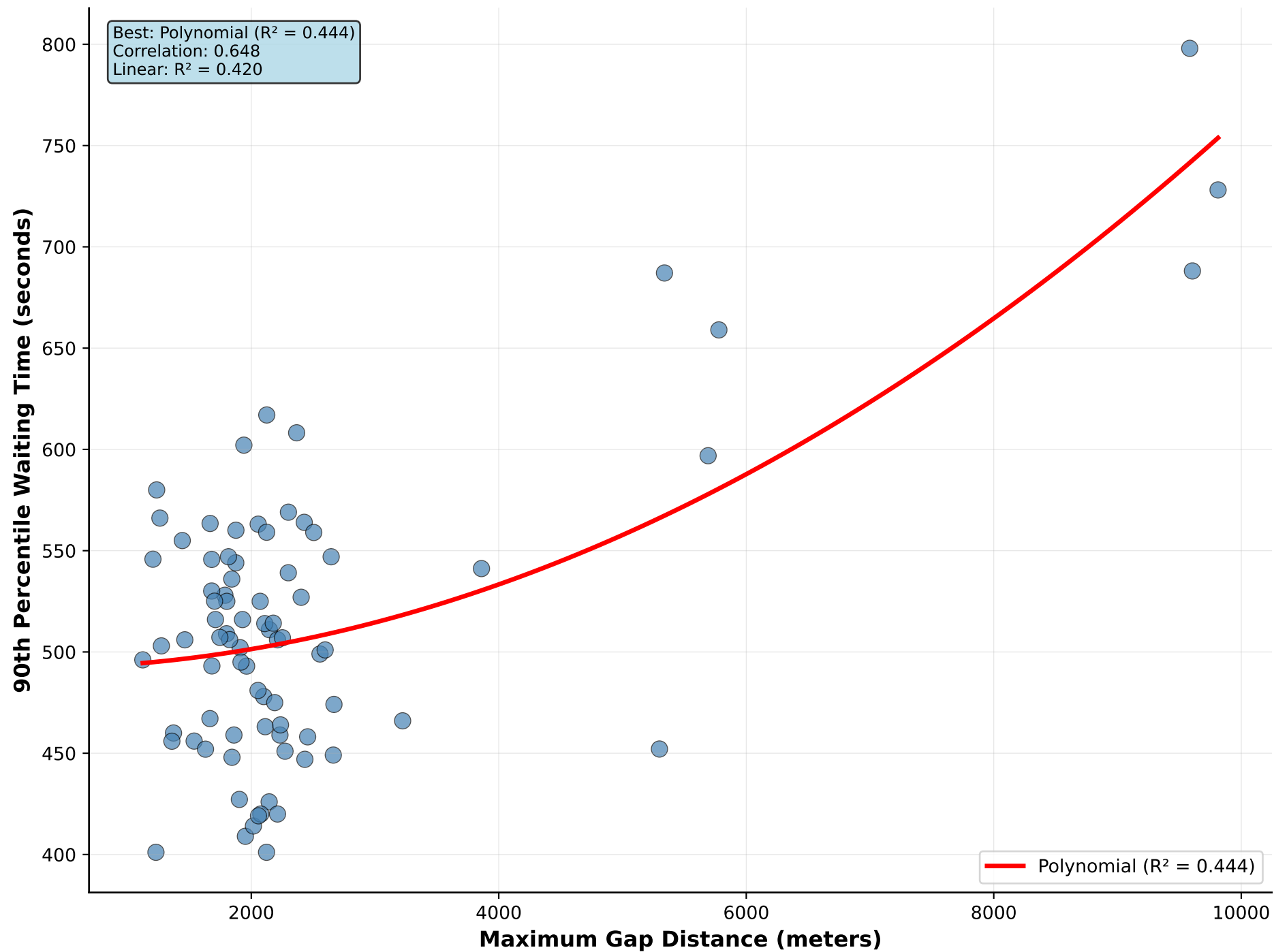
Maximum Gap Distance vs 90th Percentile Waiting Time
