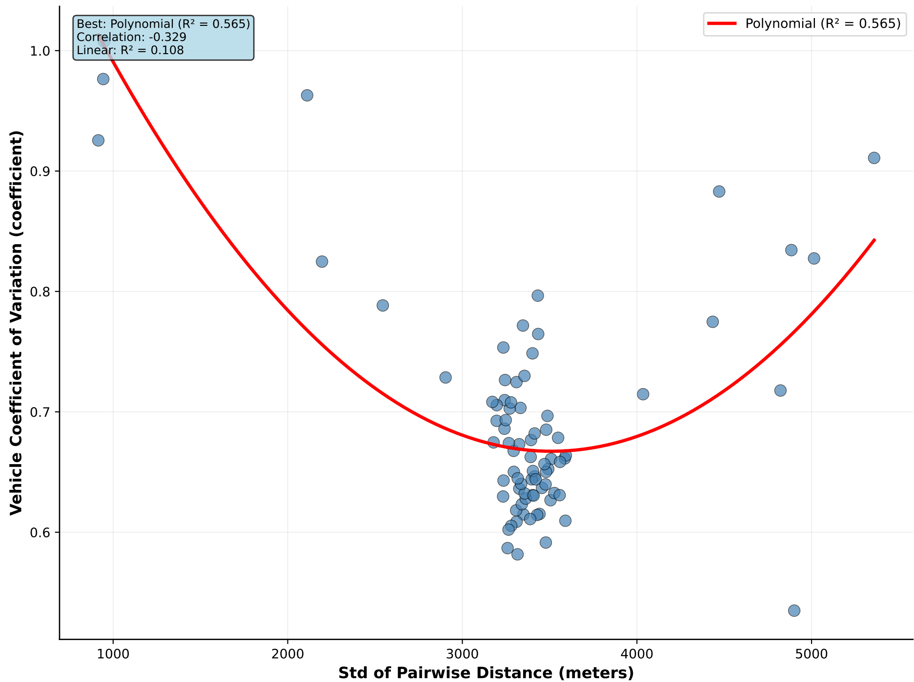
Std of Pairwise Distance vs Vehicle Coefficient of Variation
