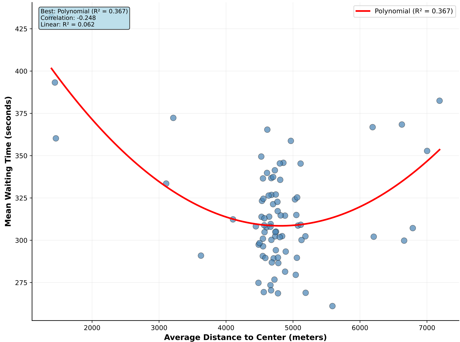
Average Distance to Center vs Mean Waiting Time
