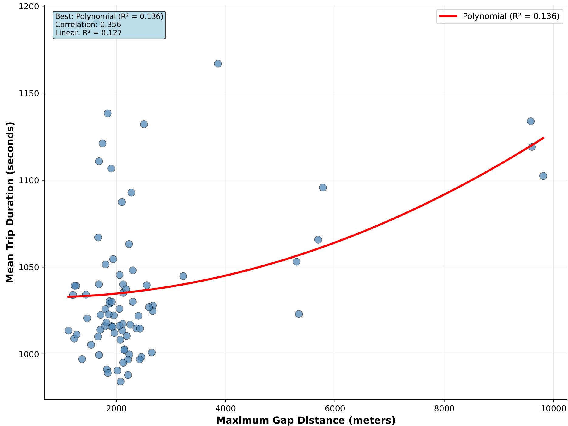
Maximum Gap Distance vs Mean Trip Duration
