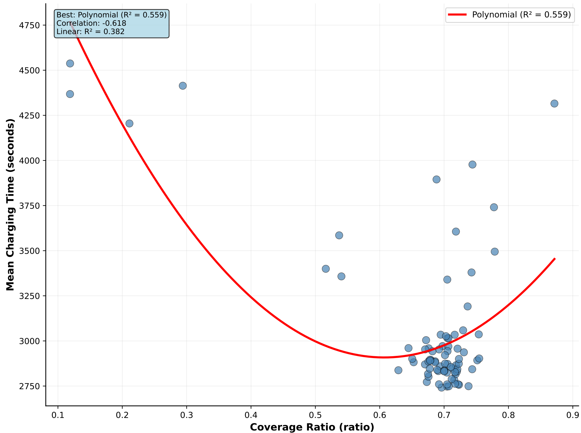
Coverage Ratio vs Mean Charging Time
