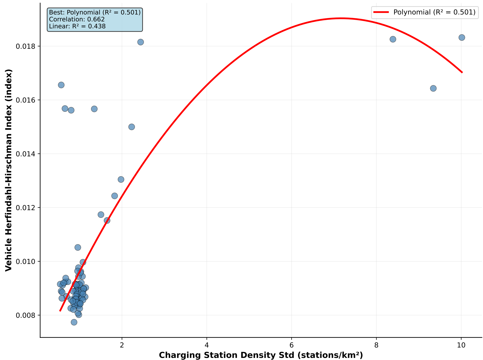
Charging Station Density Std vs Vehicle Herfindahl-Hirschman Index
