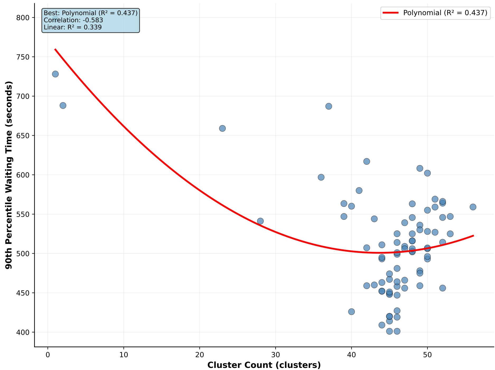
Cluster Count vs 90th Percentile Waiting Time
