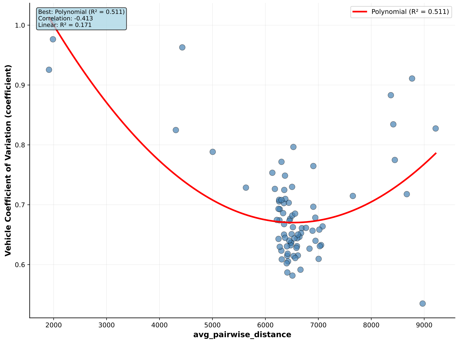
avg_pairwise_distance vs Vehicle Coefficient of Variation
