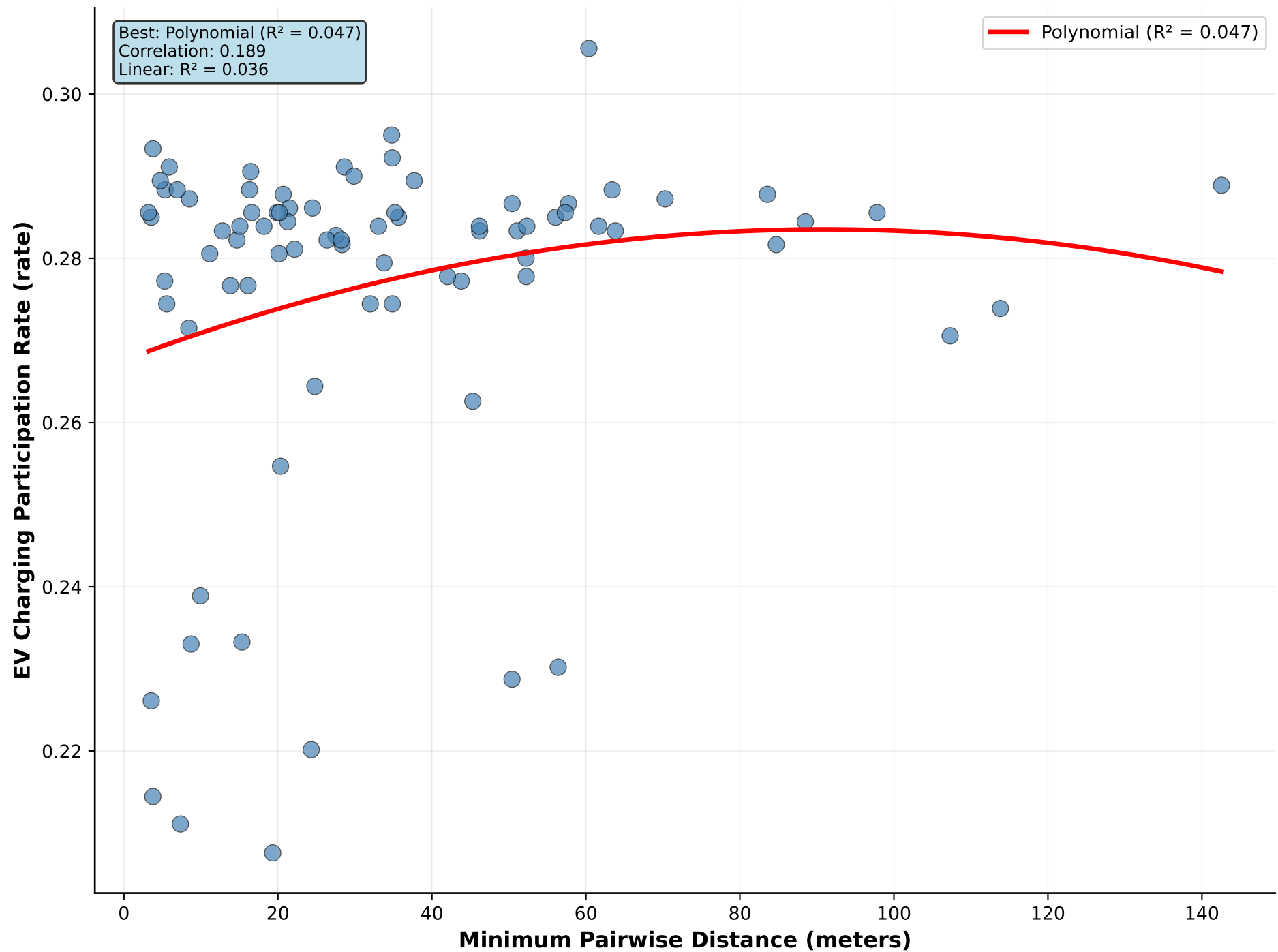
Minimum Pairwise Distance vs EV Charging Participation Rate
