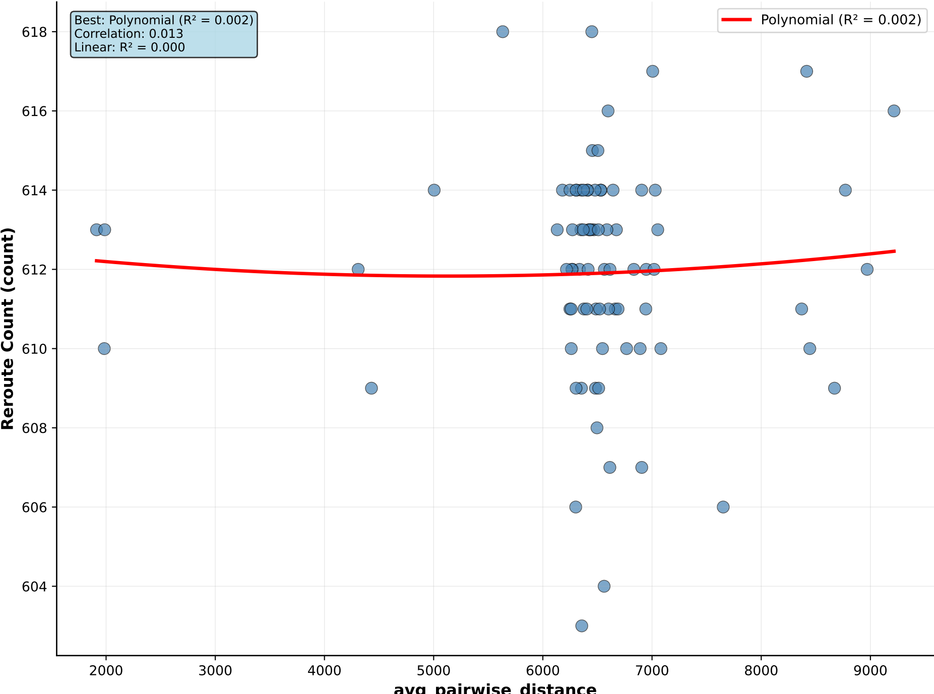
avg_pairwise_distance vs Reroute Count
