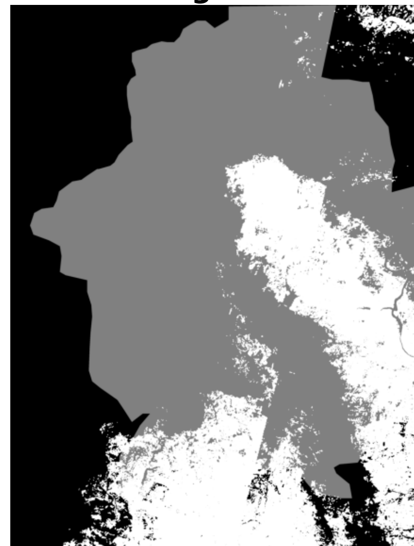
Change Mask
