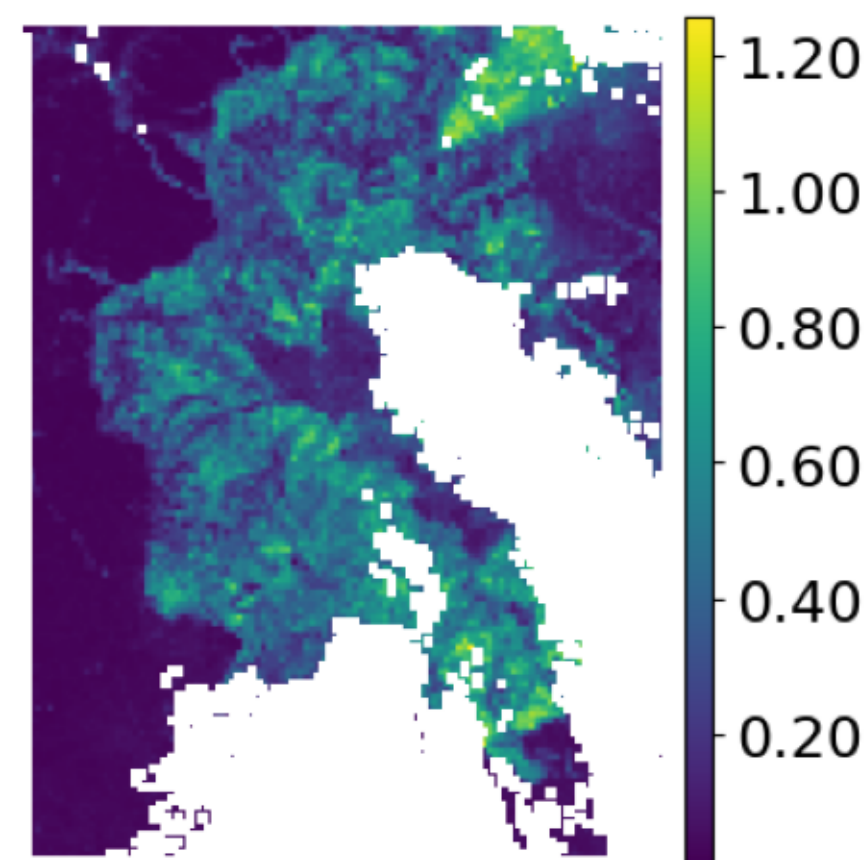
RaVAEn - best
