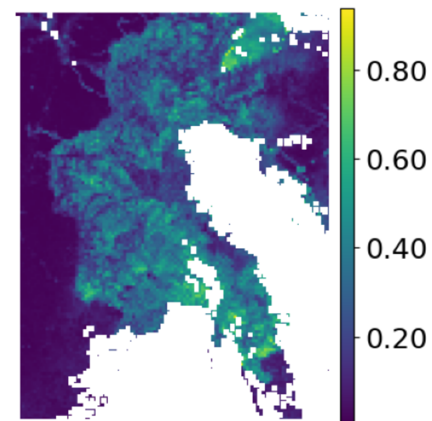
STTORM-CD - best
