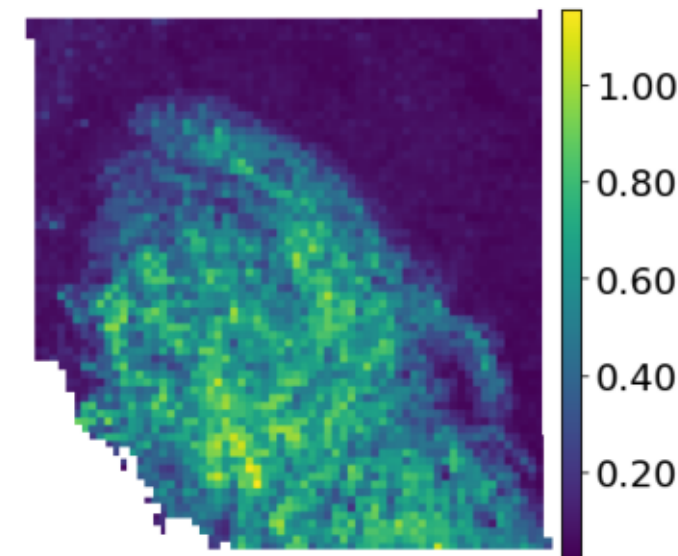
RaVAEn - best
