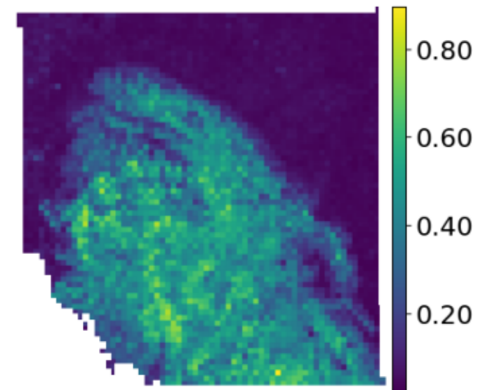
STTORM-CD - best
