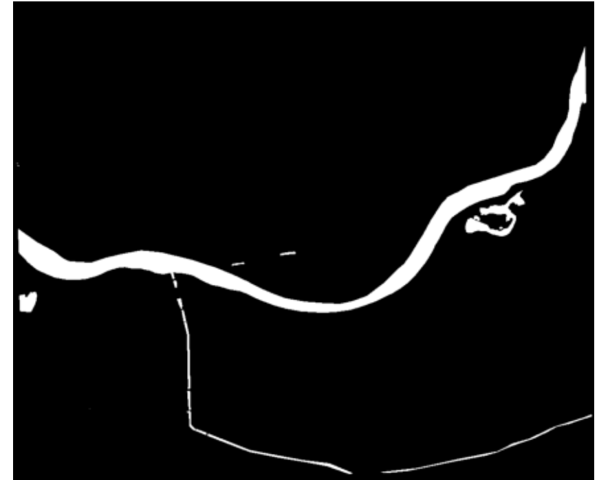
Change Mask
