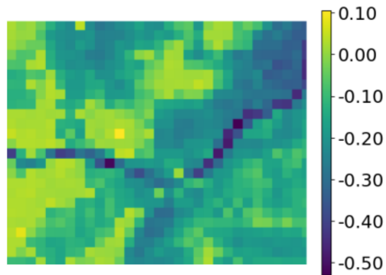
NDWI
