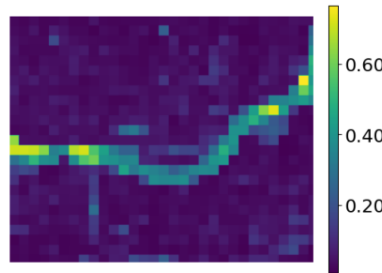
RaVAEn - best
