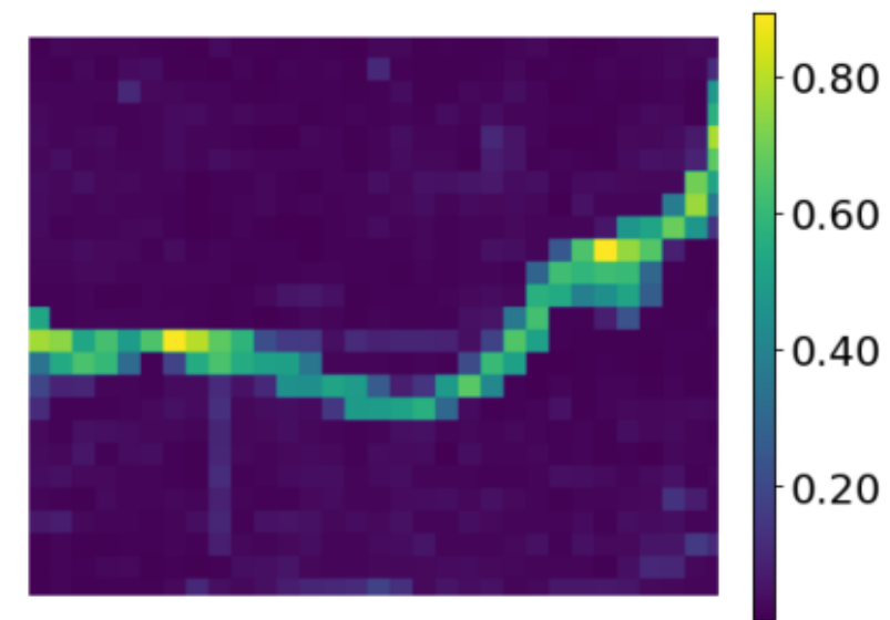
STTORM-CD - best
