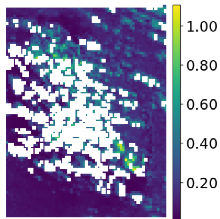
STTORM-CD - best
