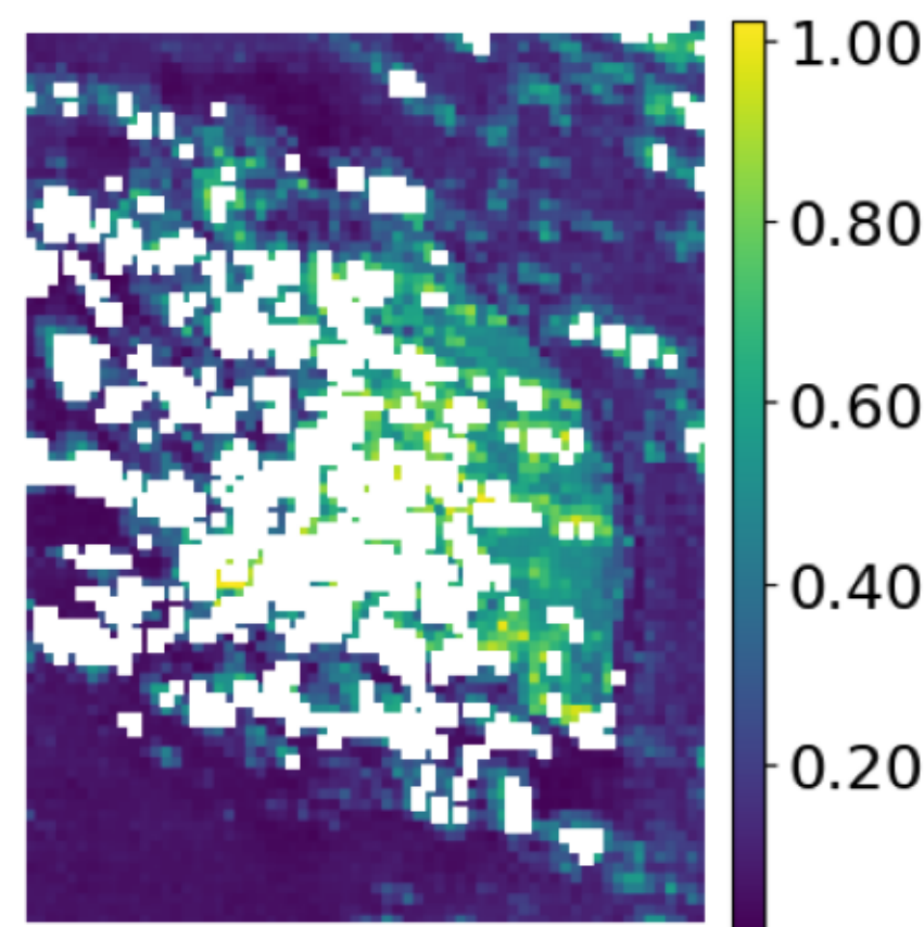
RaVAEn - best
