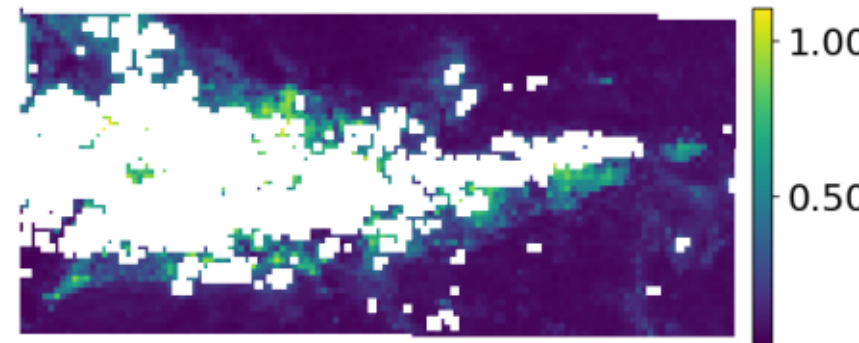
RaVAEn - best
