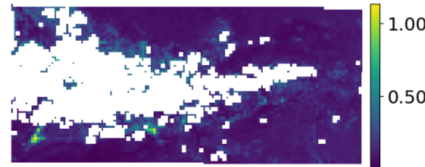
STTORM-CD - best
