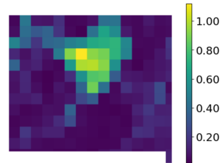
STTORM-CD - best
