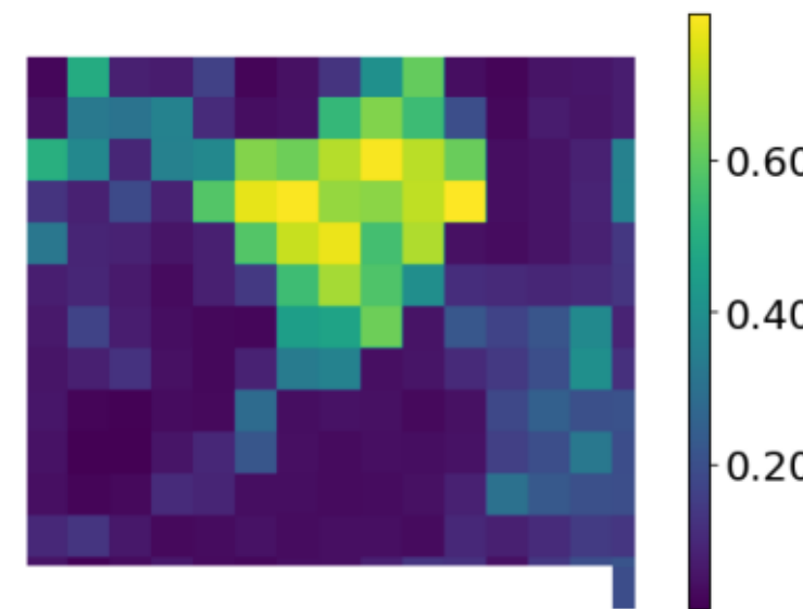
RaVAEn - best
