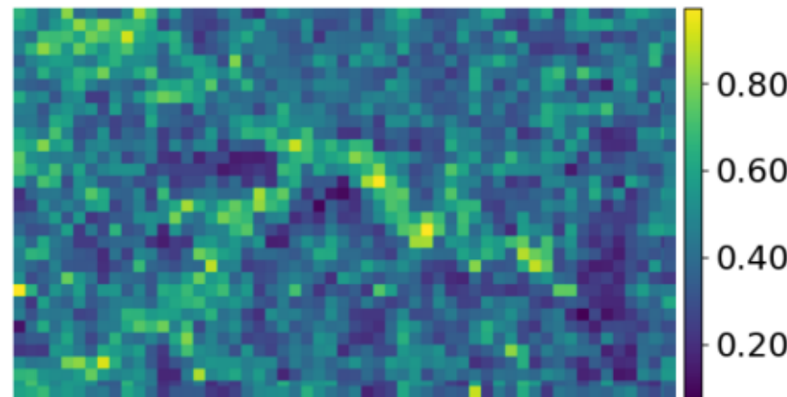
RaVAEn - best
