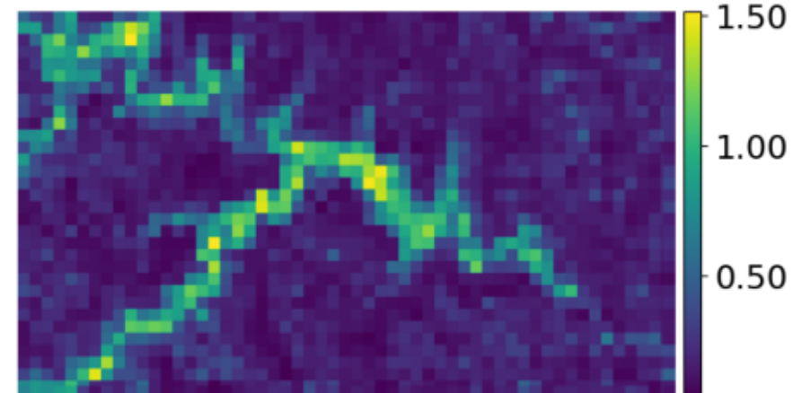
STTORM-CD - best
