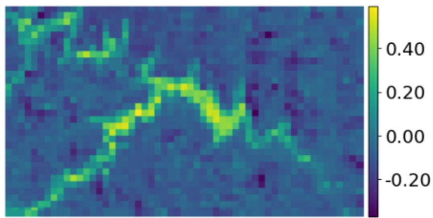
NDWI
