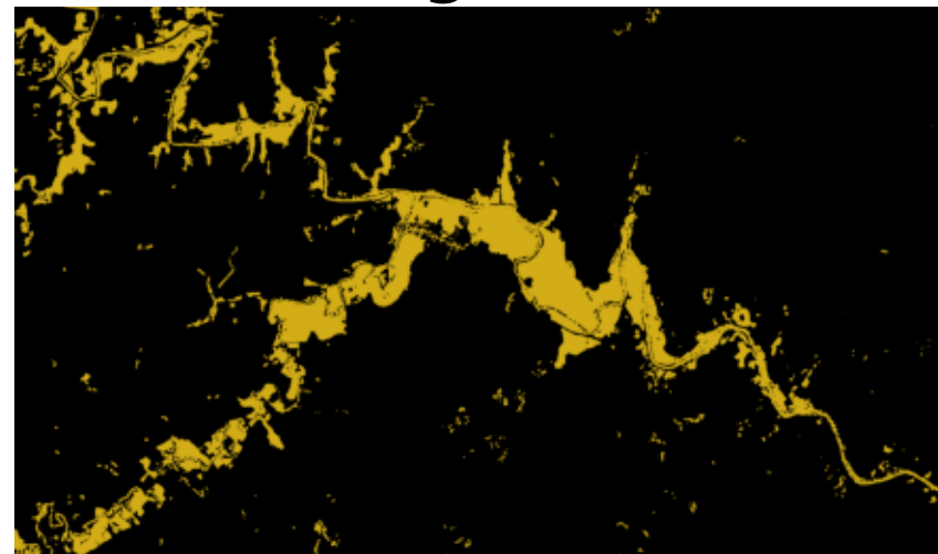
RaVAEn - best
