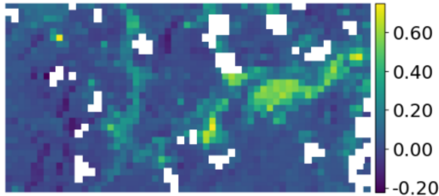
NDWI
