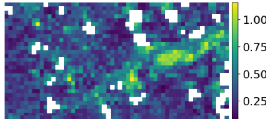
RaVAEn - best
