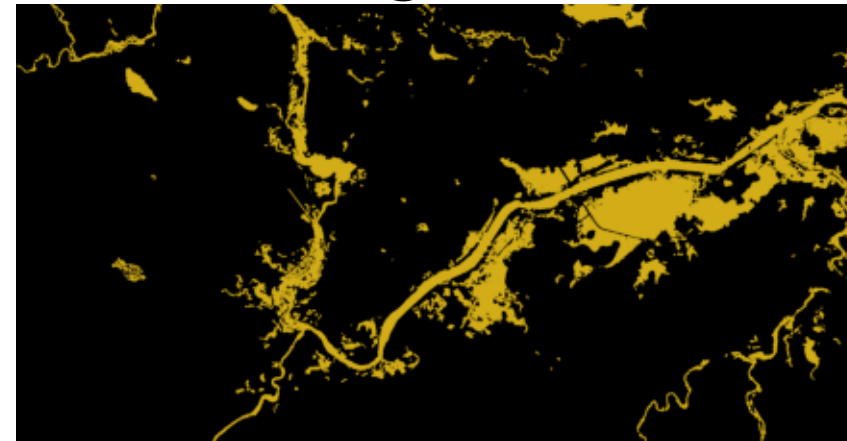
Change Mask
