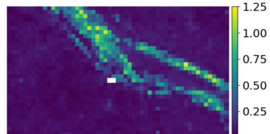
STTORM-CD - best
