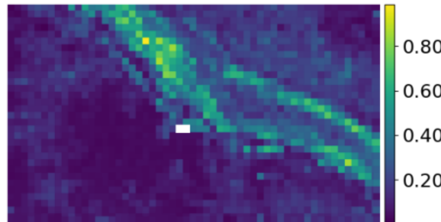
RaVAEn - best
