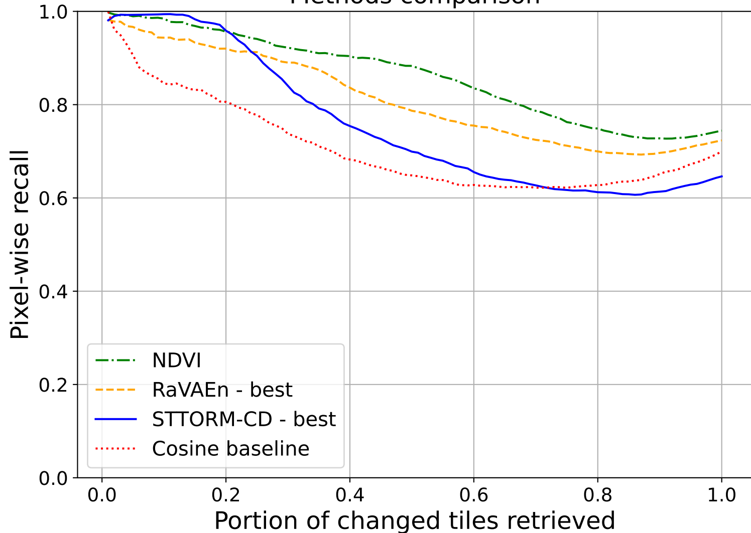
Methods comparison
