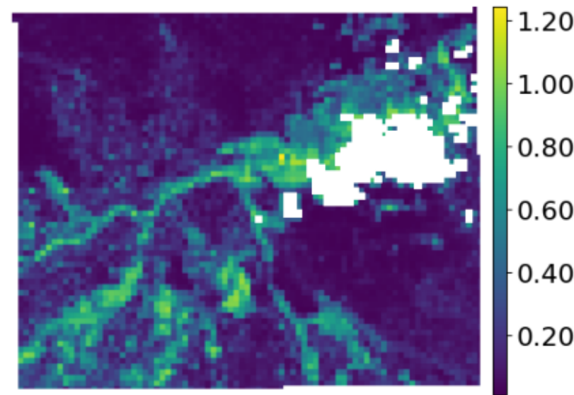
RaVAEn - best
