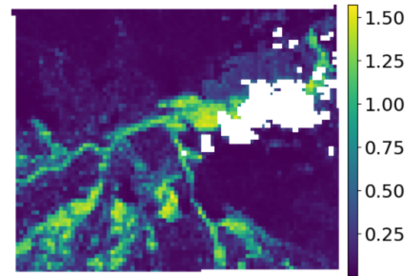
STTORM-CD - best
