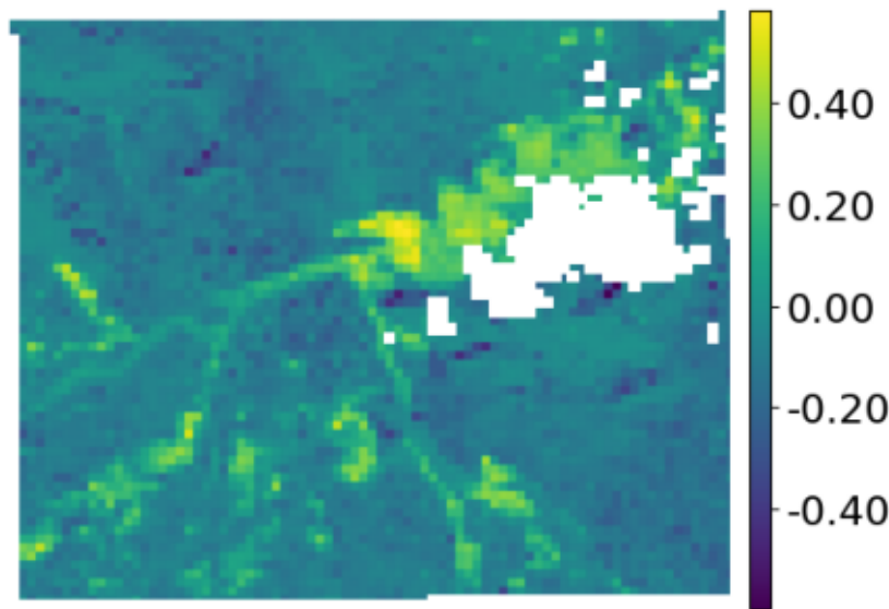
NDWI
