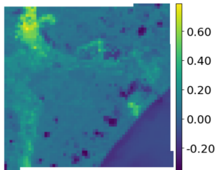
NDWI
