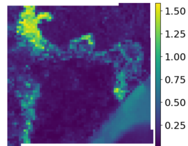
STTORM-CD - best
