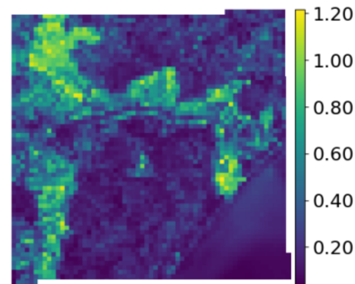
RaVAEn - best
