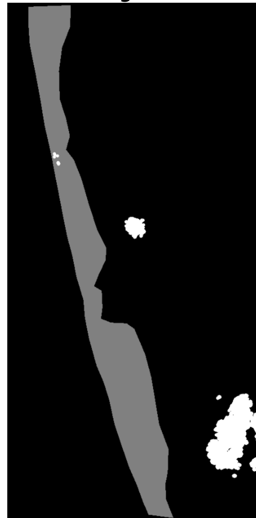
Change Mask
