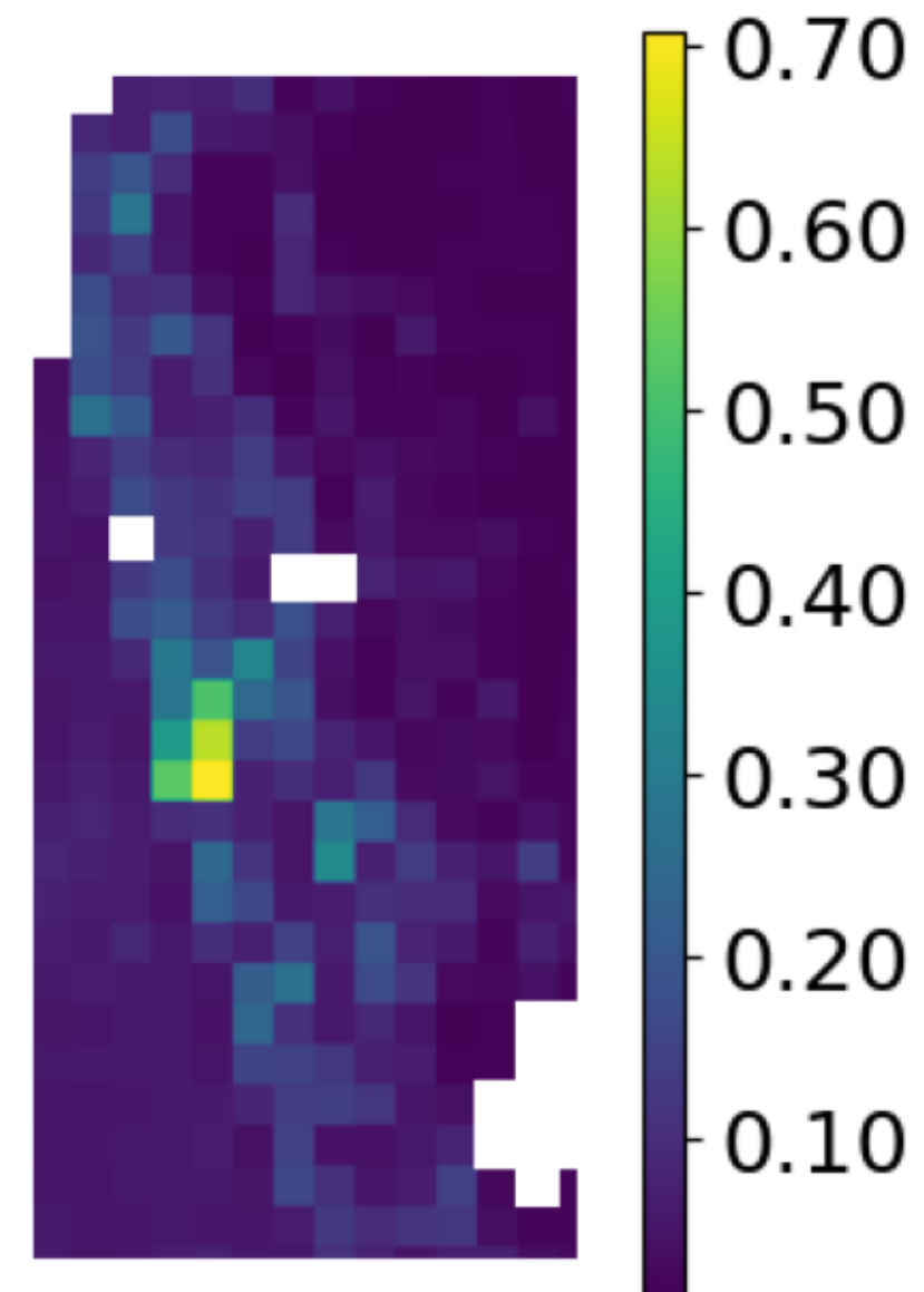
STTORM-CD - best
