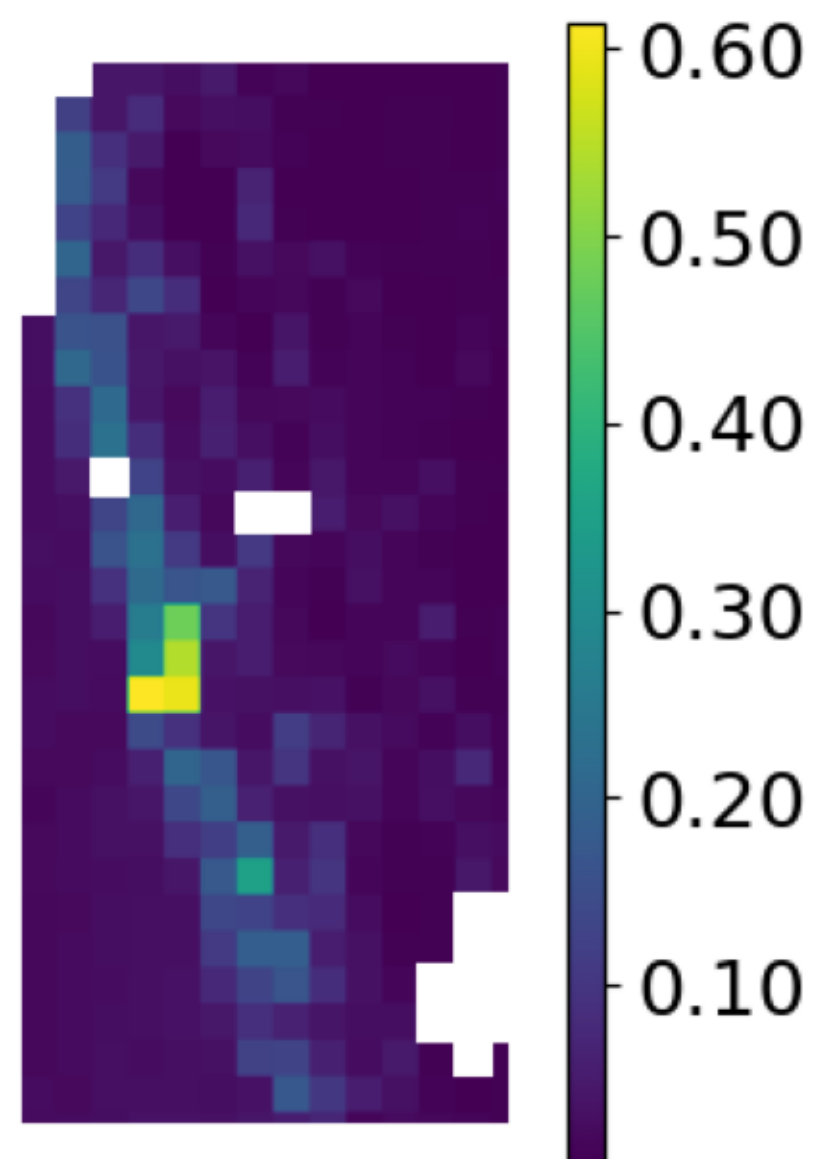
RaVAEn - best
