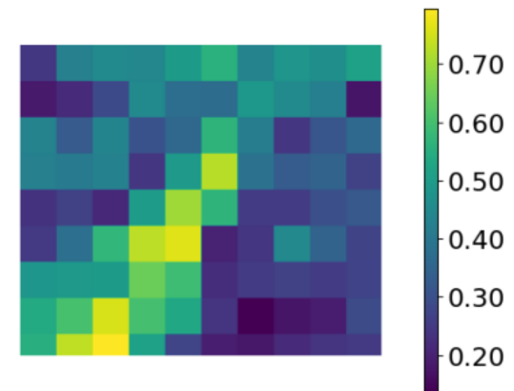
STTORM-CD - best
