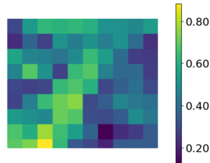
RaVAEn - best
