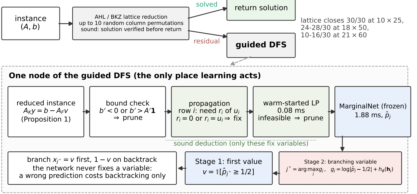
Figure 1: The deployed system. A lattice stage runs first and returns a verified solution when it succeeds; the guided depth-first search sees the residual. Inside a search node, sound deduction (bound check, propagation, the relaxation’s infeasibility test) is what may fix variables or prune, and the learned components only choose the branching variable and the value tried first. The frozen marginal network supplies \hat{p}_j ; Stage 1 takes the value from it, Stage 2 takes the variable from the cost-tuned policy head. Neither fixes a variable, so a wrong prediction costs backtracking and nothing else.
