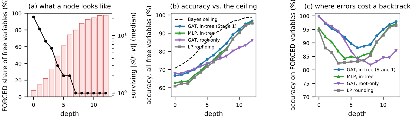
Figure 7: Prediction against the exact posterior on 2,640 held-out in-tree states of 10 \times 25 instances, by depth. (a) The FORCED share of free variables and the median number of surviving solutions. (b) Per-variable accuracy on all free variables against the Bayes ceiling (3). (c) Accuracy on FORCED variables, where an error costs a backtrack. Four predictors share the labels, the loss and the states: the Stage-1 network (a GAT trained in-tree), the same GAT trained on root states only, a graph-free MLP with constraint aggregates trained in-tree, and relaxation rounding.
