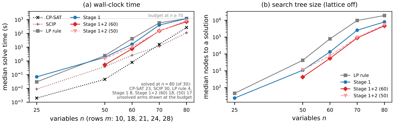
Figure 6: Scaling with size (Table 4). (a) Median wall-clock time; at n \geq 70 whiskers span the three seeds and at n = 80 the labels give solve counts, with unsolved arms drawn at the budget. (b) Median nodes to a solution, lattice off. Both stages were trained at n \leq 60 .
