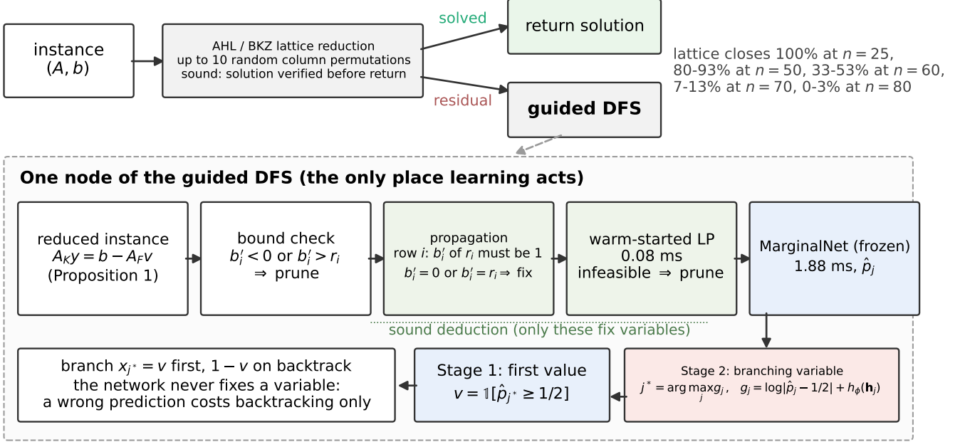
Figure 1: The deployed system. A lattice stage runs first and returns a verified solution when it succeeds; the guided depth-first search receives the residual. Inside a node, only sound deduction (bound check, propagation, relaxation infeasibility) fixes variables or prunes; the learned components choose the branching variable and the value tried first. The frozen marginal network supplies \hat{p}_j ; Stage 1 takes the value from it, Stage 2 takes the variable from the cost-tuned policy head. A wrong prediction costs backtracking and nothing else.
