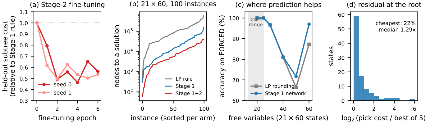
Figure 5: (a) Stage-2 fine-tuning: total subtree cost on 150 held-out states relative to the Stage-1 rule, two training seeds; the selected epochs are 4 and 2. (b) Nodes to a solution on the 100-instance 21 \times 60 set, each arm sorted. (c) Accuracy on FORCED variables of 21 \times 60 in-tree states by number of free variables: the Stage-1 margin over relaxation rounding lies outside its training range. (d) Residual at the root: cost of the confidence rule’s choice relative to the cheapest of its five candidates (100 held-out states, 45–50 free variables).
