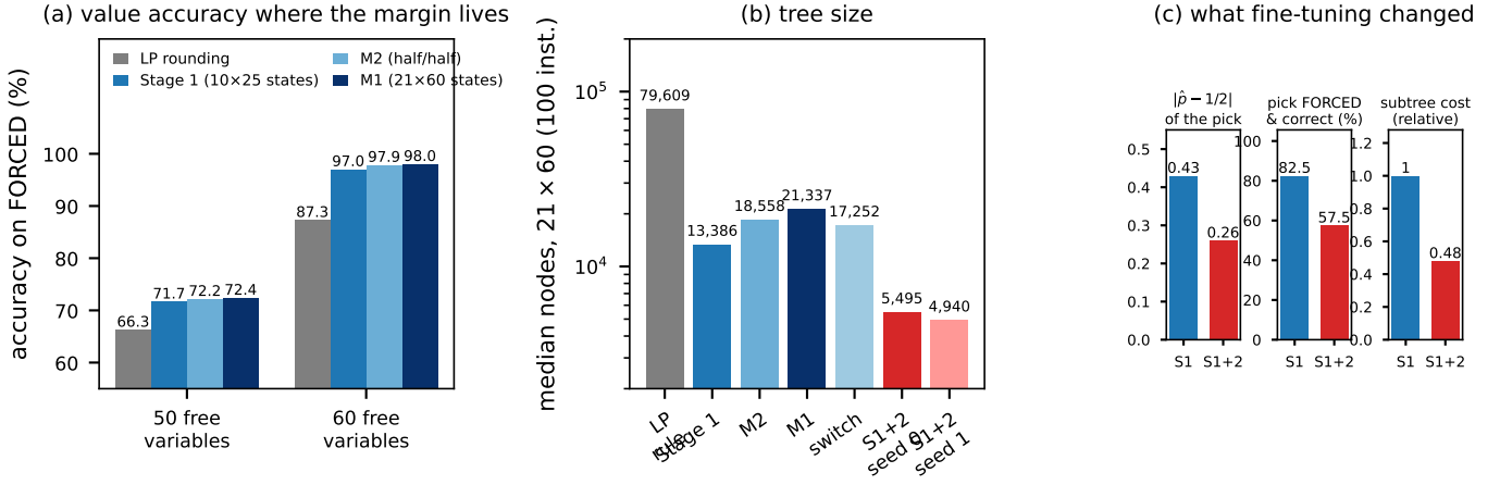
Figure 8: Value accuracy and tree size move independently. (a) Accuracy on FORCED variables of 21 \times 60 in-tree states with 50 and 60 free variables, for relaxation rounding, the Stage-1 network trained on 10 \times 25 states, and the same architecture trained on 21 \times 60 states (M1) or on a half-and-half mix (M2). (b) Median nodes on the 100-instance set: the networks with the higher value accuracy expand more nodes; the cost-tuned policy expands fewer. (c) On 300 held-out states the fine-tuned policy picks less confident variables that are less often FORCED-and-correct, and its subtree cost is half.
