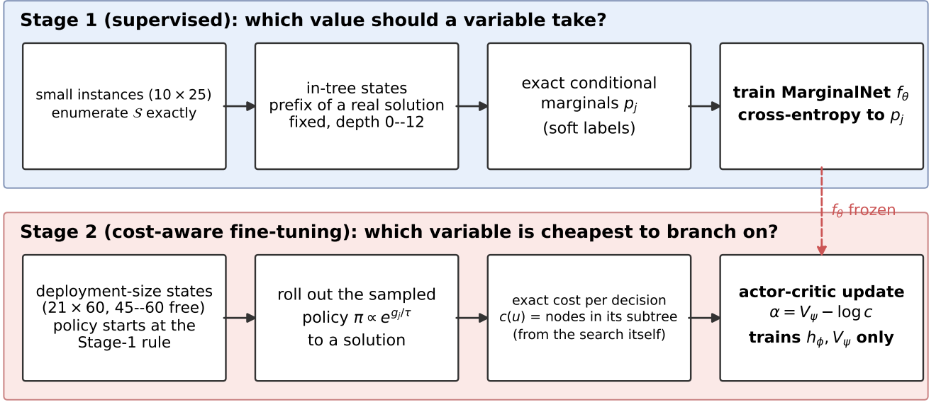
Figure 4: The two training stages. Stage 1 learns which value from exact conditional marginals of enumerable instances; Stage 2 learns which variable from the exact subtree cost of every decision, produced by the search, with the Stage-1 network frozen.
