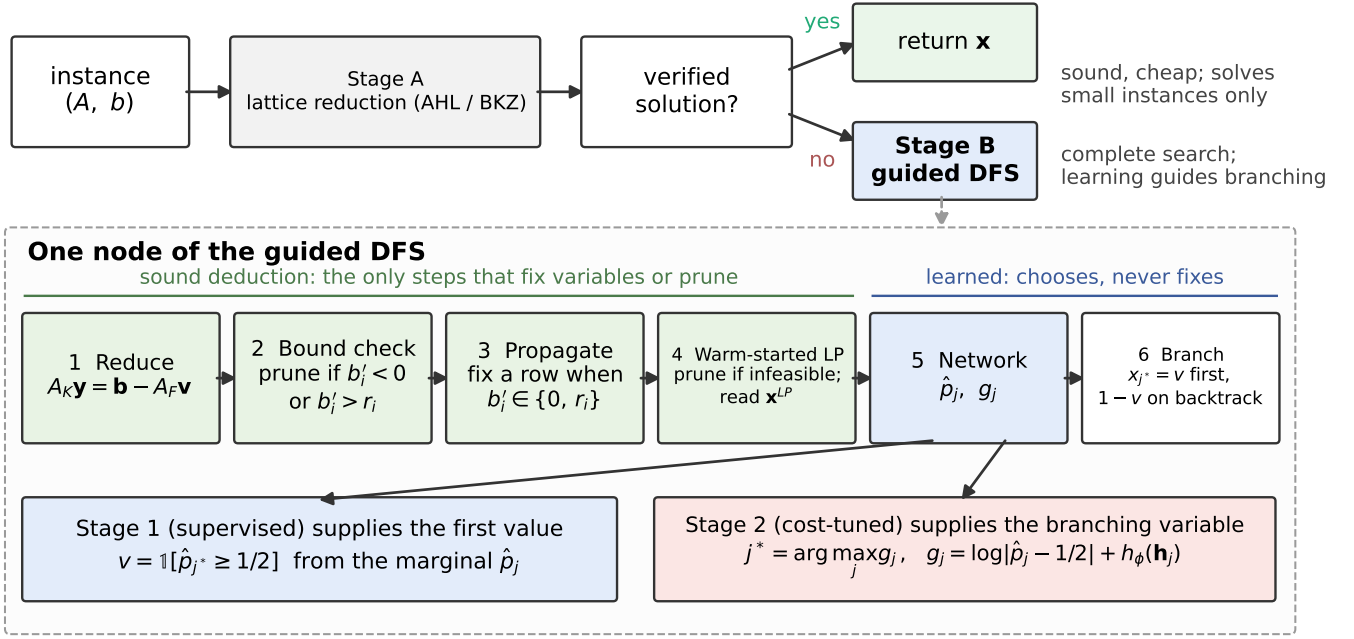
Figure 1: The deployed solver. Stage A, lattice reduction, returns a verified solution when it finds one; Stage B, the guided depth-first search, handles the rest. Inside a node, steps 1–4 are sound and are the only steps that fix variables or prune; the network at step 5 only chooses, the value from Stage 1 and the variable from Stage 2.
