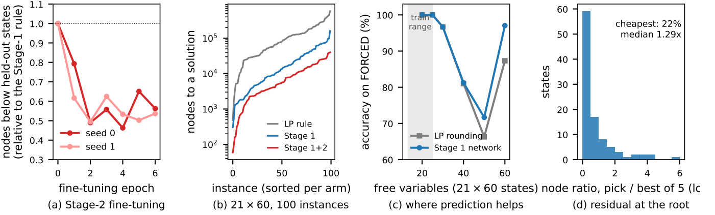
Figure 6: (a) Stage-2 fine-tuning: nodes expanded below 150 held-out states relative to the Stage-1 rule, two training seeds; the selected epochs are 4 and 2. (b) Nodes to a solution on the 100-instance 21 \times 60 set, each arm sorted. (c) Accuracy on FORCED variables of 21 \times 60 in-tree states by number of free variables: the Stage-1 margin over relaxation rounding lies outside its training range. (d) Residual at the root: nodes below the confidence rule’s choice relative to the cheapest of its five candidates (100 held-out states, 45–50 free variables).
