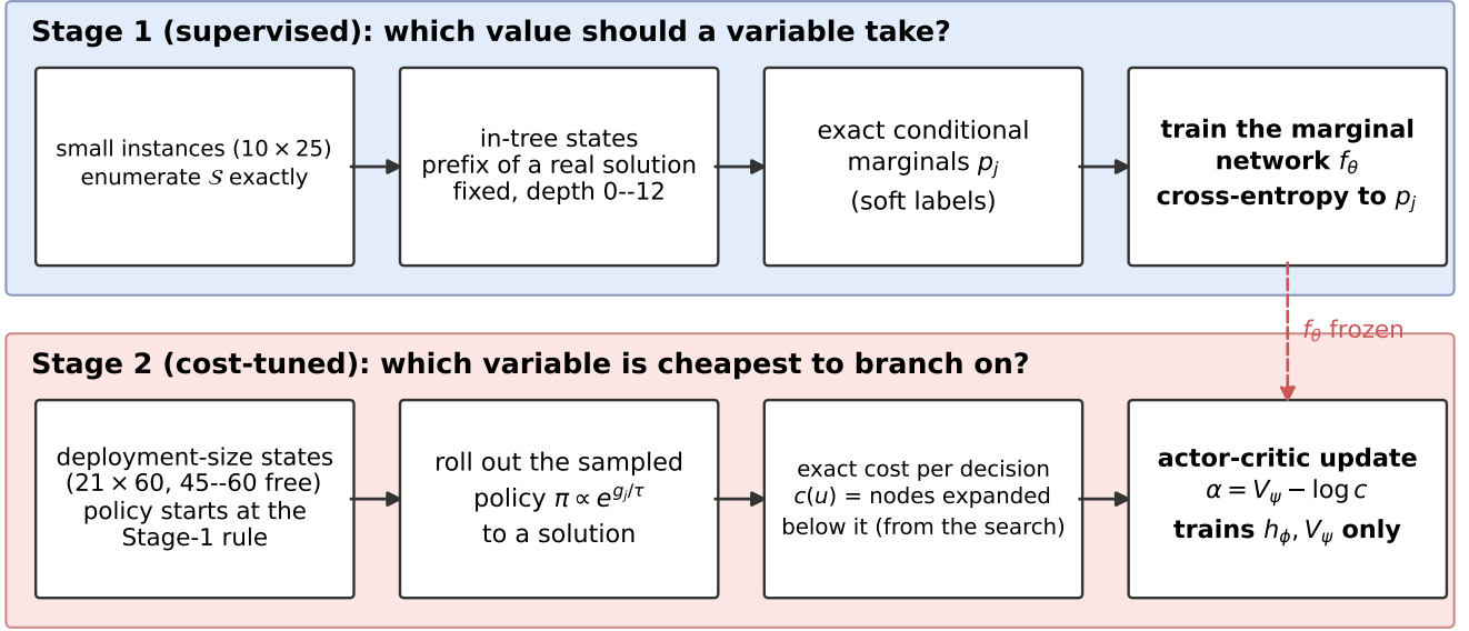
Figure 5: The two training stages. Stage 1 learns which value from exact conditional marginals of enumerable instances; Stage 2 learns which variable from the exact number of nodes every decision costs, produced by the search, with the Stage-1 network frozen.
