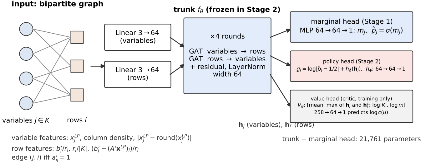
Figure 4: The network. The reduced instance enters as a bipartite graph with three features per variable and per row; a trunk of four graph-attention rounds produces an embedding per variable and per row; three heads read them. The marginal head is trained in Stage 1, the policy head in Stage 2 on the frozen trunk, and the value head serves only as the critic during Stage 2.
