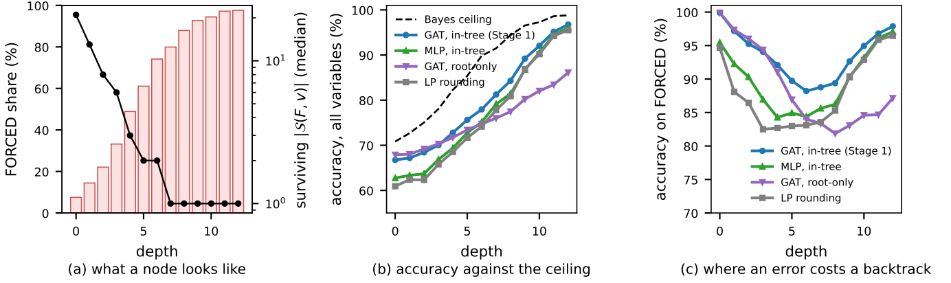
Figure 8: Prediction against the exact posterior on 2,640 held-out in-tree states of 10 \times 25 instances, by depth. (a) The FORCED share of free variables and the median number of surviving solutions. (b) Per-variable accuracy on all free variables against the Bayes ceiling (3). (c) Accuracy on FORCED variables, where an error costs a backtrack. Four predictors share the labels, the loss and the states: the Stage-1 network (a GAT trained in-tree), the same GAT trained on root states only, a graph-free MLP with constraint aggregates trained in-tree, and relaxation rounding.
