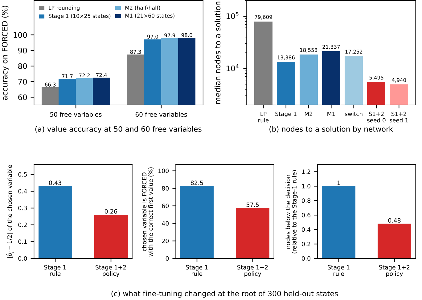
Figure 9: Value accuracy and tree size move independently. (a) Accuracy on FORCED variables of 21 \times 60 in-tree states with 50 and 60 free variables, for relaxation rounding, the Stage-1 network trained on 10 \times 25 states, and the same architecture trained on 21 \times 60 states (M1) or on a half-and-half mix (M2). (b) Median nodes to a solution on the 100-instance set: the networks with the higher value accuracy expand more nodes; the cost-tuned policy expands fewer. (c) At the root of 300 held-out states the fine-tuned policy picks a less confident variable that is less often FORCED-and-correct, and the number of nodes below its decision is half.
