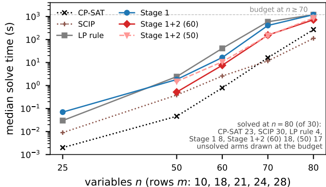
(a) wall-clock time
