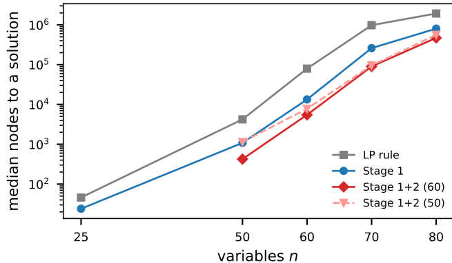
(b) search tree size (lattice off)
