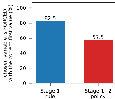
(c) what fine-tuning changed at the root of 300 held-out states
