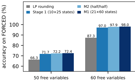
(a) value accuracy at 50 and 60 free variables
