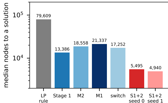
(b) nodes to a solution by network
