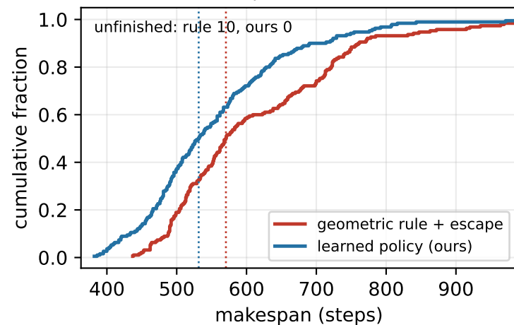
paired difference (learned - rule) median -54, 141 wins / 45 losses, p<0.0001
