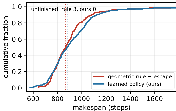
paired difference (learned - rule) median +18, 109 wins / 127 losses, p=0.172
