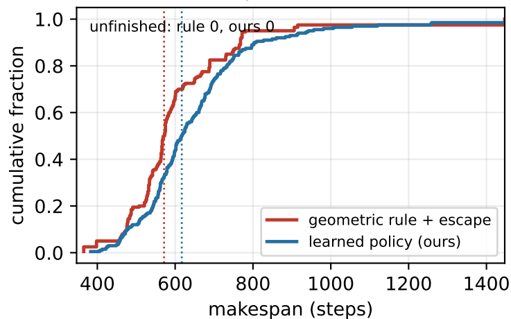
paired difference (learned - rule) median +40, 73 wins / 127 losses, p<0.0001
