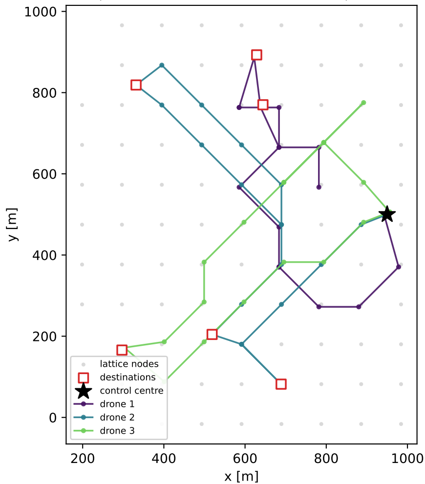
MILP plan, 3 drones, 6 destinations (makespan 180\,s)
