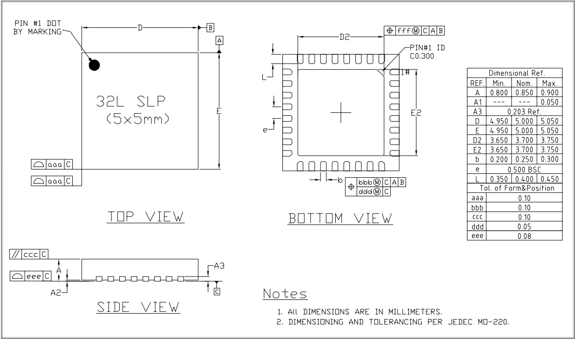
Figure 6-1. ESP8285 Package
