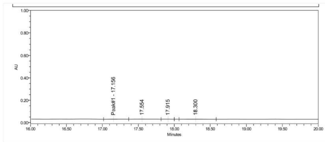
Fig. 1 - HPLC-UV Chromatogram at 214nm
