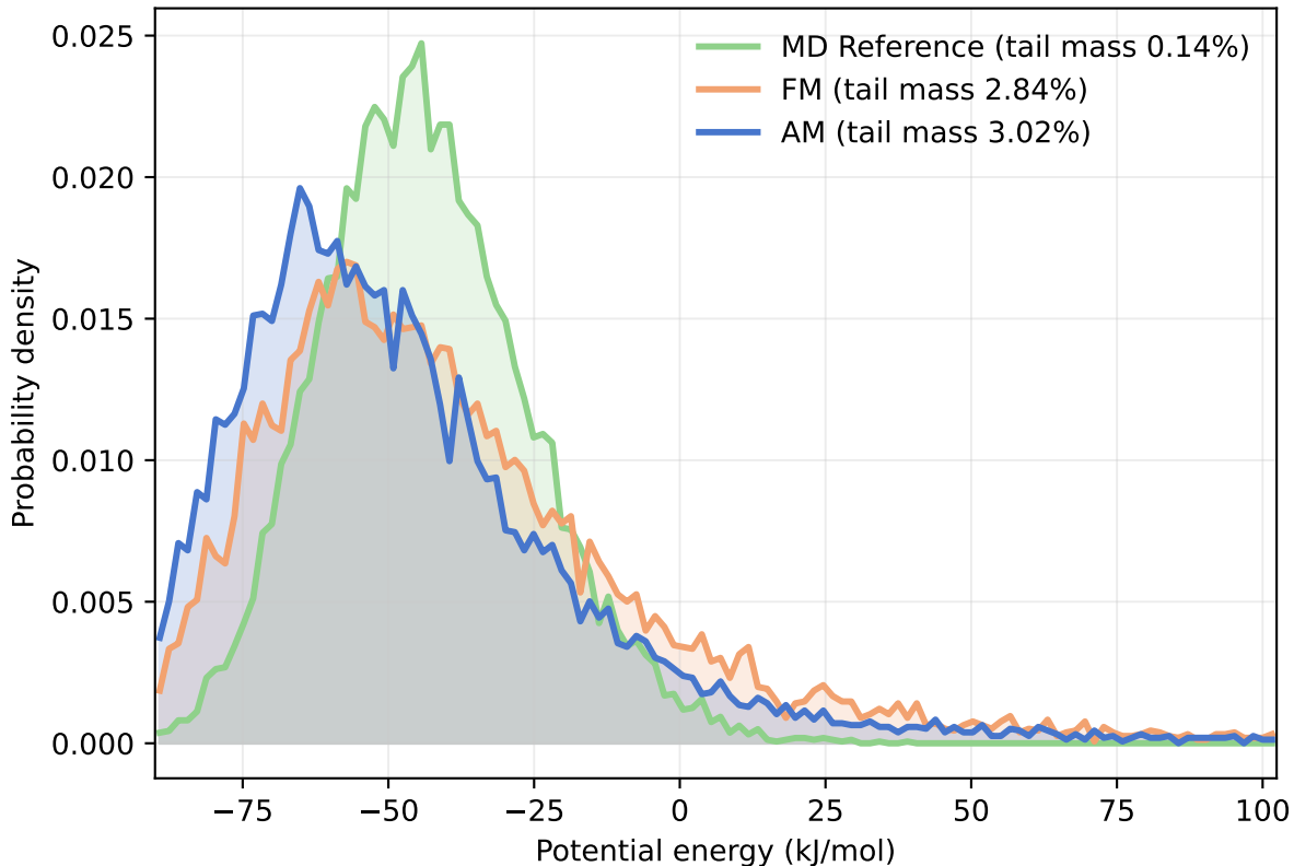
ADTM Ala2 400 K - potential energy
