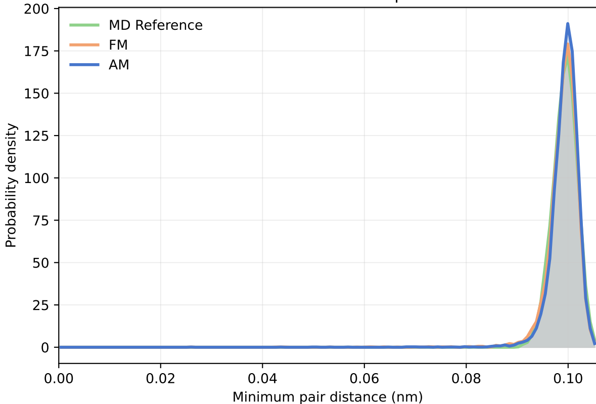
ADTM Ala2 400 K - minimum pair distance
