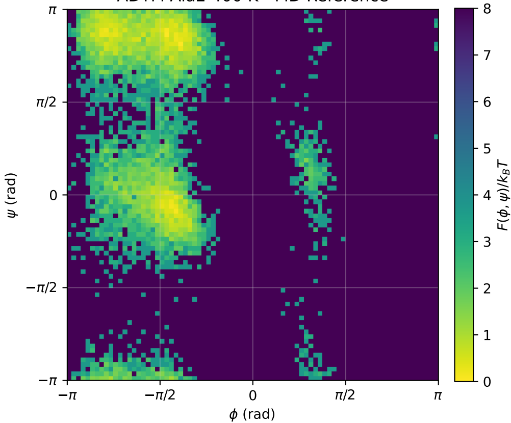
ADTM Ala2 400 K - MD Reference
