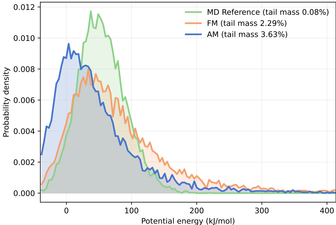
ADTM Ala2 800 K - potential energy
