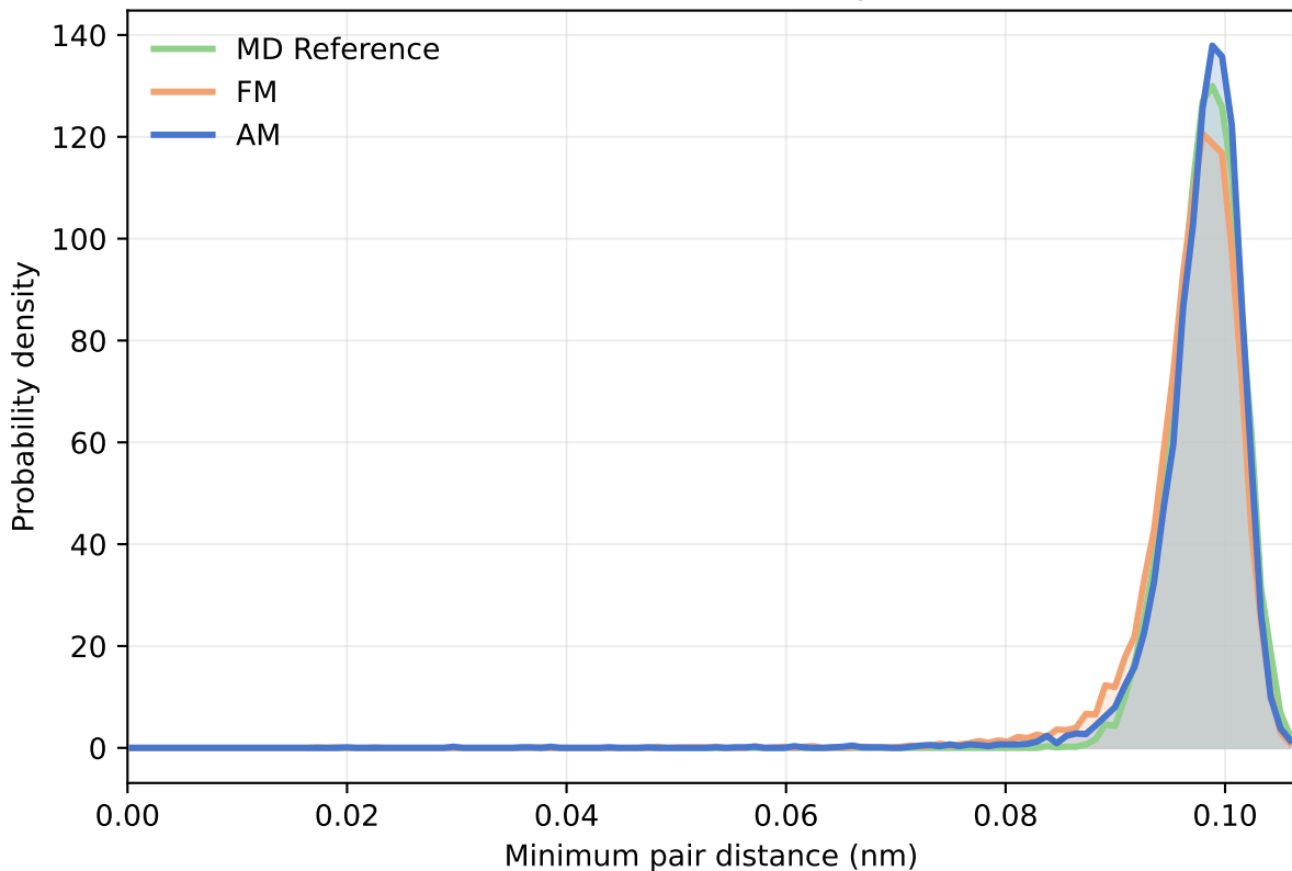
ADTM Ala2 800 K - minimum pair distance
